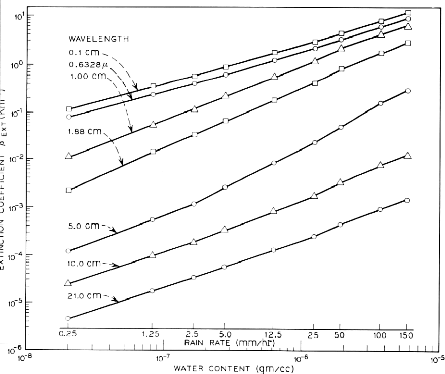
Fig. 2—Rainfall water content and rain rate versus extinction coefficient \beta_{ext} .
