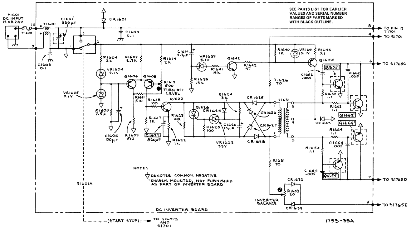
Fig. Option 7-5. 464 Option 7 dc inverter.
