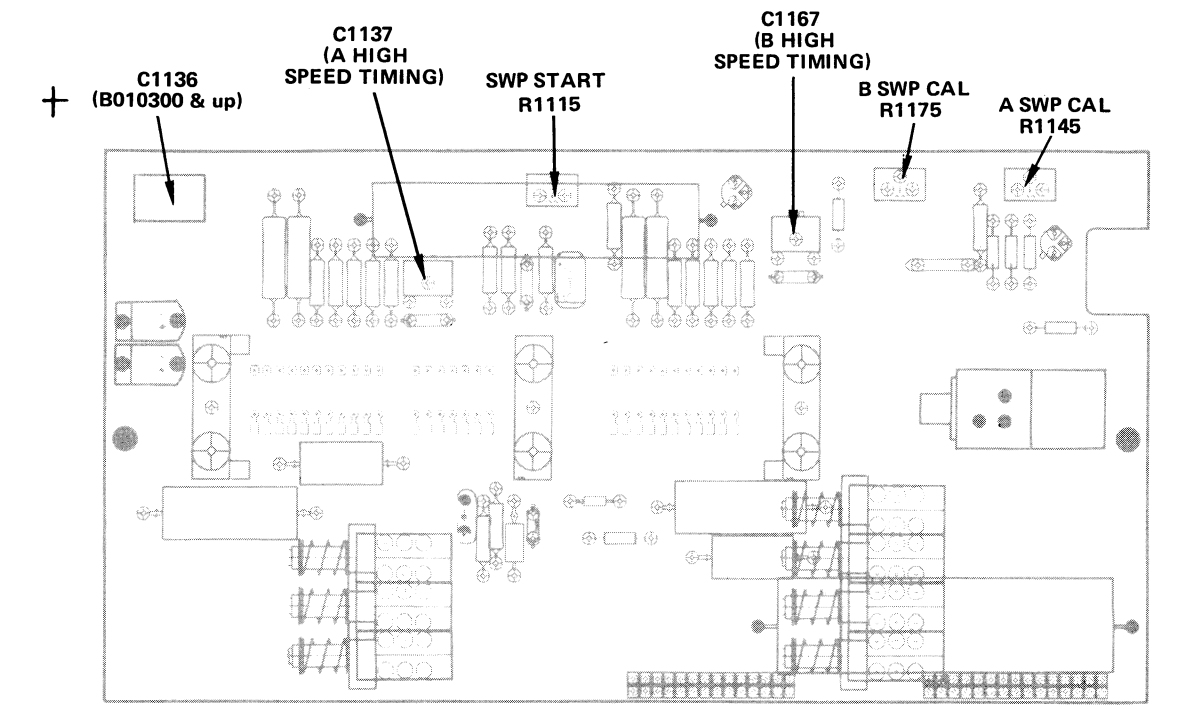
(C) Timing circuit board adjustment locations.
