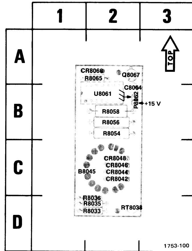
(A) A11 Fan Motor board (SN B138090 & up).
