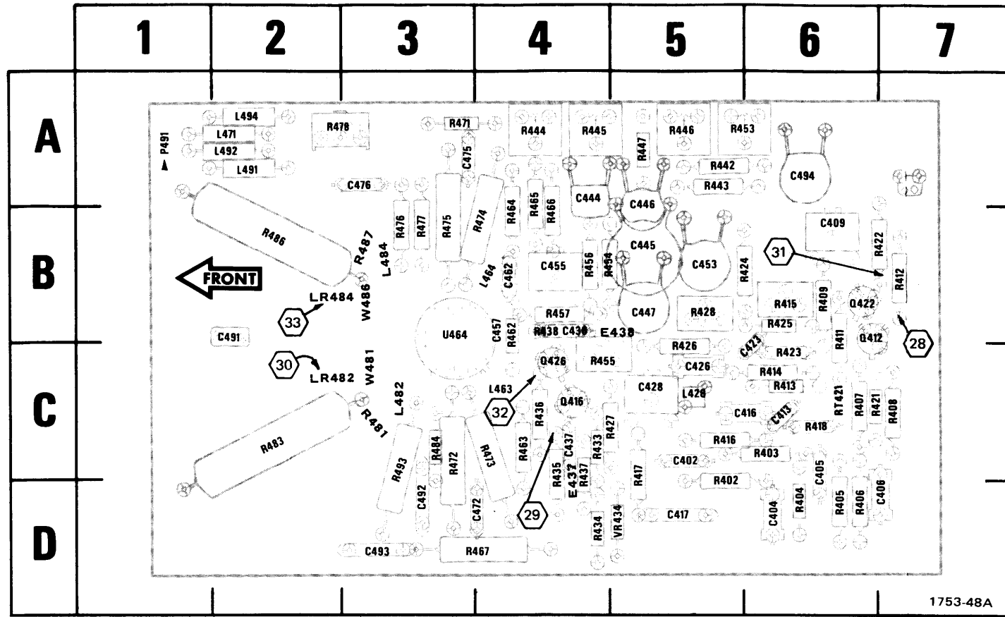
(A) A4 Vertical Output circuit board (SN B150755-up).
