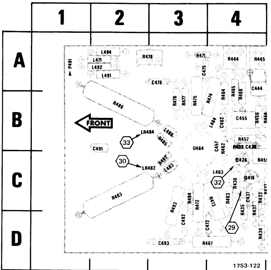
(C) Partial A4 Vertical Output circuit board (SN B150754 & below).
