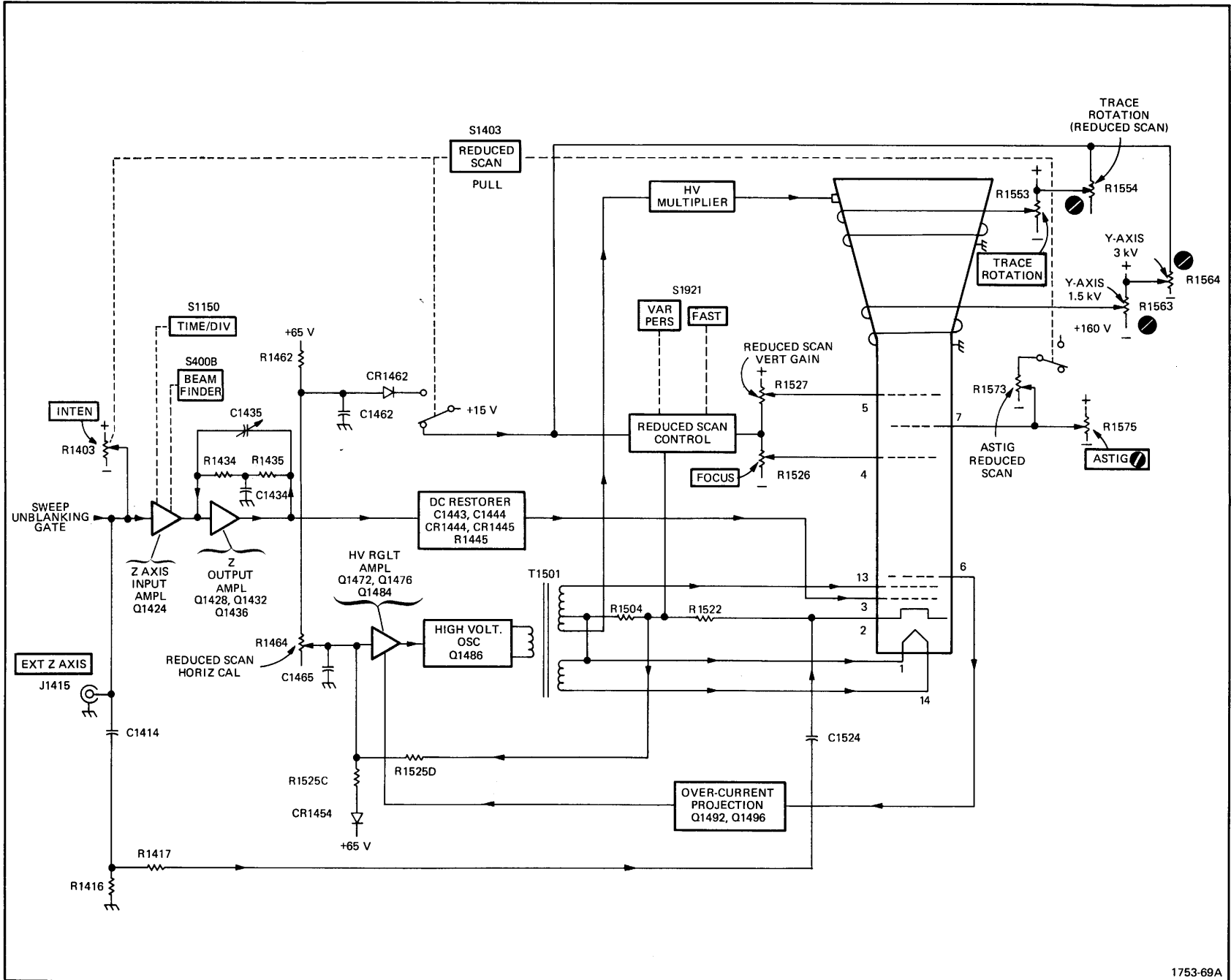
Fig. 3-7. Z-Axis/CRT Circuit Detailed Block Diagram.
