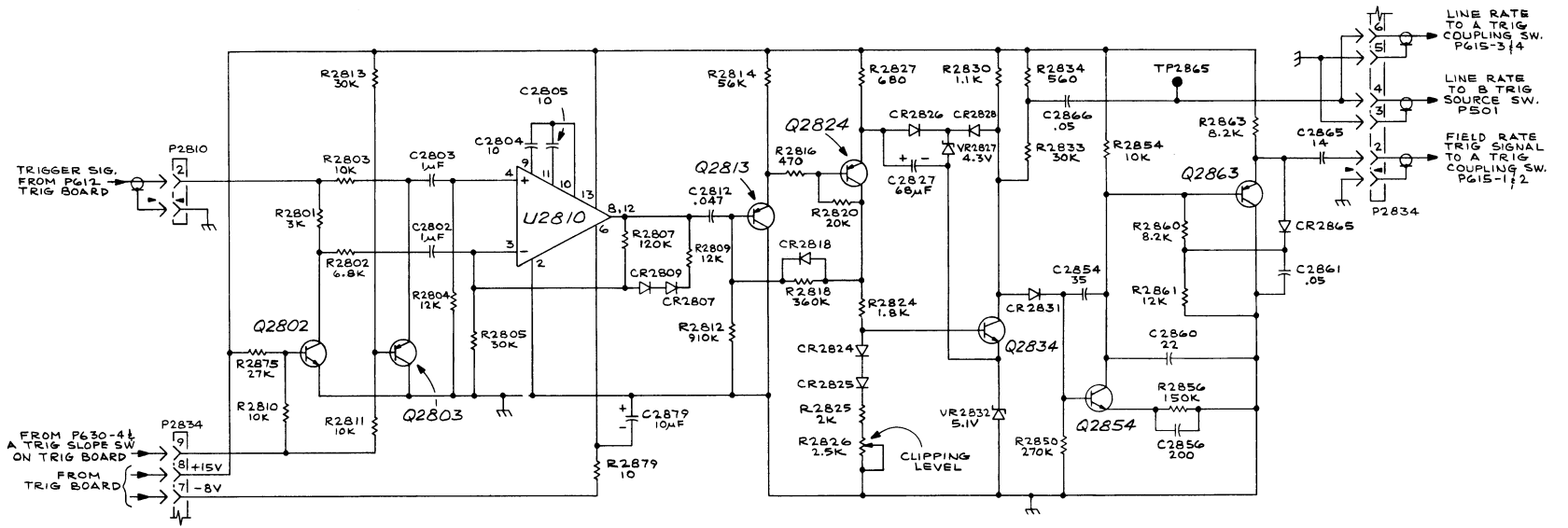
Fig. Option 5-6. Option 5 TV Sync Separator & Inverter Ampl.
