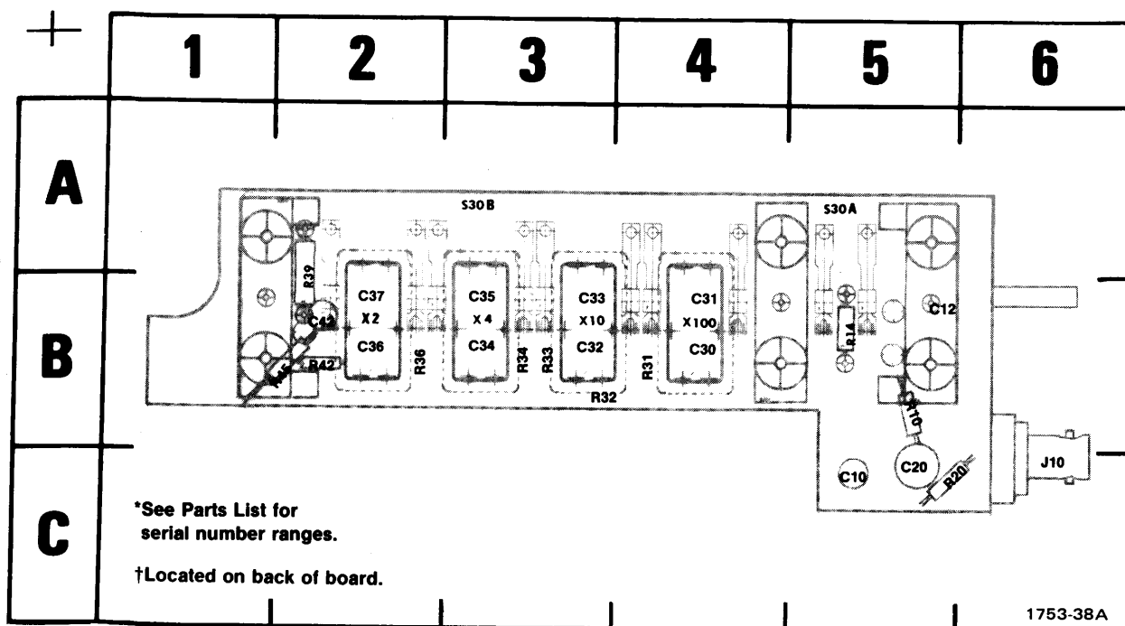
(A) A1 Attenuator circuit board.
