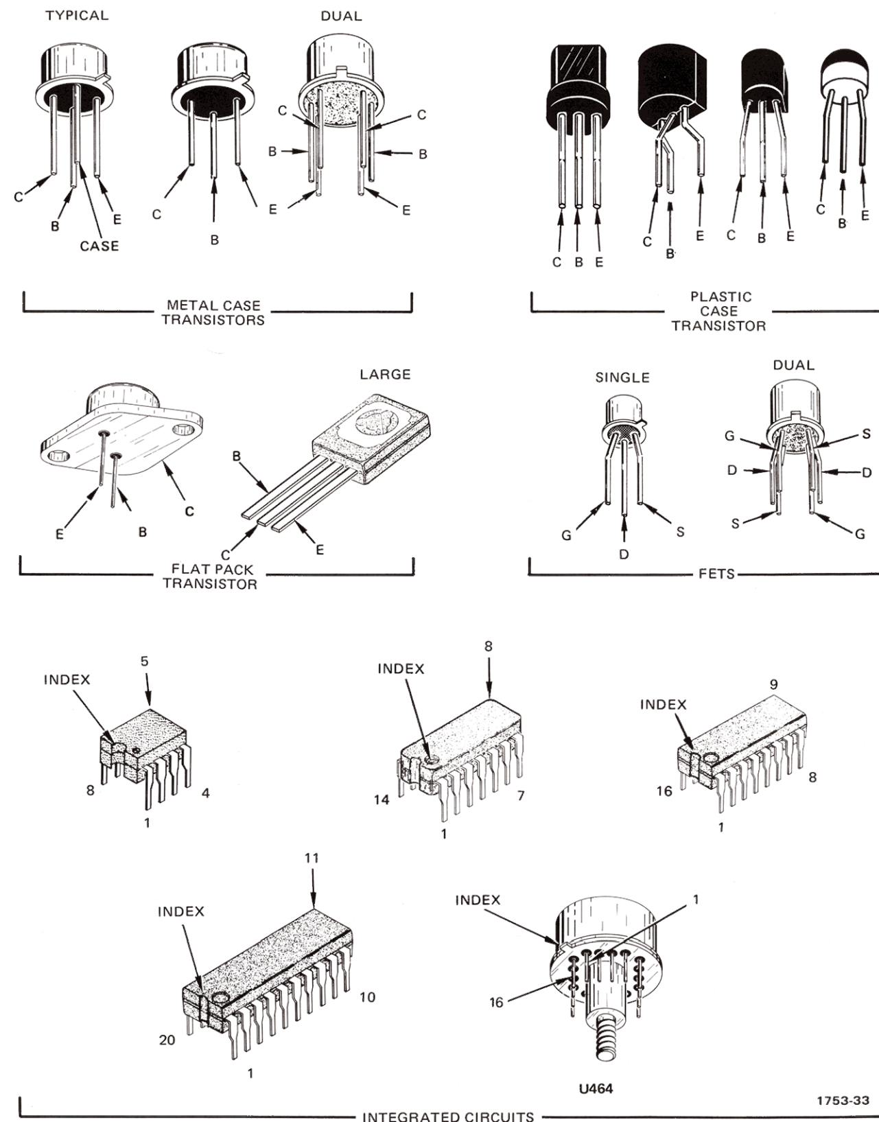
Fig. 7-1. Semiconductor Lead configurations.
