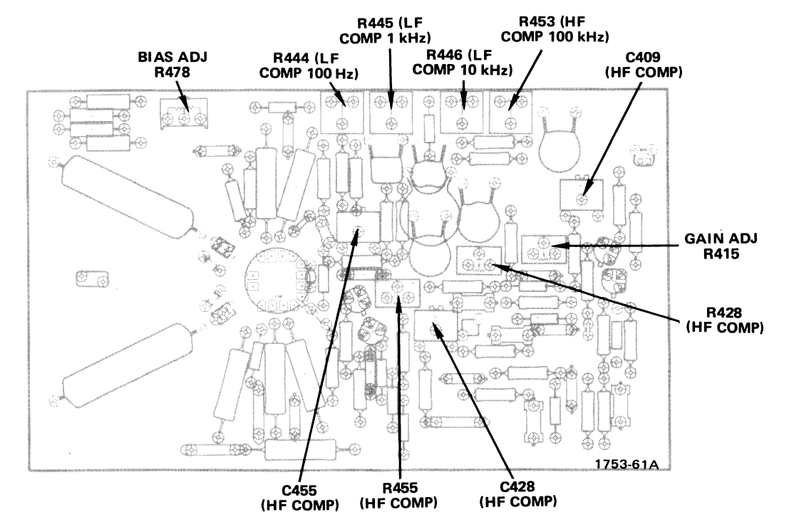
(B) Vertical Output circuit board adjustment locations.
