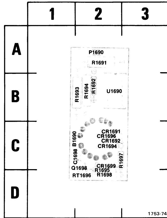
(C) A11 Fan Motor board (SN below B138090).
