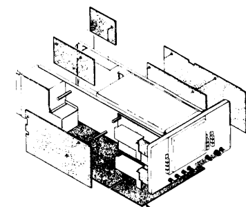
1753-56 STORAGE A10 (B) Board location.
