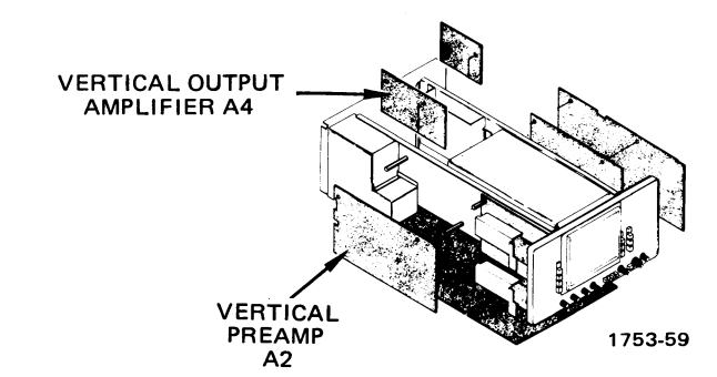
(A) Board locations
