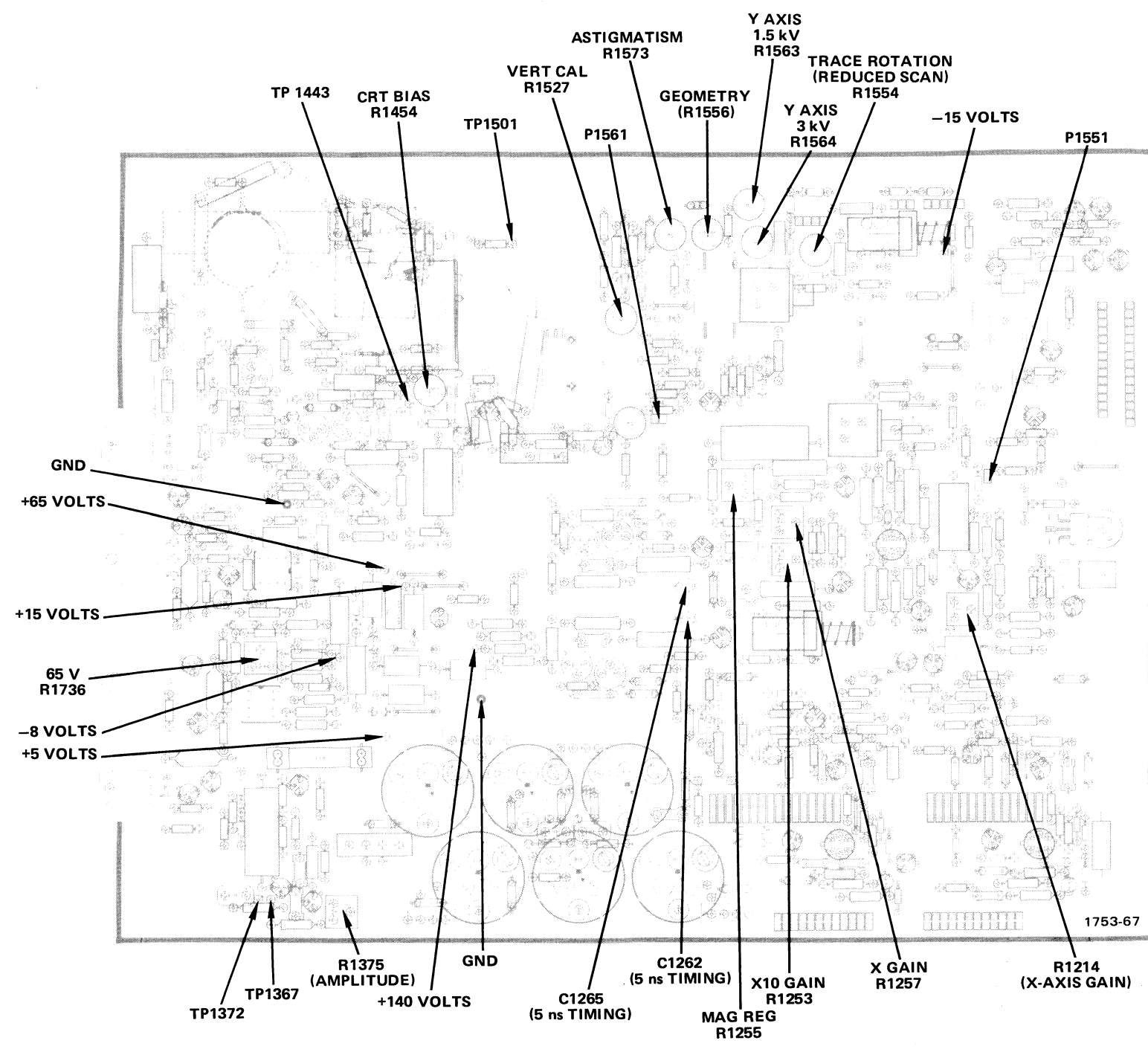
(B) Main Interface circuit board adjustment locations.
