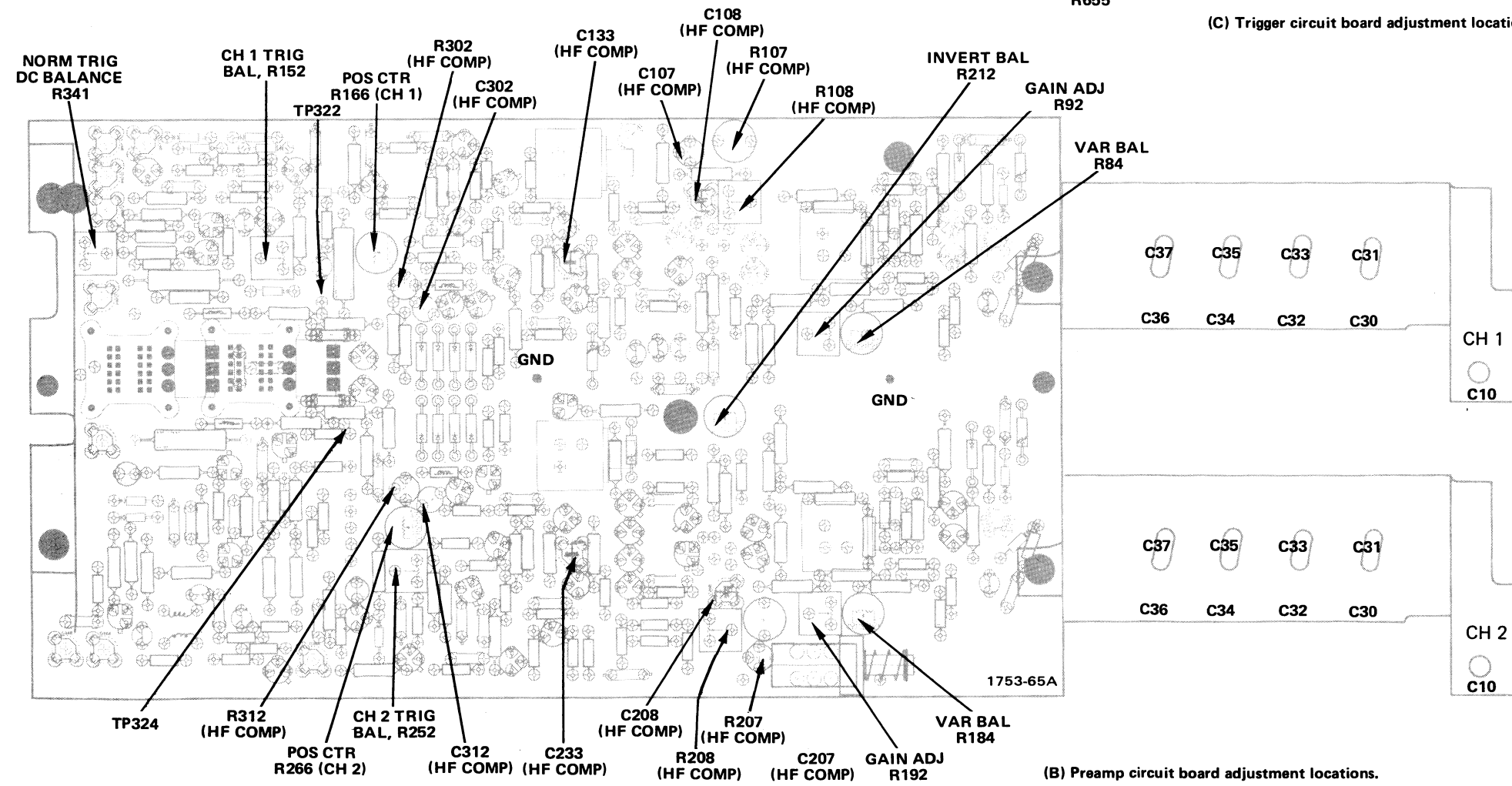
(B) Preamp circuit board adjustment locations.
