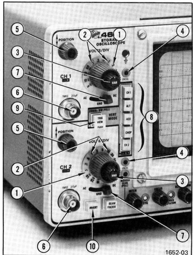
Fig. 2-2. Vertical Section.
