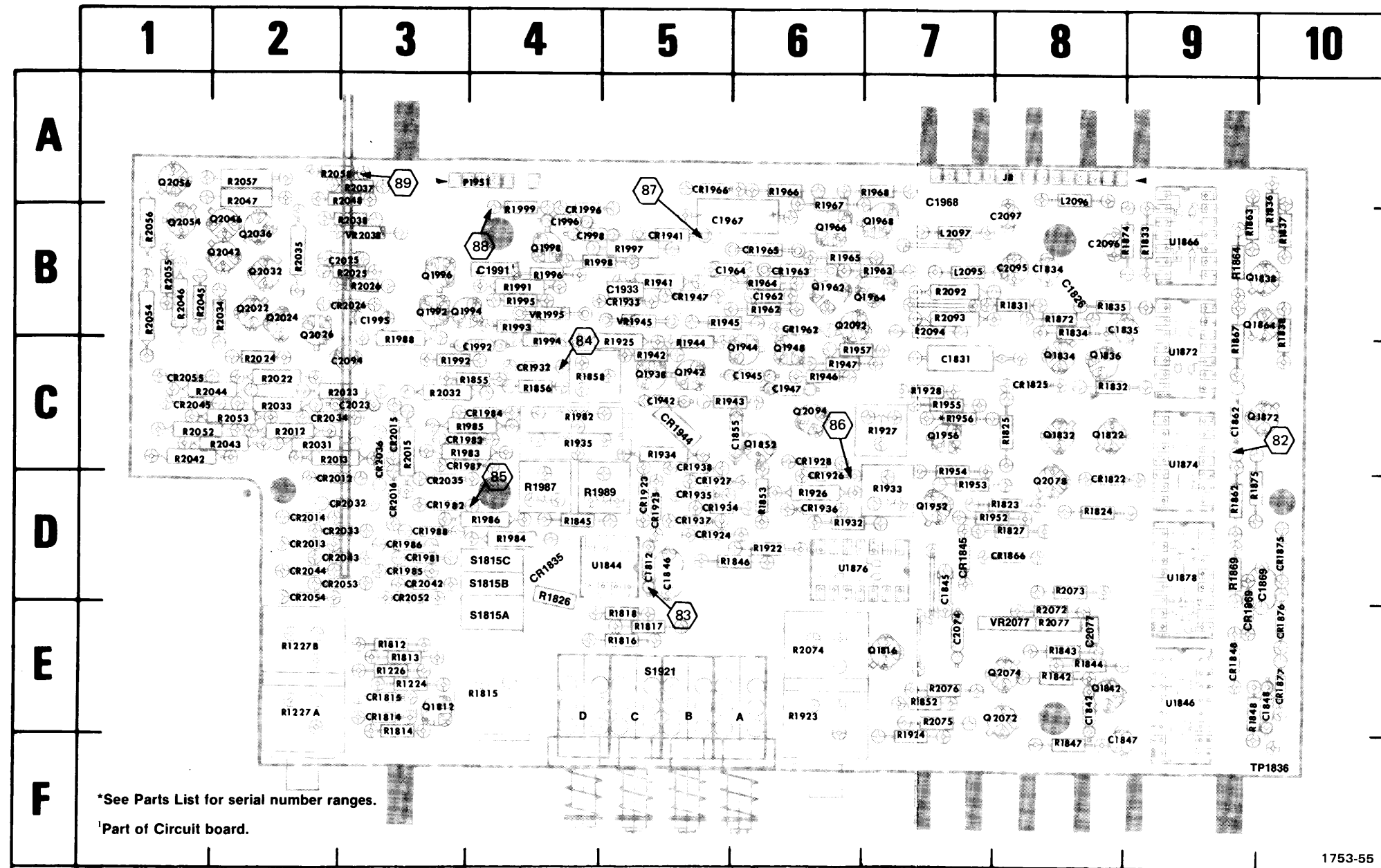
(A) A10 Storage board.
