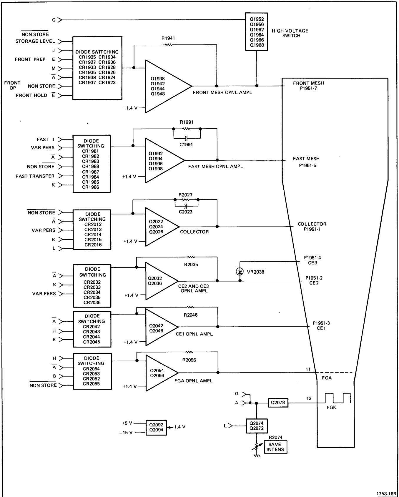
Fig. 3-10. Storage Output Circuits Block Diagram.
