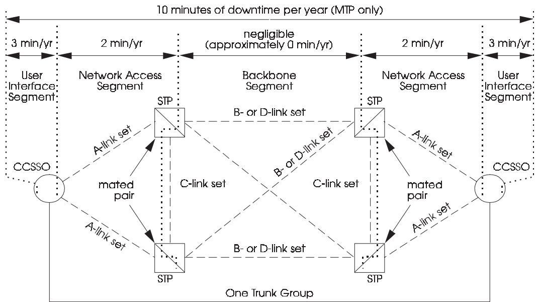
Figure 4-26. Example Case: One Trunk Group with Its Terminating CCSOs)
