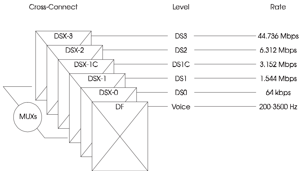
Figure 9-5. Interconnection Hierarchy
