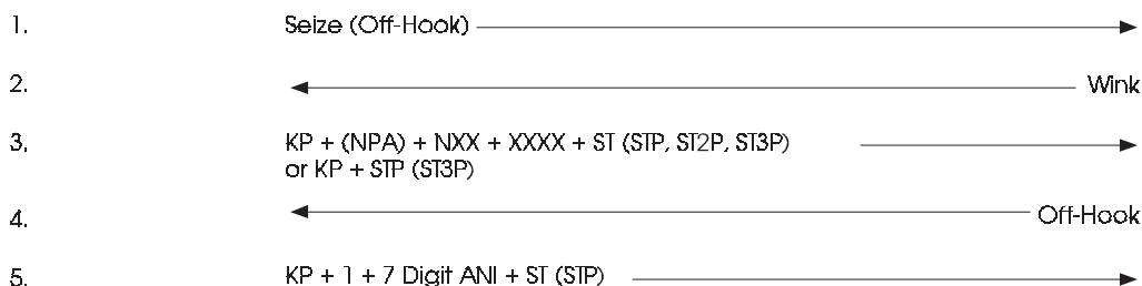
Figure 6-58. Originating Signaling Sequence
