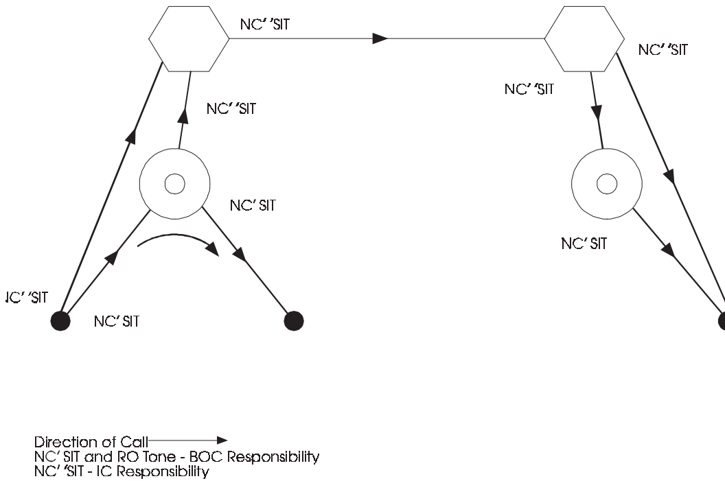
Figure 6-62. No-Circuit Condition
