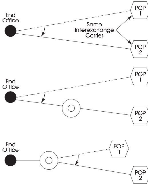
Figure 4-13. Alternate Routing
