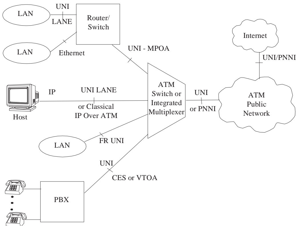
Figure 14-37. Campus/Enterprise Environment
