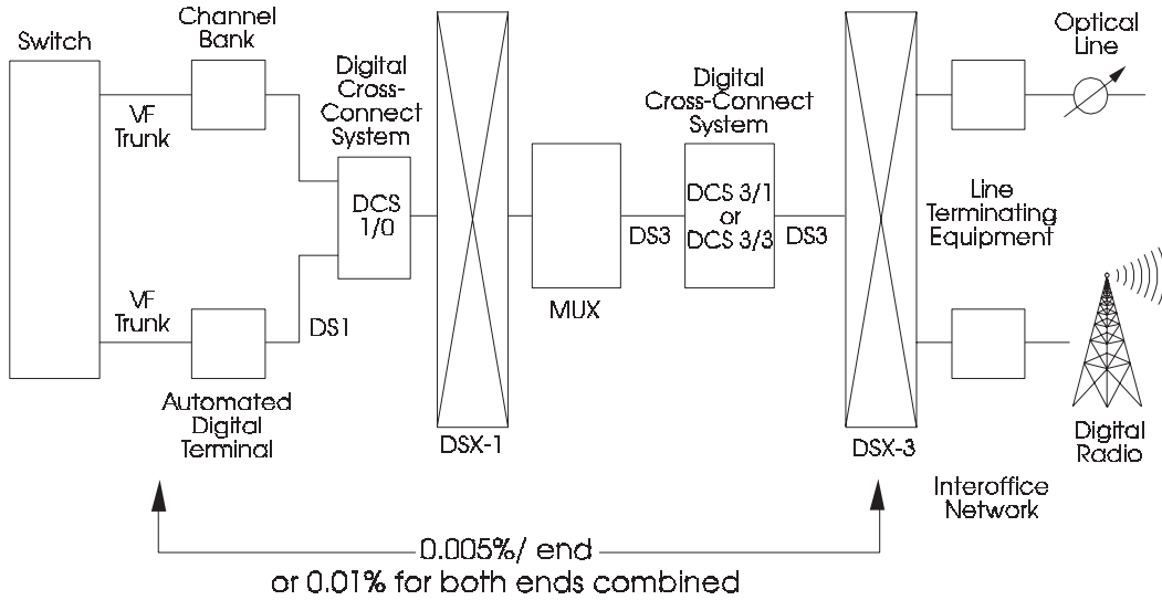
Figure 4-23. Facility-Entrance Network Segment Availability
