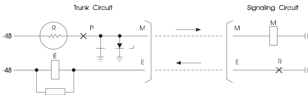
Figure 6-17. Type I Interface
