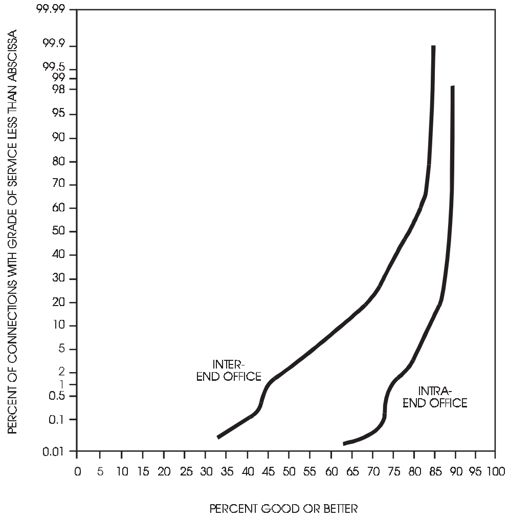
Figure 7-13. Grade-of-Service Distributions
