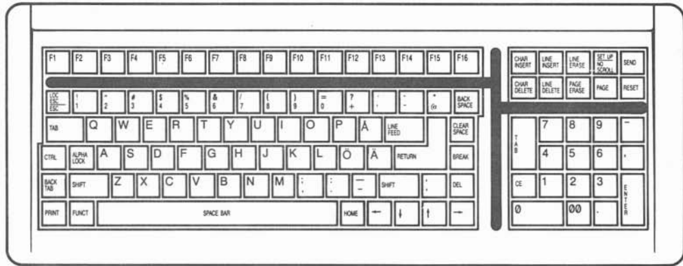
Figure F-7 Finnish Keyboard Layout
