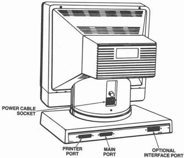
Figure 1-4 955 Terminal, Rear View
