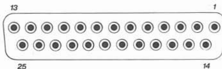
Figure 1-5 Pin Numbers (25-Pin RS-232 Connector)
