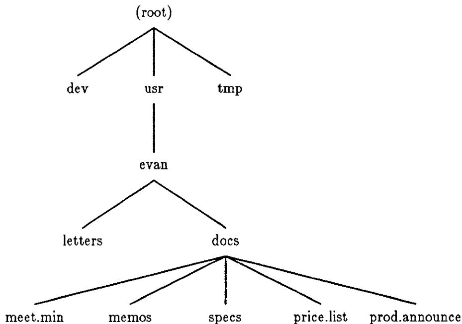
Figure 1-2: Sample File Hierarchy
