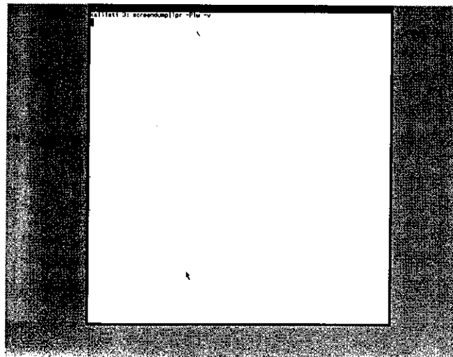
Figure 3-1: Sample Window
