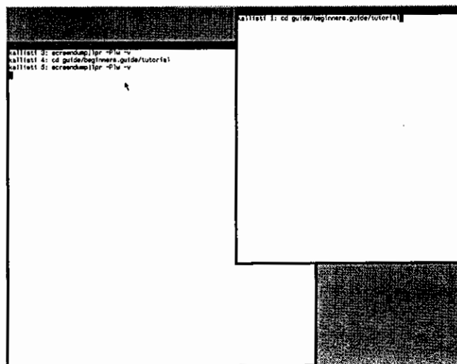
Figure 3-3: Copying Text
