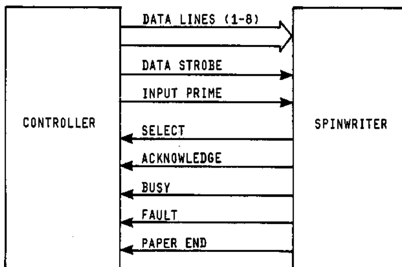
Centronics-Type Interface Lines
