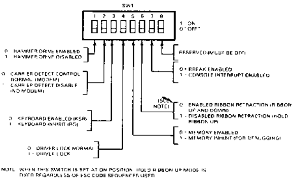
5500 G9DWC PCB (5540) SW1 Switch Functions
