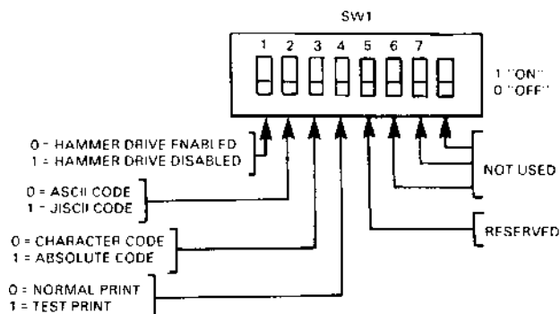
5500 G9CUR PCB SW1 Switch Functions (Early 5510, 5520 Models)
