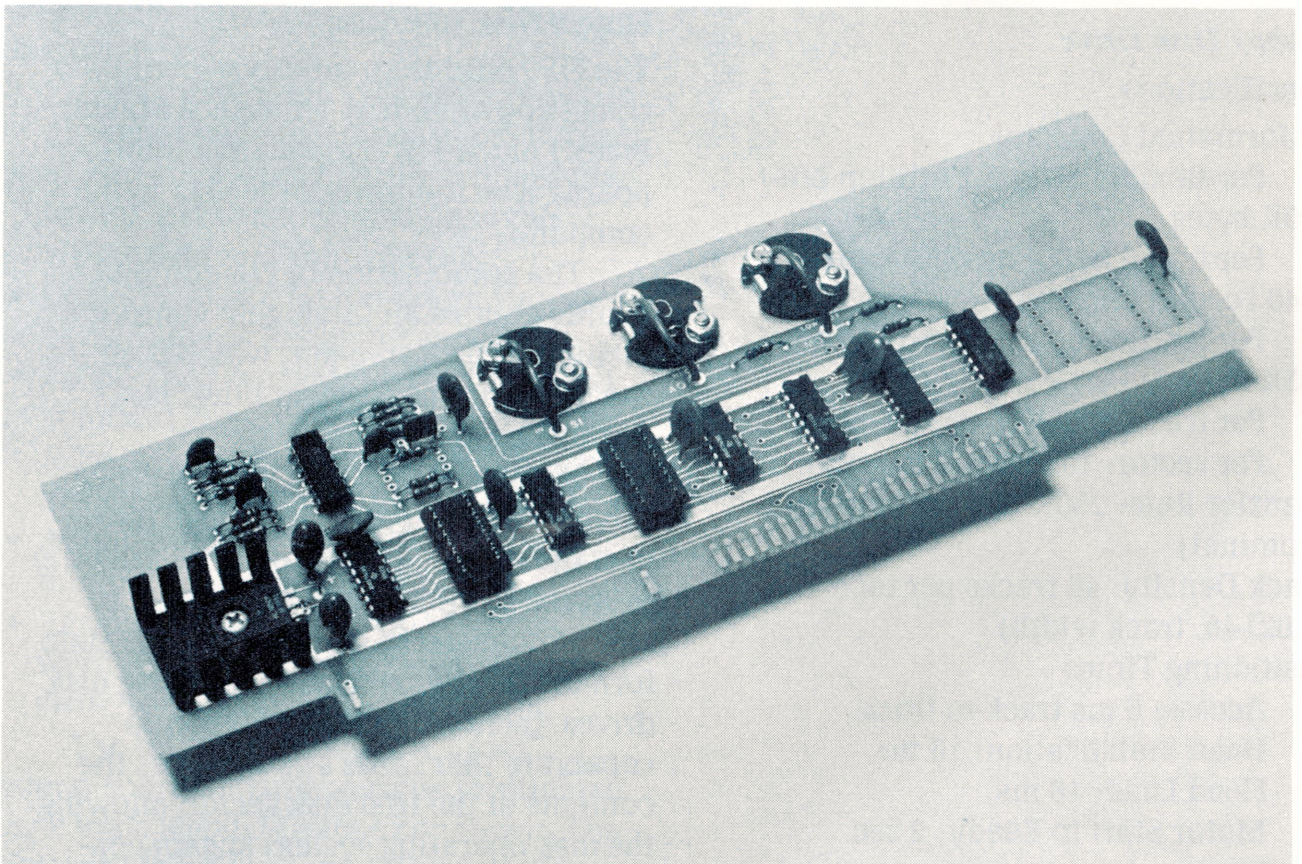
Universal Tape Cassette Recorder Interface UCRI-1
