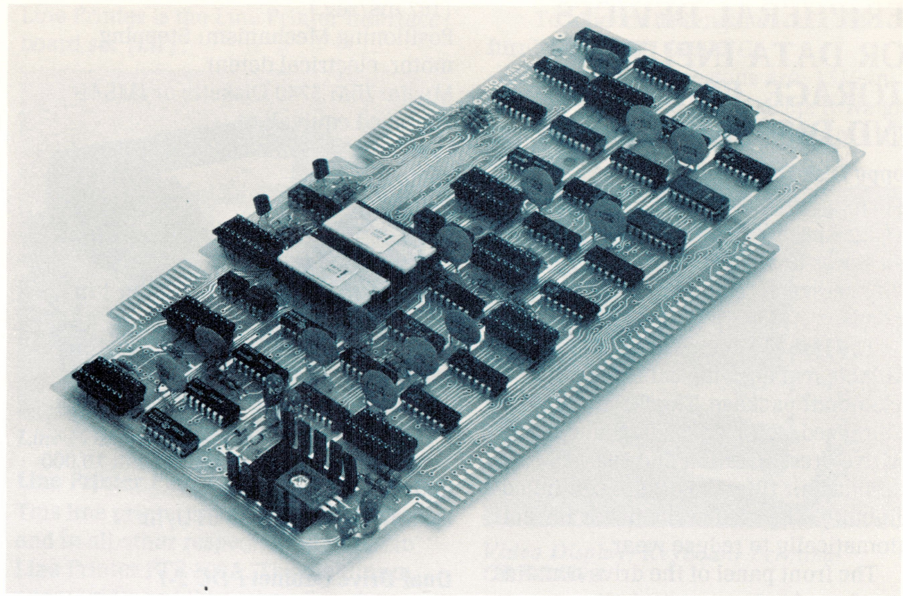
Serial I/O Interface SIO 2-2
