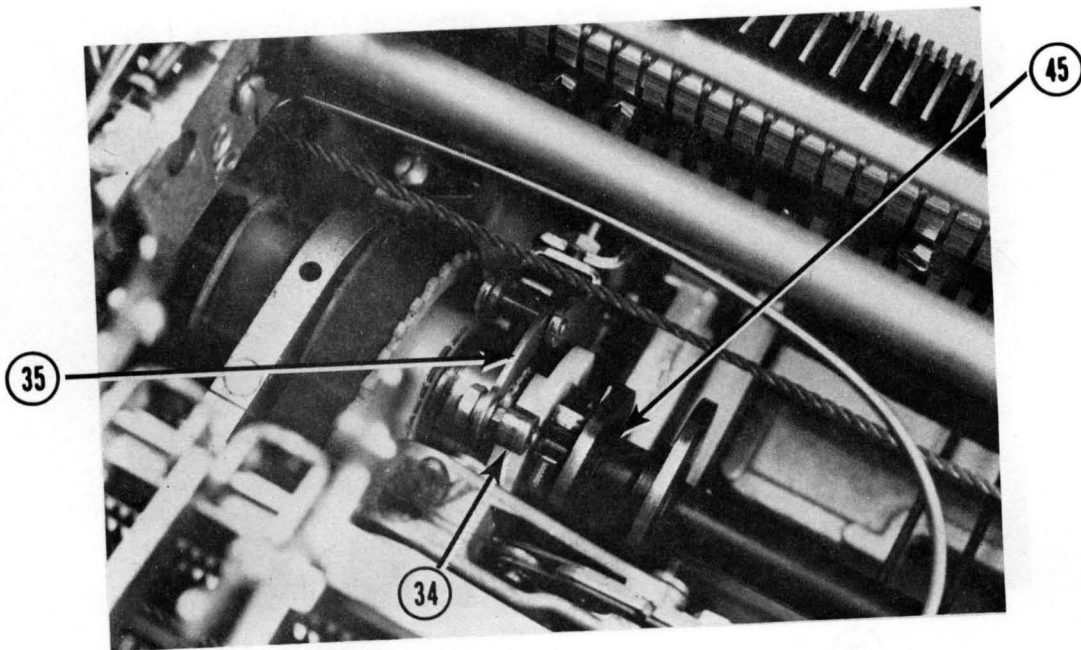
Figure 50. Cycle clutch
