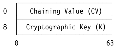
Figure 7-54. Parameter Block for KMAC-DEA
