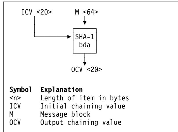
Figure 7-38. Symbol for SHA-1 Block Digest Algorithm
