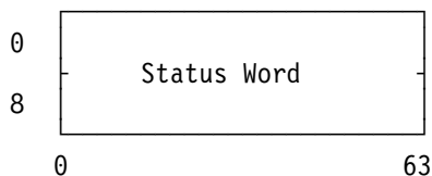
Figure 7-53. Parameter Block for KMAC-Query
