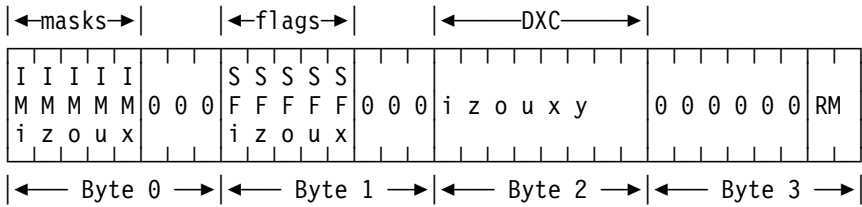
Figure 19-1. FPC Register Overview
