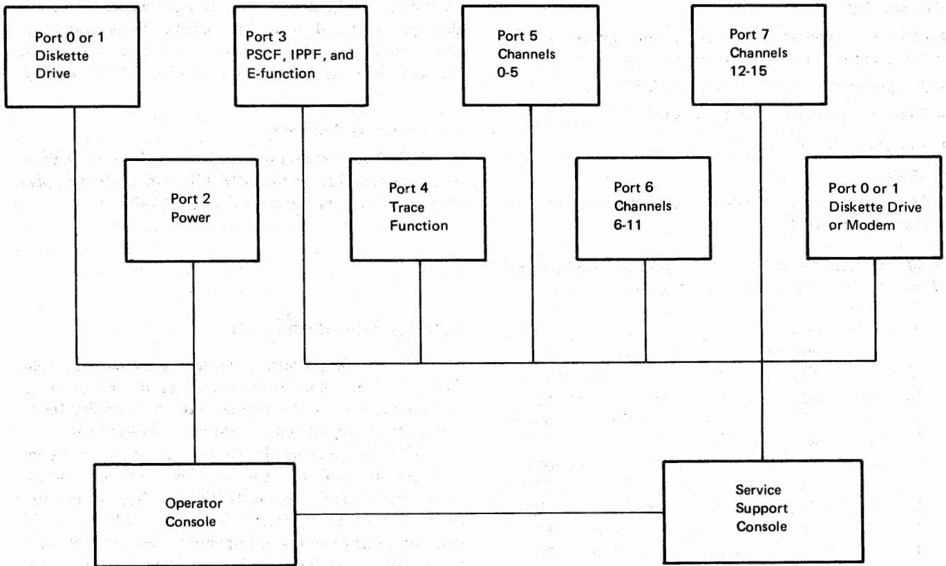
Figure 4-6. Normal Configuration
