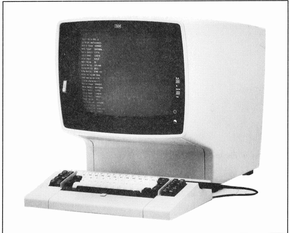
Figure 5-3278-1. 3278 Display Station
