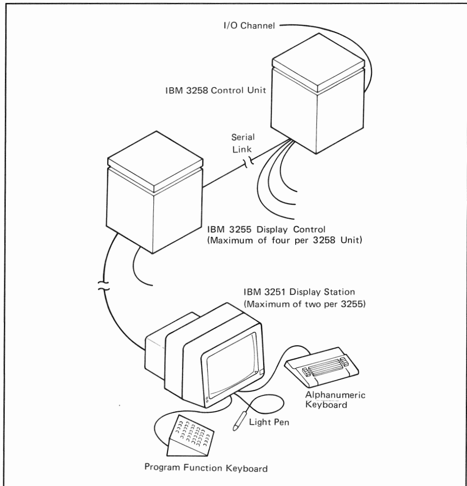
Figure 11-3250-2. 3250 System Simplified Configuration
