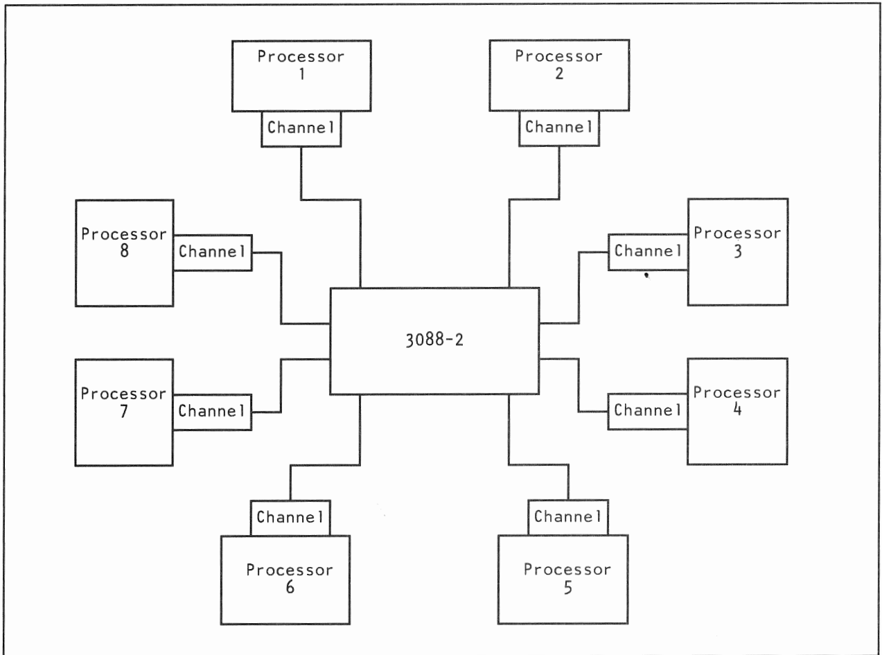
Figure 1-3088-3. 3088 Model 2 Configuration
