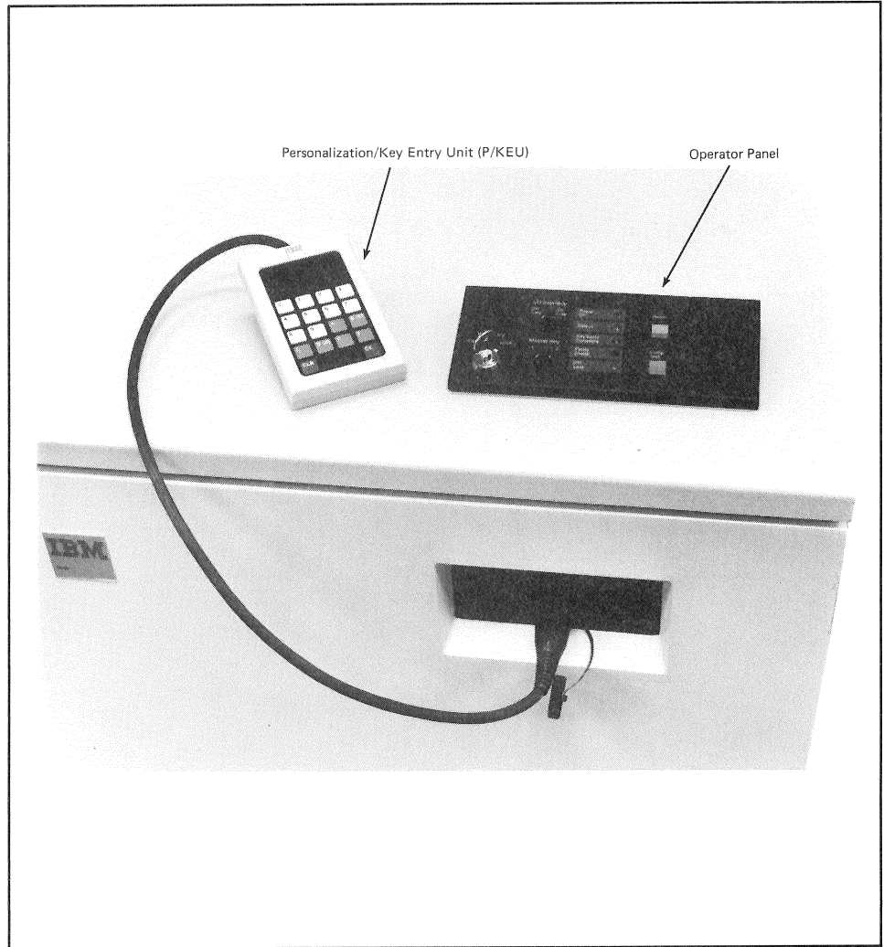
Figure 1-3848-2. 3848 Personalization/Key Entry Unit and Operator Panel
