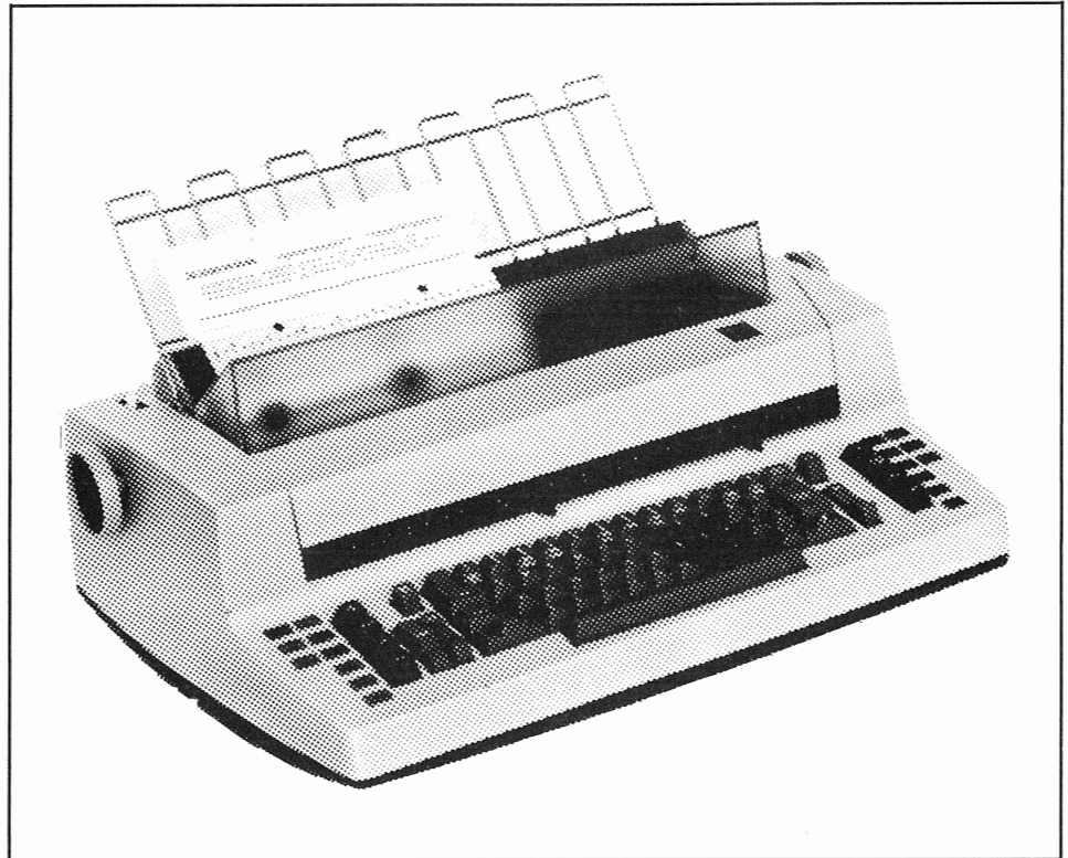
Figure 11-3790-5. 3793 Keyboard-Printer
