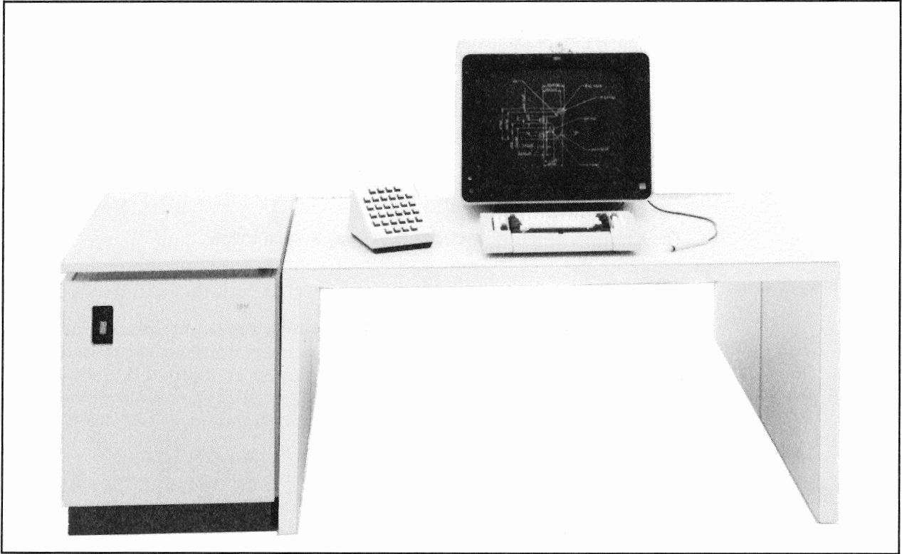
Figure 11-3250-1. 3250 Graphics Display System
