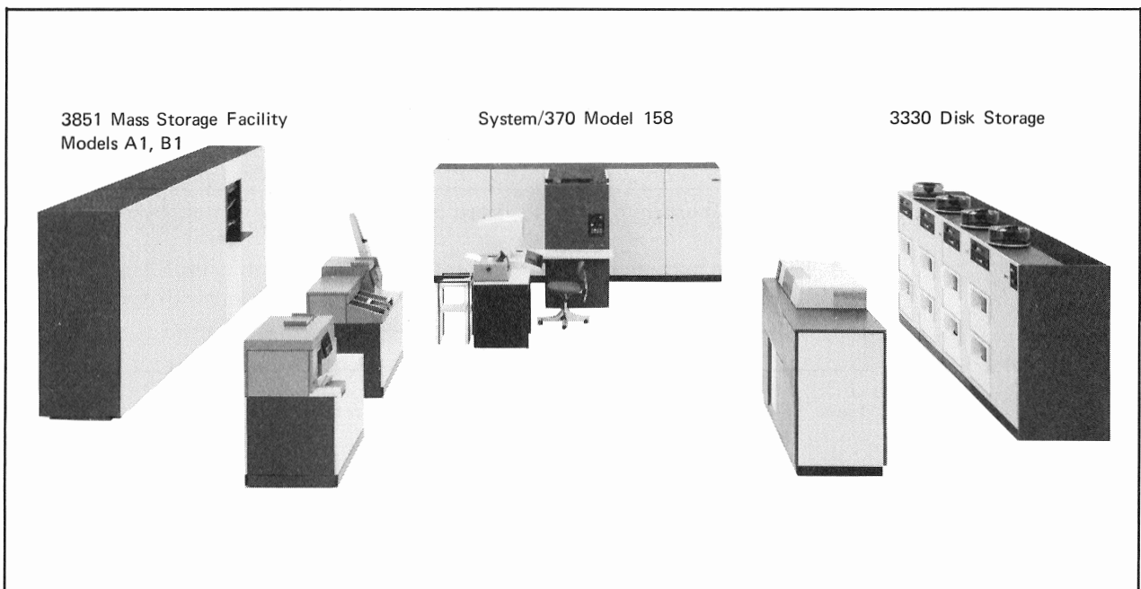
Figure 11-3850-1. 3850 Mass Storage System with 3851 Mass Storage Facility, System/370 Model 158, and 3330 Disk Storage
