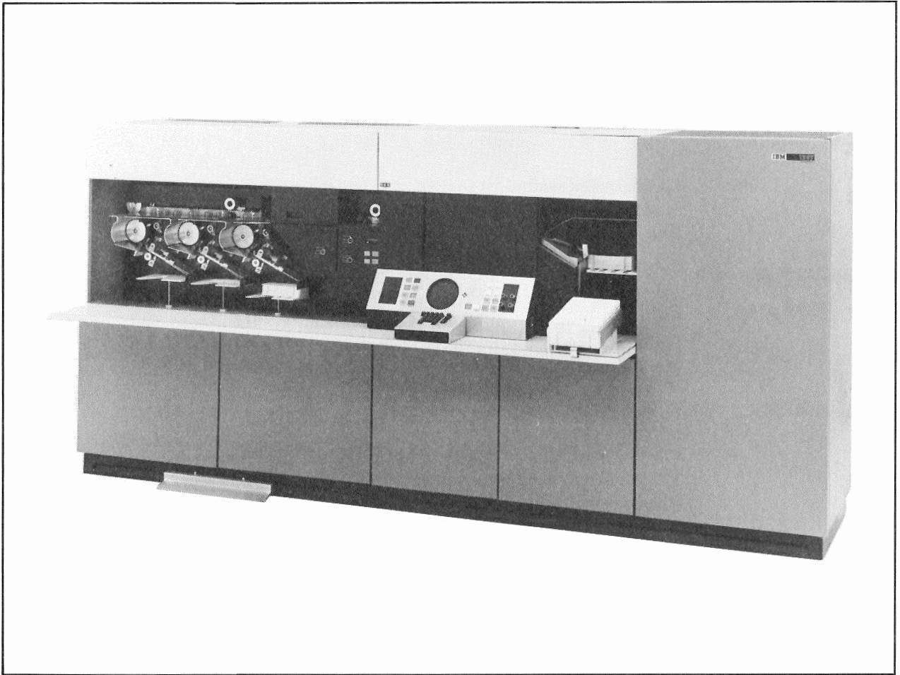
Figure 7-1287-2. 1287 Optical Reader Model 5
