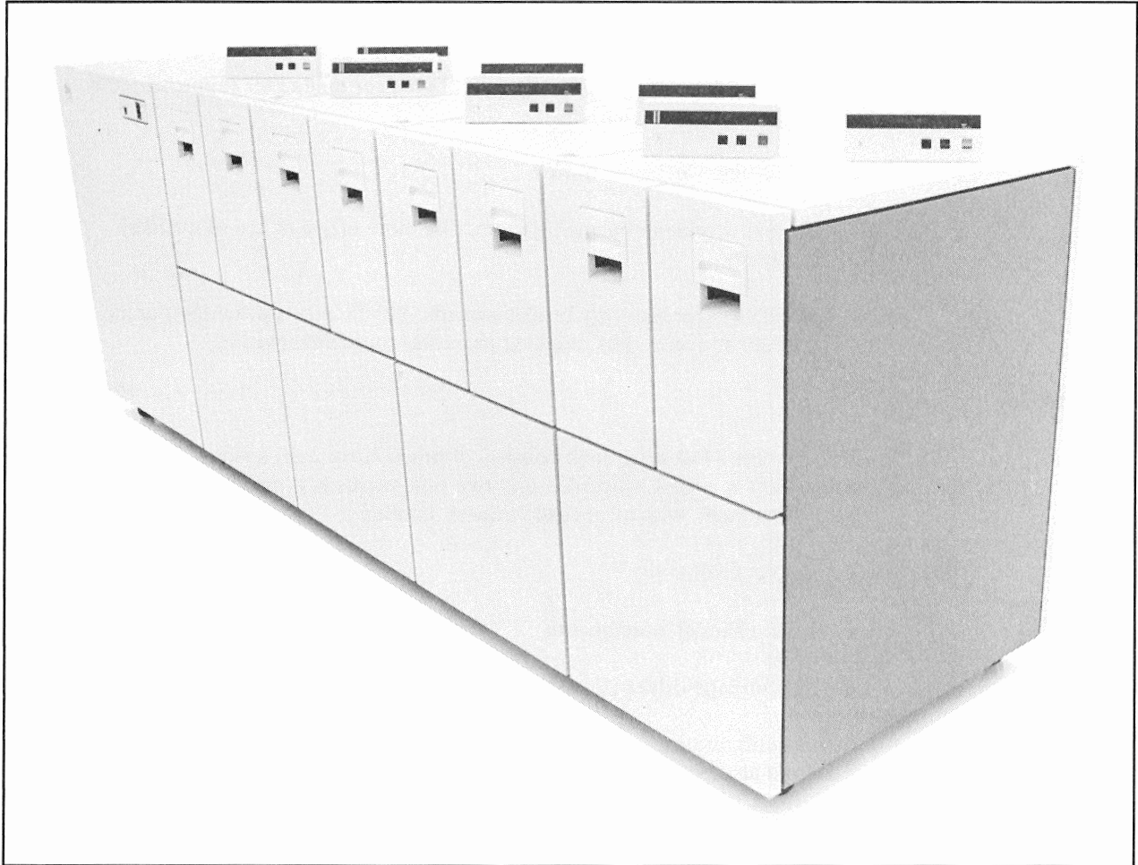
Figure 4-3480-1. 3480 Magnetic Tape Subsystem
