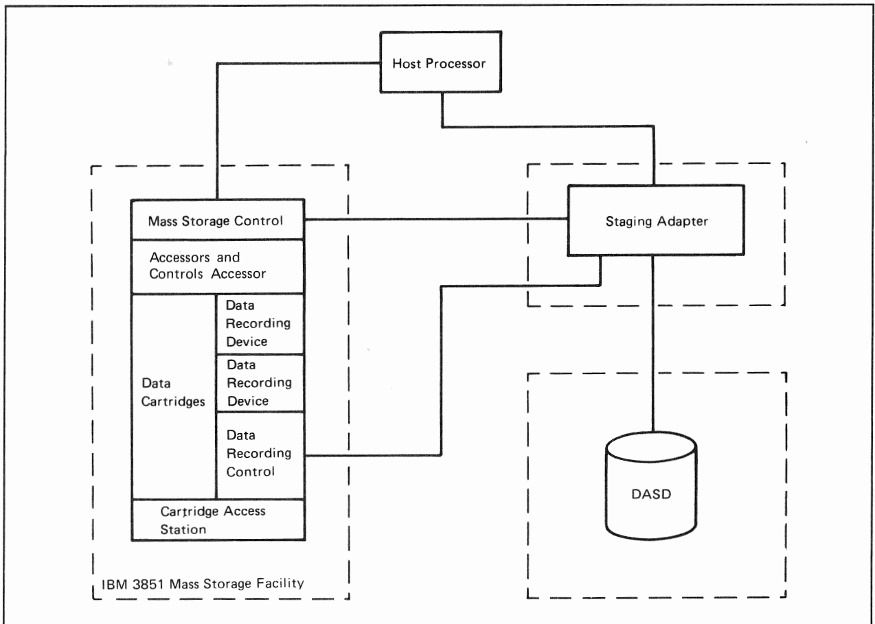
Figure 11-3850-3. 3850 Mass Storage System Logical Units
