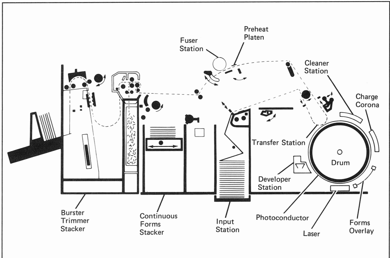
Figure 8-3800-2. 3800 Printing Subsystem Functional Units
