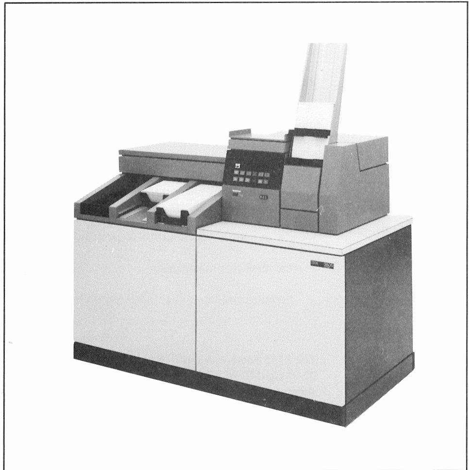
Figure 9-3505-1. 3505 Card Reader
