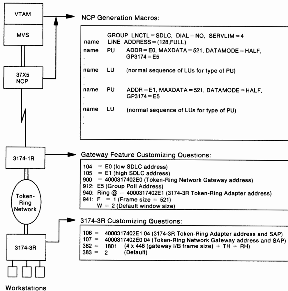
Figure 4-2. Configuration Example for 3174 Model 1R with the IBM Token-Ring Network 3270 Gateway feature
