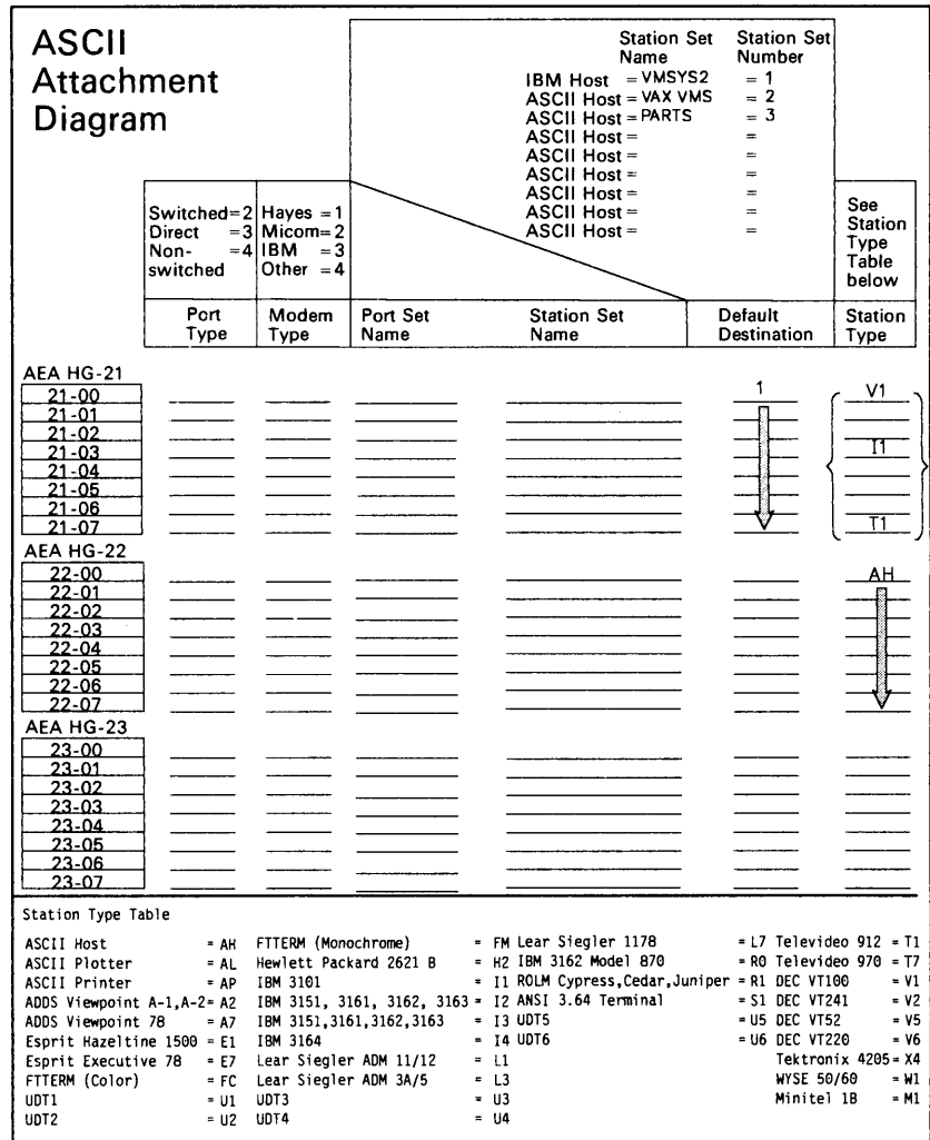
Figure 12-11. Filling In the Default Destination Column on the ASCII Attachment Diagram
