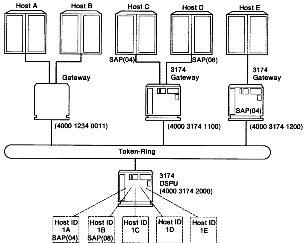
Figure E-5. Combination of Gateway Capabilities
