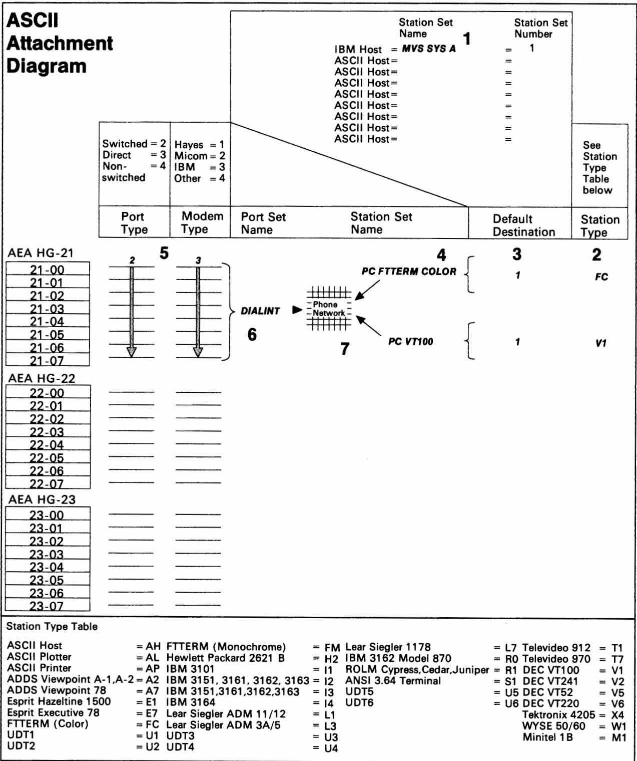
Figure B-8. 3270 Terminal Emulation—ASCII Attachment Diagram
