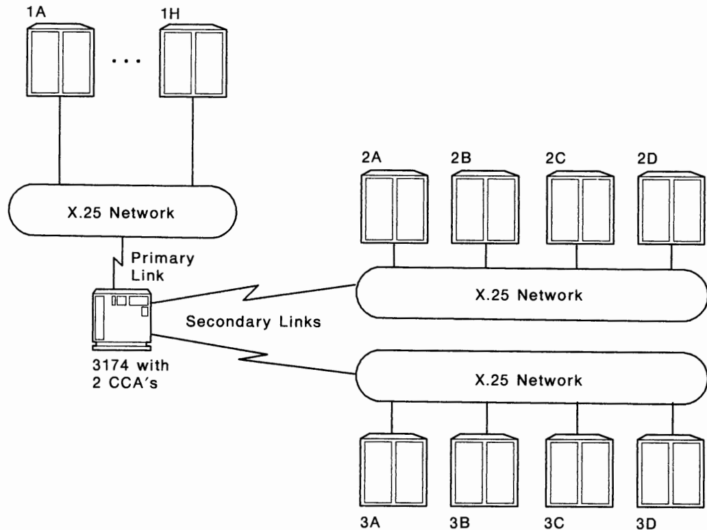
Figure 2-4. X.25 Single Link Multi-Host Support
