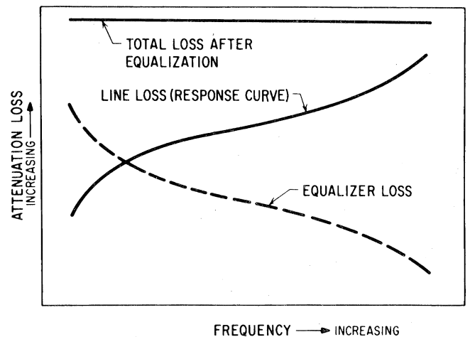
Figure 24. Frequency distortion
