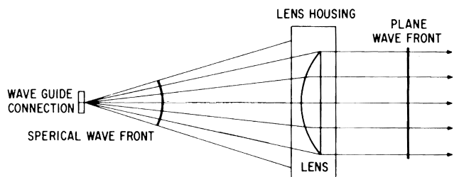
Figure A3.5 Delay lens horn antenna
