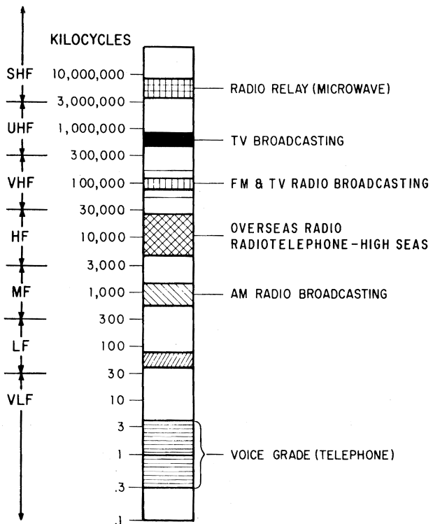
Figure 33. Frequency spectrum
