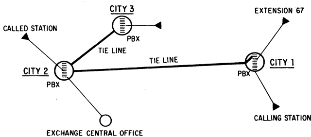
Figure 43. Tie line operation
