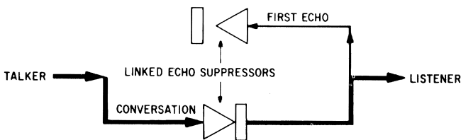
Figure 38. Principle of echo suppression
