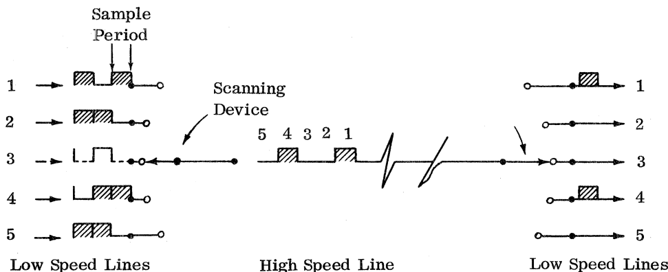
Figure 23. Time multiplexing
