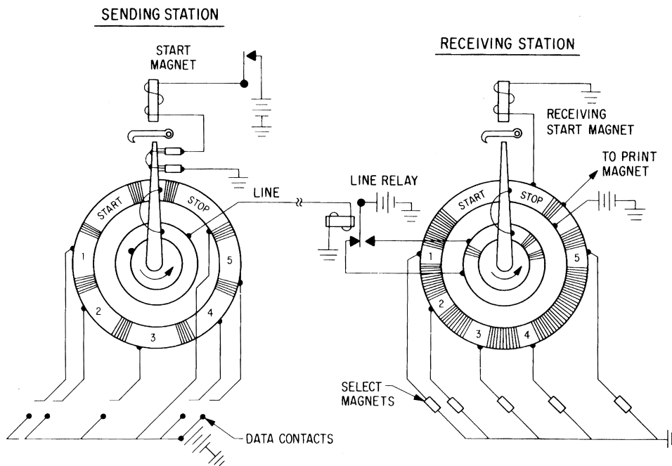
Figure A2.4 Theory of start-stop teletypewriter system
