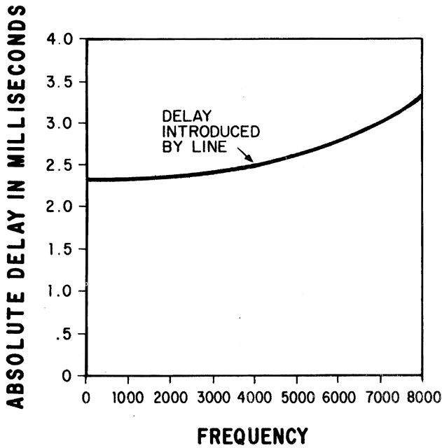
Figure 25. Delay distortion
