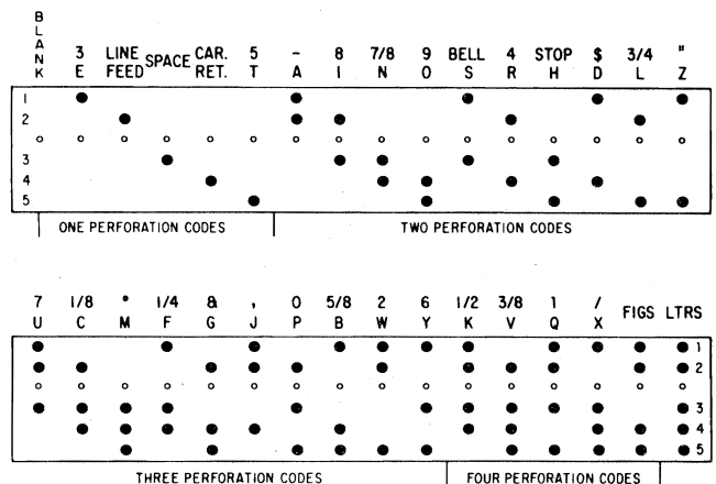
Figure 5. Baudot code
