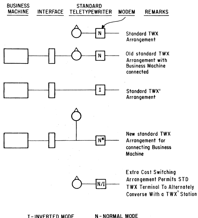
Figure 41. TWX & TWX' station arrangements
