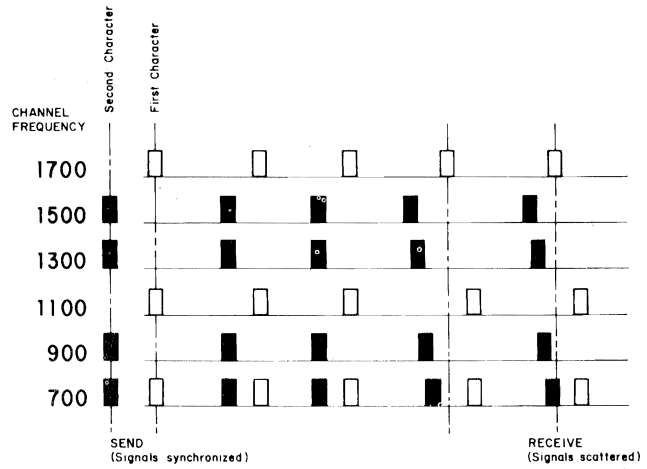
Figure 26. Effect of delay distortion
