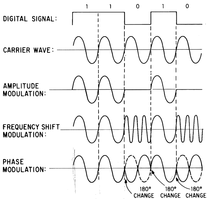
Figure 20. Modulation techniques
