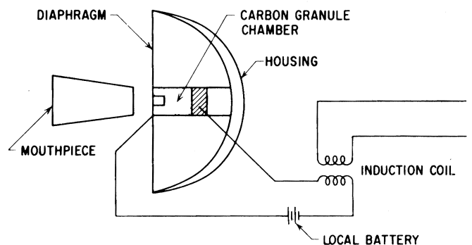
Figure A1.3 Basic telephone transmitter
