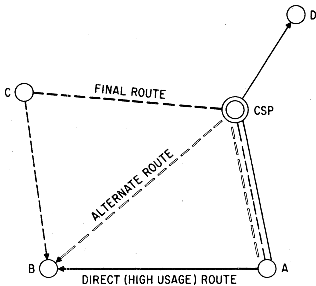
Figure 49. Trunk arrangements
