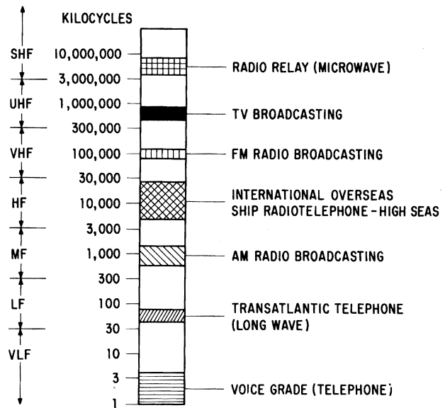
Figure A3.3 Frequency spectrum
