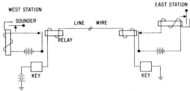
Figure A2.1 Elementary uni-polar telegraph circuit
