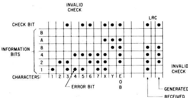
Figure 30. Error correction
