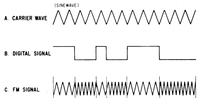
Figure 19. Frequency modulation
