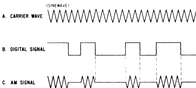
Figure 18. Amplitude modulation
