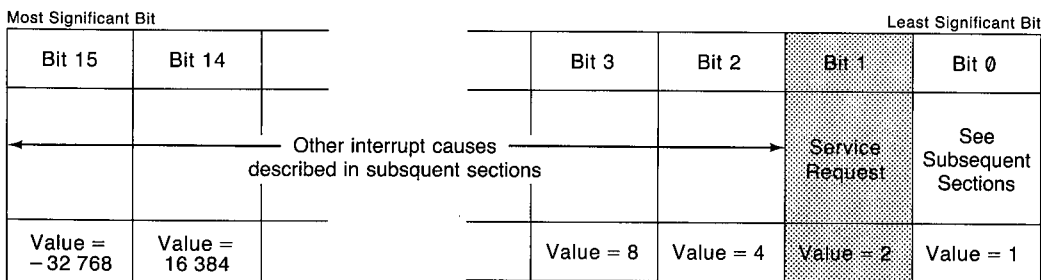
Figure 7-5. HP-IB Interrupt-Enable Register
