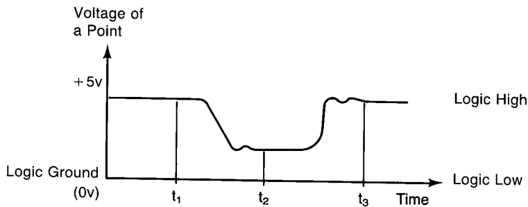
Figure 2-9. Voltage and Positive-True Logic
