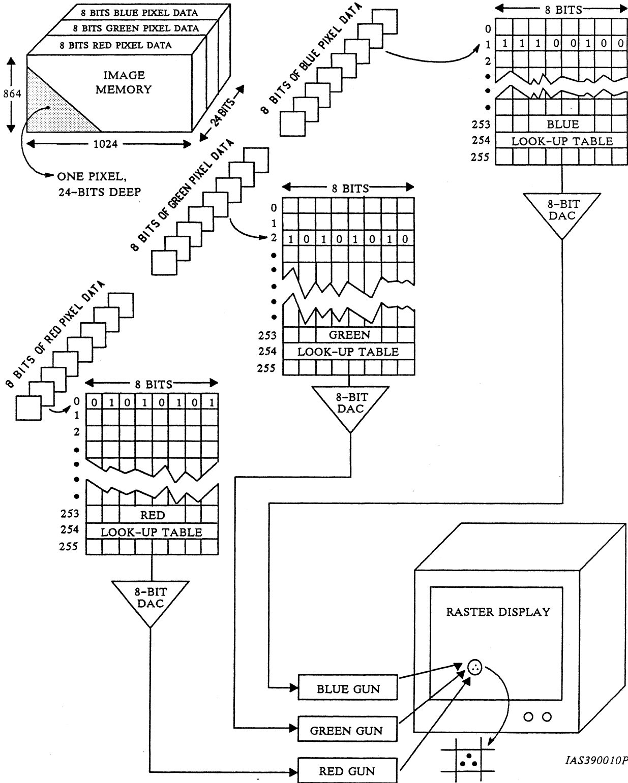
Figure 1. Pixel Mapping to Color Lookup Tables
