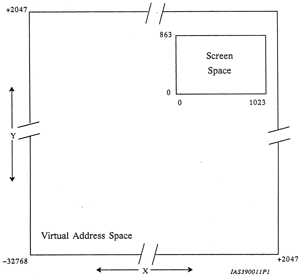
Figure 2. Virtual Address Space and Screen Space
