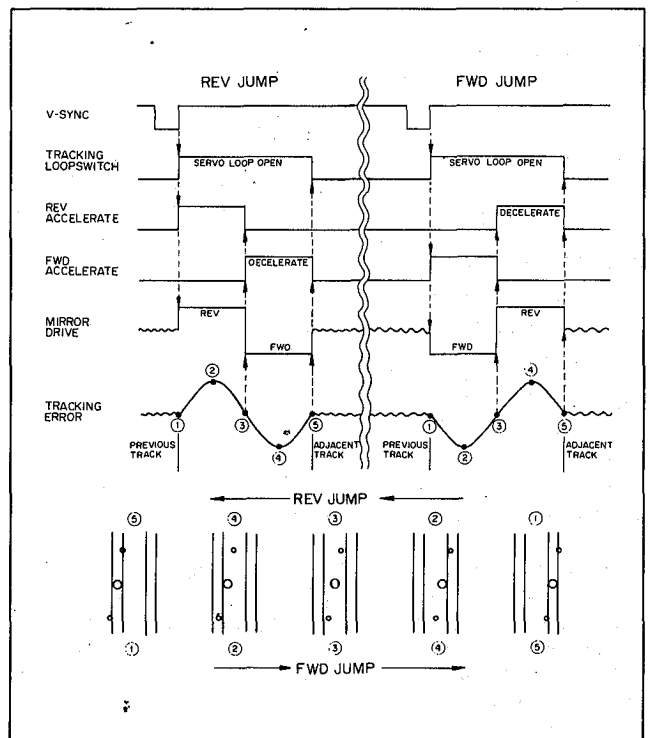
Fig. 2-19. Track jump system
