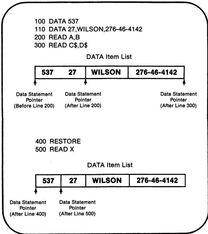
Figure 5-1. DATA Statement Pointer
