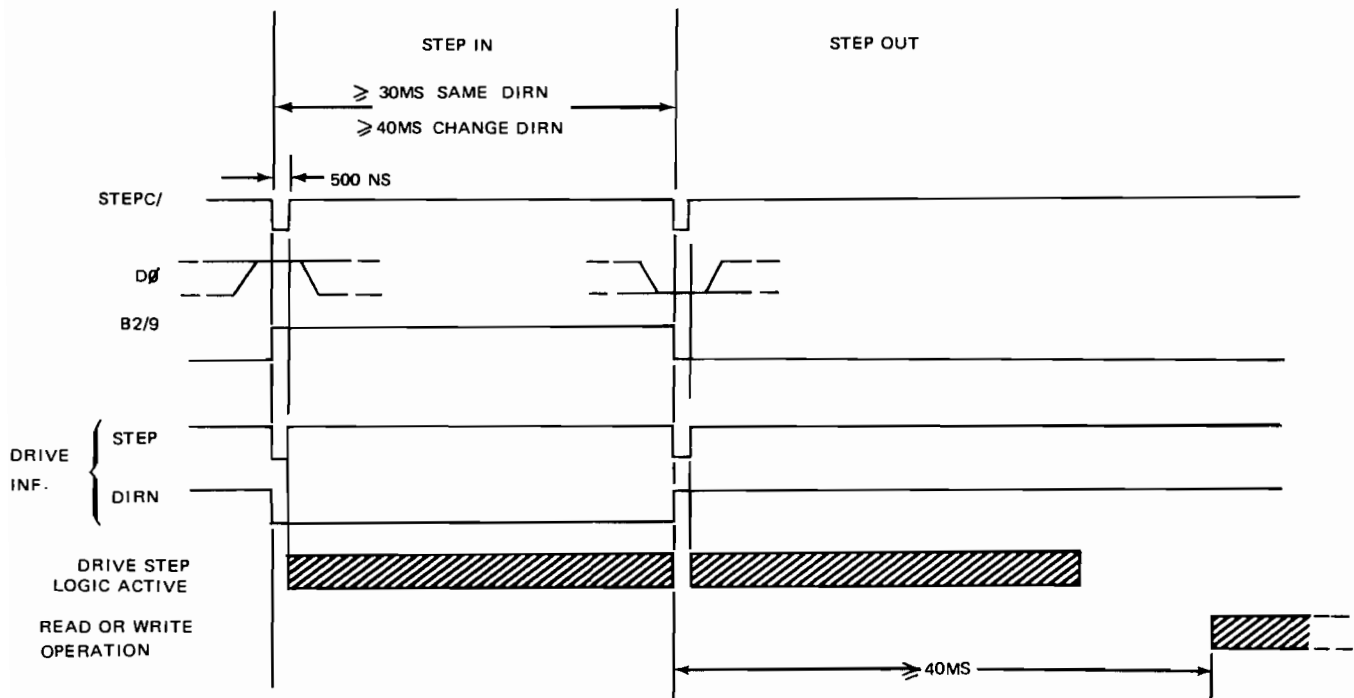
Figure 3-23. Step Control Signals, Timing Diagram
