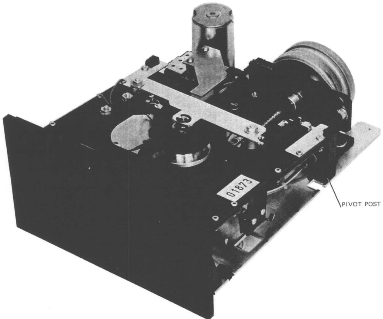
Figure 6-12. Single Drive, Top Front View, PCBA Removed
