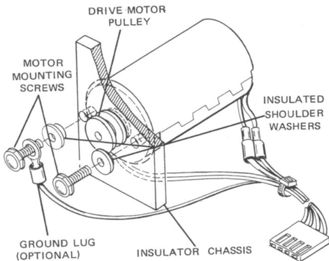
Figure 6-7. Drive Motor Installation
