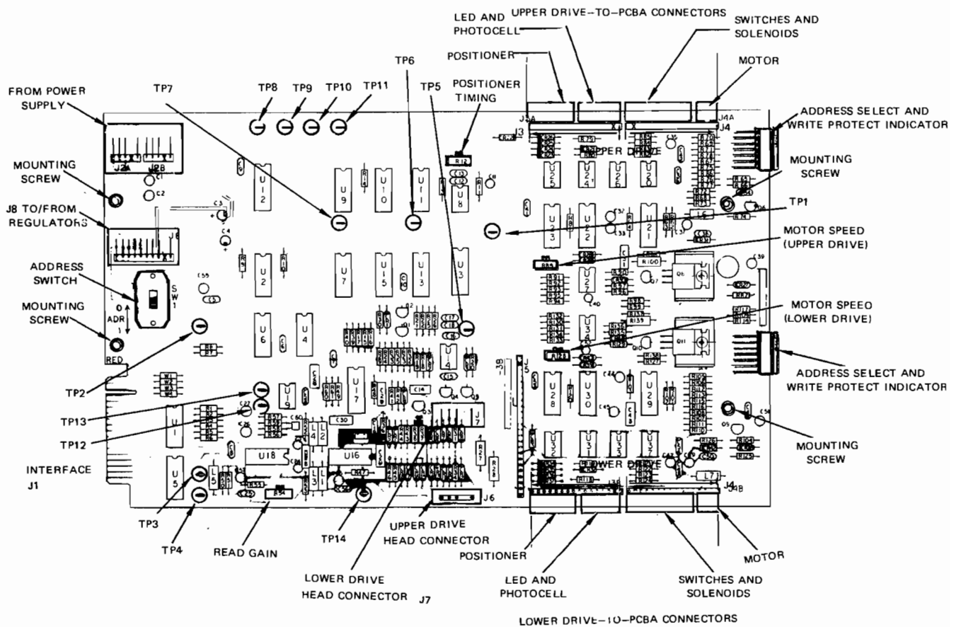
Figure 4-3. Connectors, Controls, Indicators, and Test Points for Dual Drive PCBA (P/N 100060)
