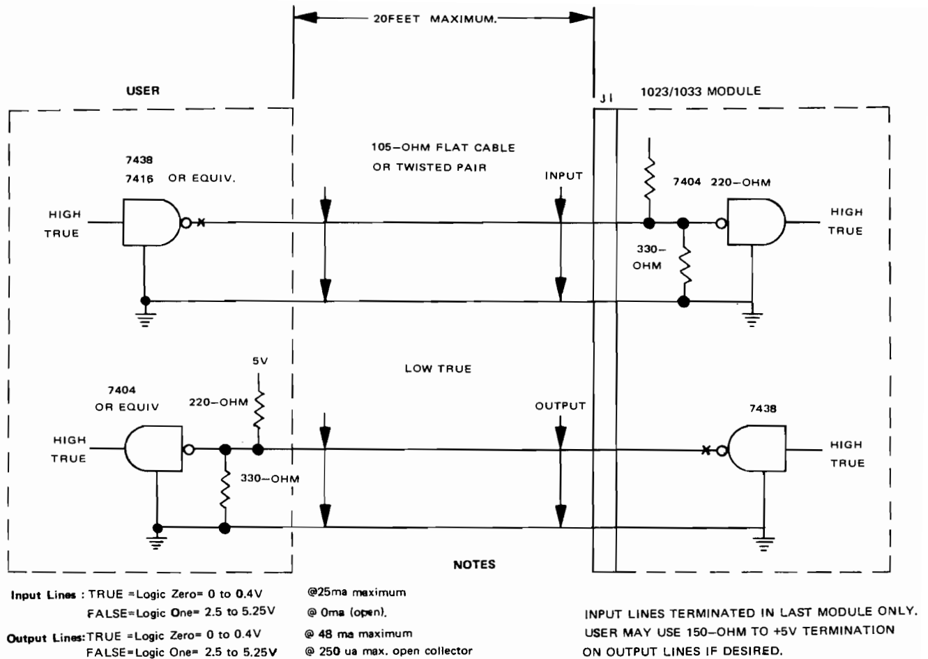
Figure 3-4. Signal Interface Characteristics
