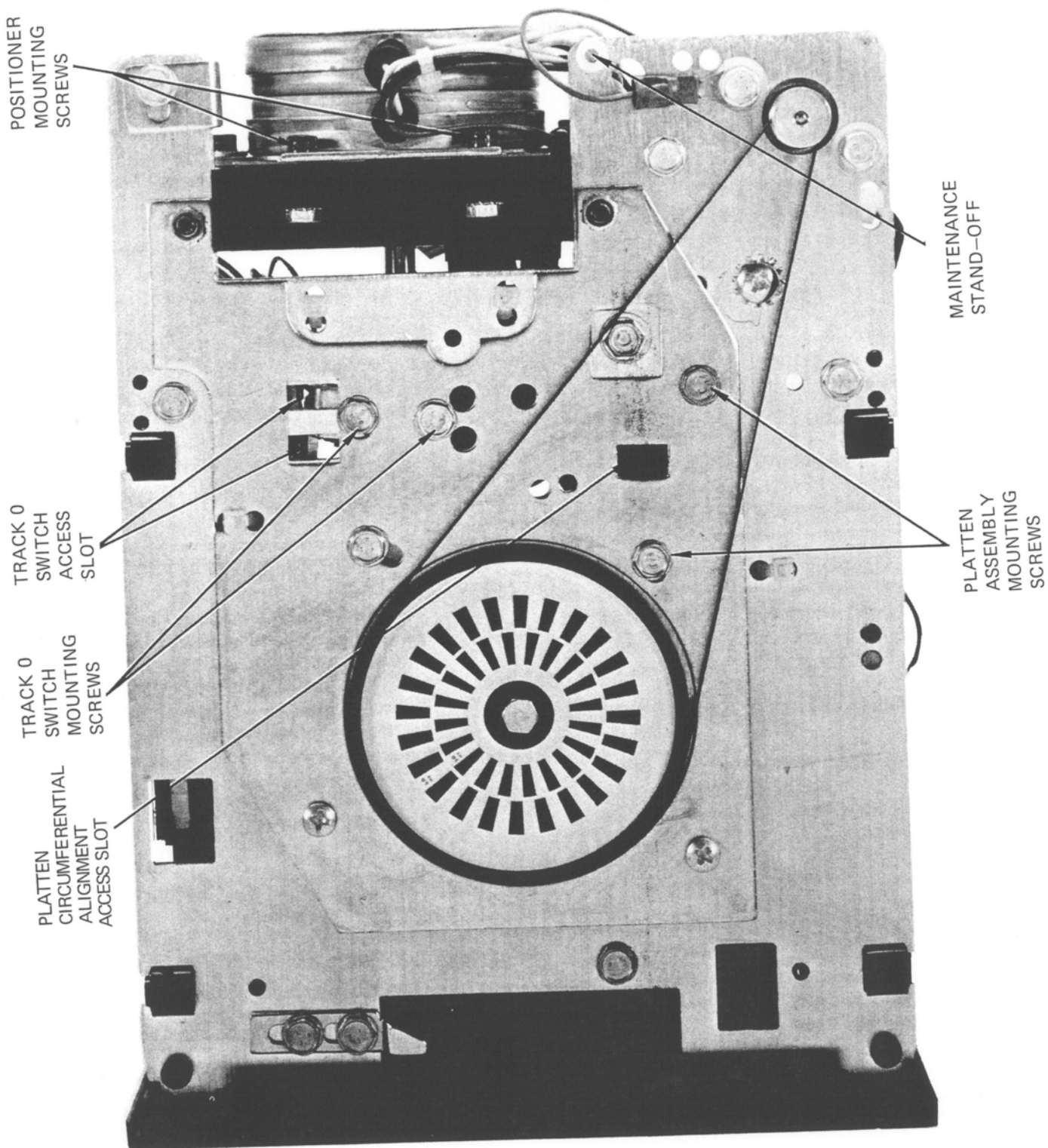
Figure 4-7. Drive Adjustment Access
