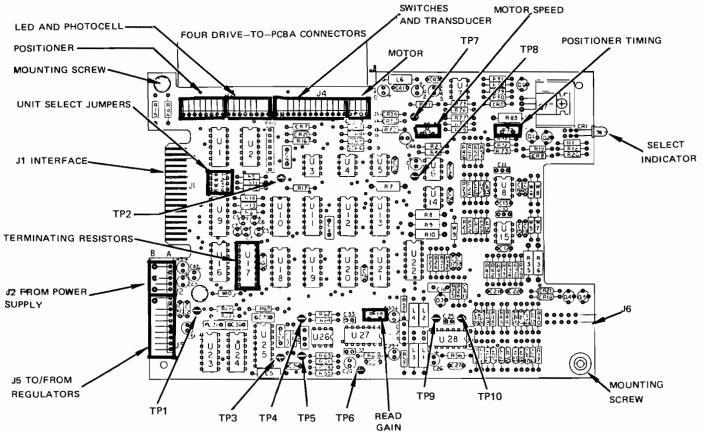
Figure 4-2. Connectors, Controls, Indicators, and Test Points for Single B Drive PCBA (P/N 100063)
