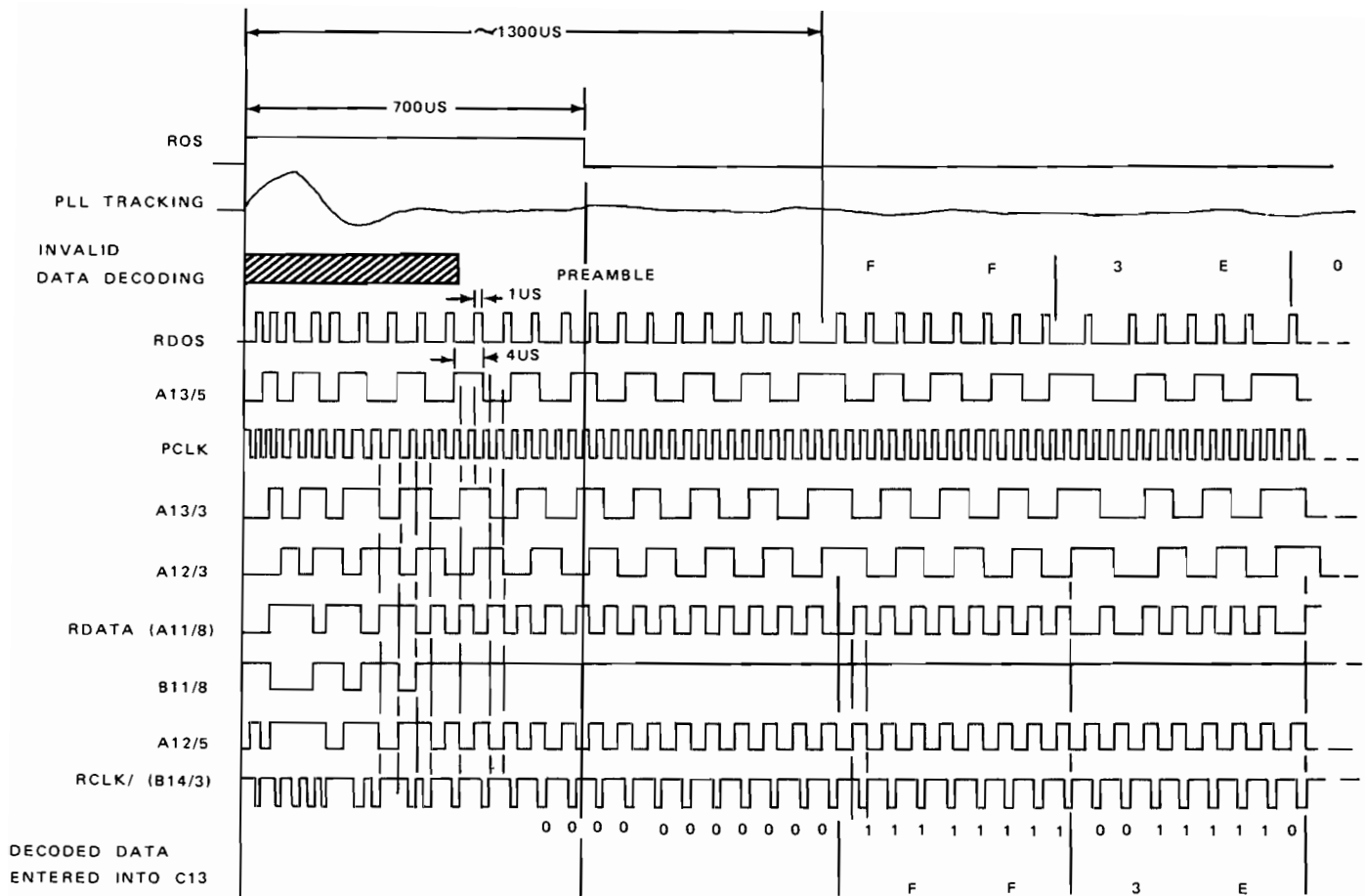
Figure 3-31. Read Decoding and Sync Circuits, Timing Diagram
