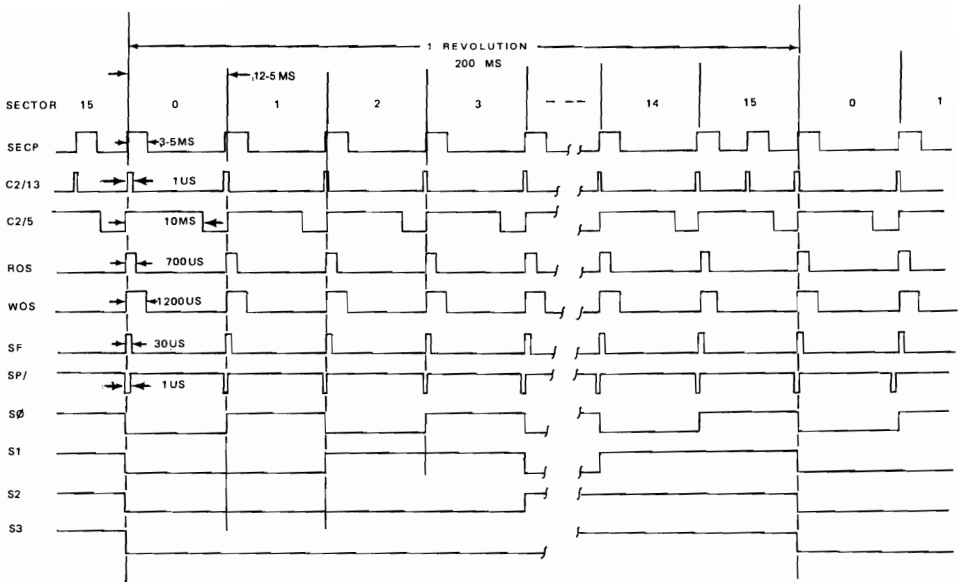
Figure 3-26. Sector Separation Signals, Timing Diagram
