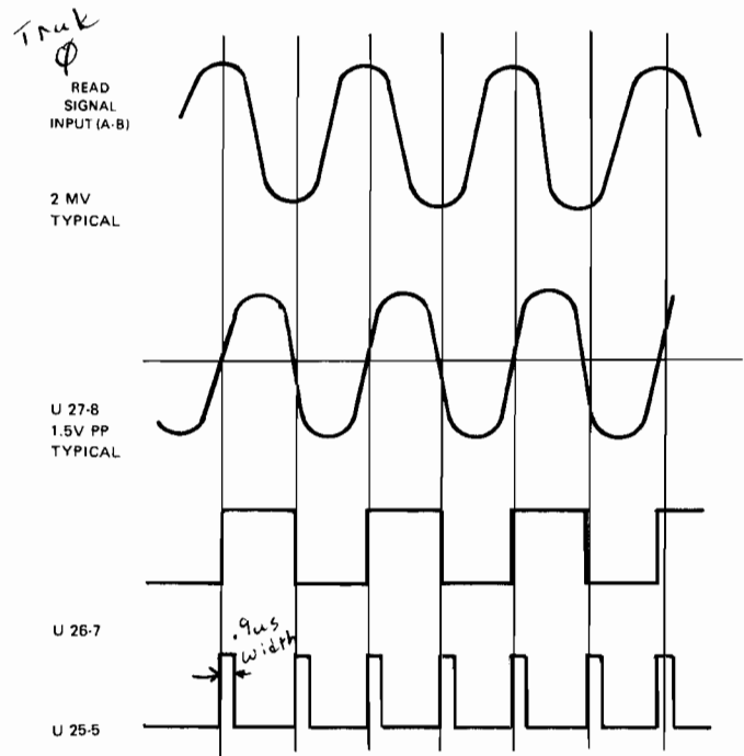
Figure 3-14. Single B Drive Read Circuits, Timing Diagram
