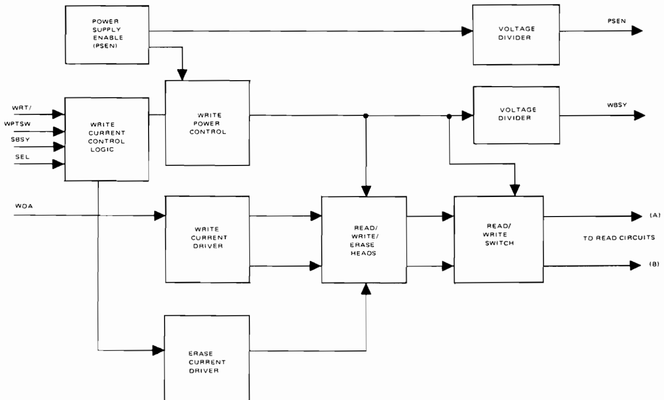
Figure 3-10. Single A Drive Write Circuits, Block Diagram
