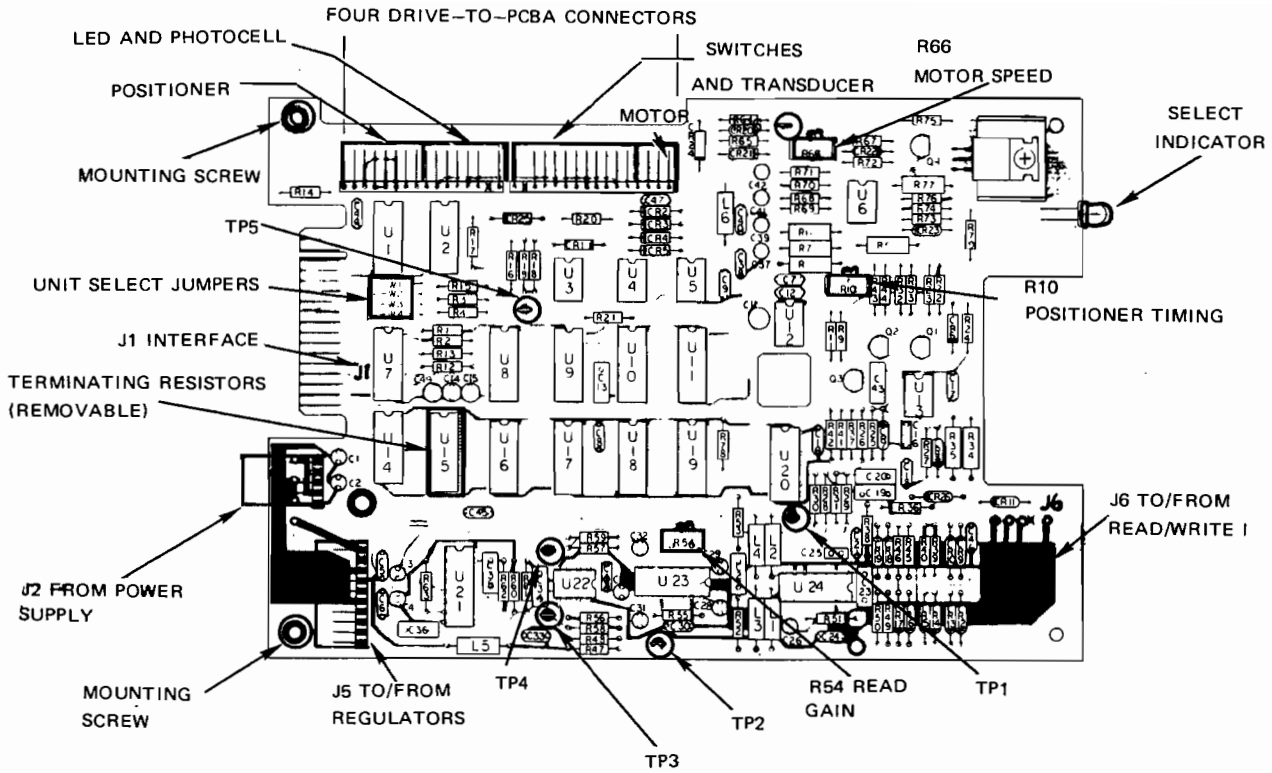
Figure 4-1. Connectors, Controls, Indicators, and Test Points for Single A Drive PCBA (P/N 100071)
