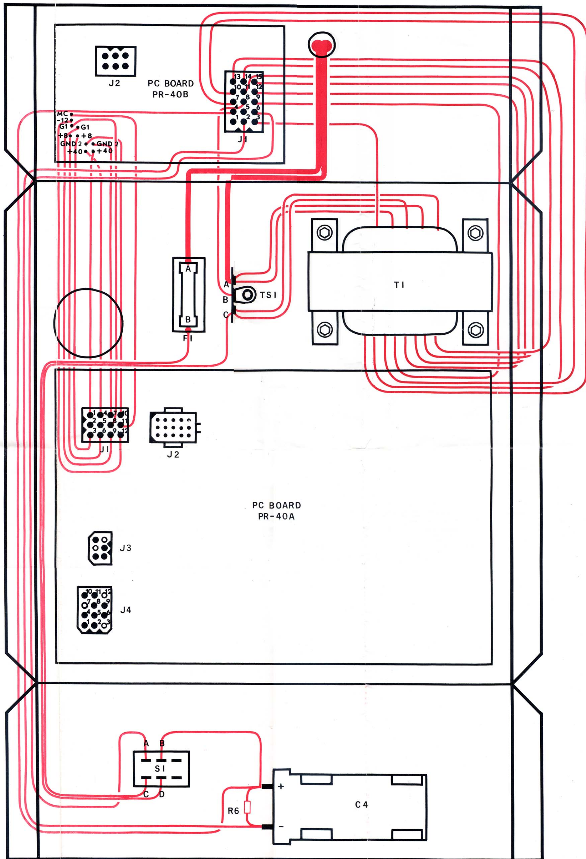
PR-40 WIRING PICTORIAL
