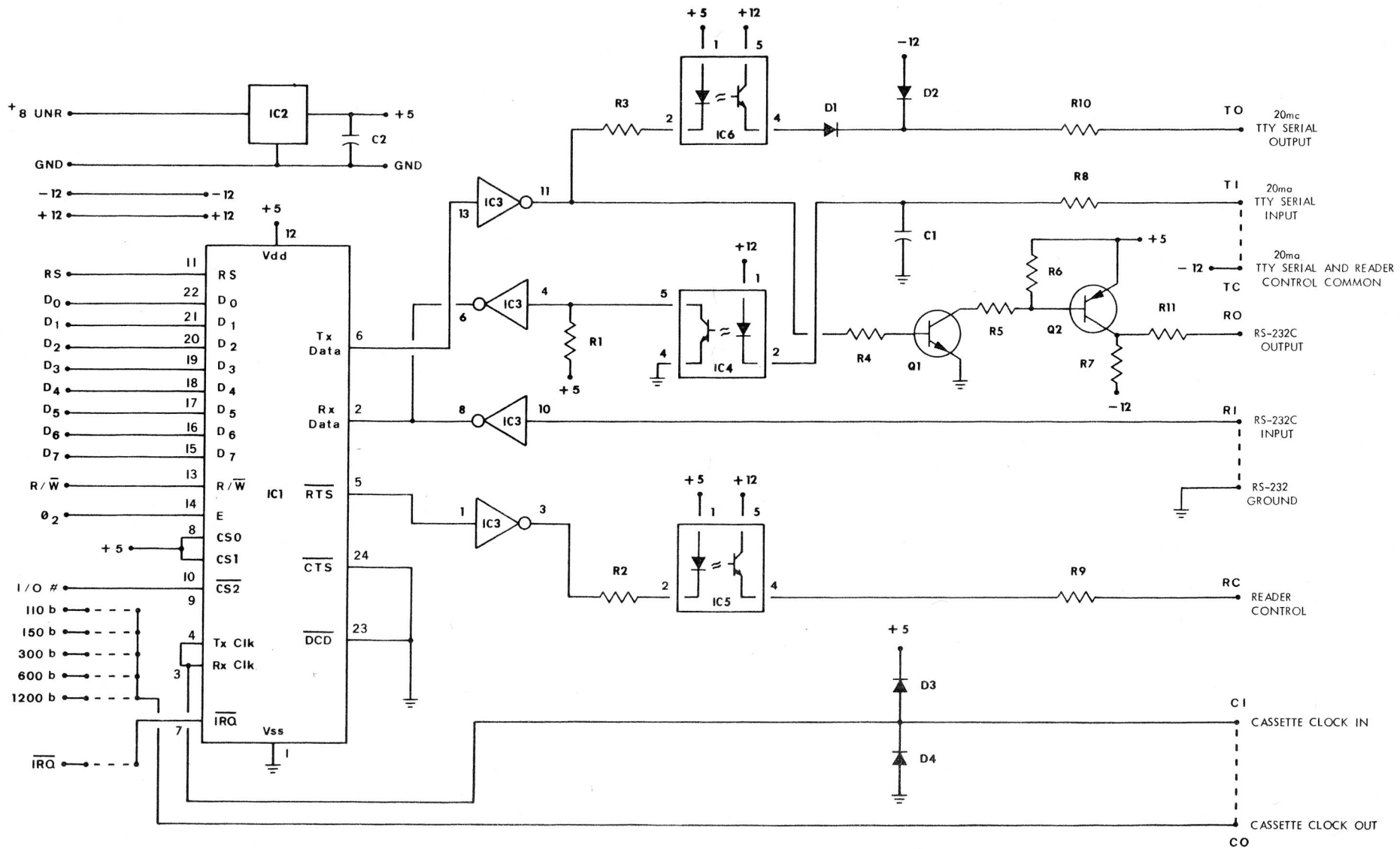
SCHEMATIC MP-S SERIAL INTERFACE
