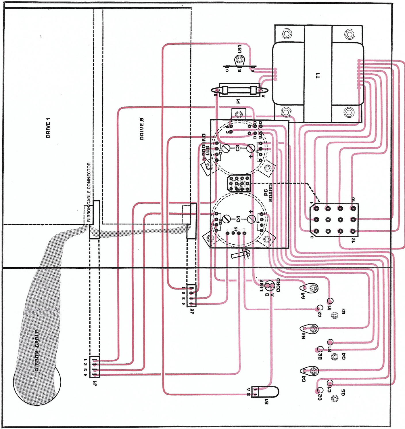
MF-69 MINIFLOPPY DISK — WIRING PICTORIAL
