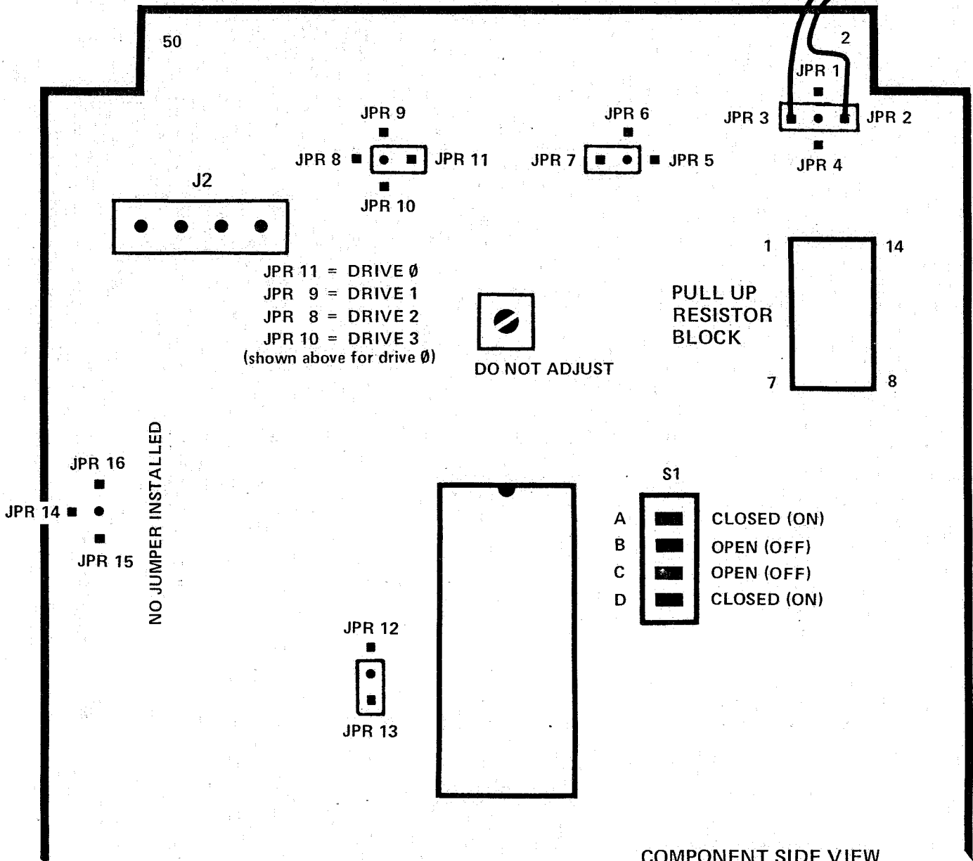
COMPONENT SIDE VIEW CORRECT JUMPERS SHOWN FOR DRIVE 0
