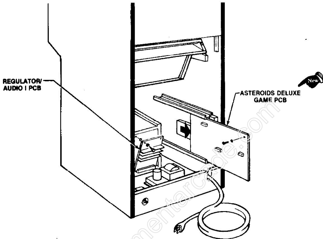
Figure 13 Printed-Circuit Board Replacement
