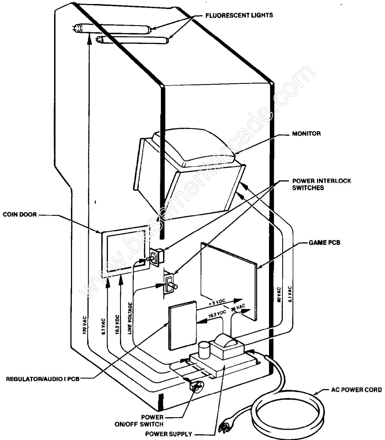
Figure 14 Power Distribution
