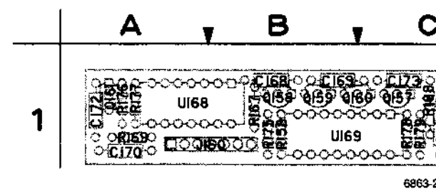
Figure 10-8. A15—Holdoff board.
