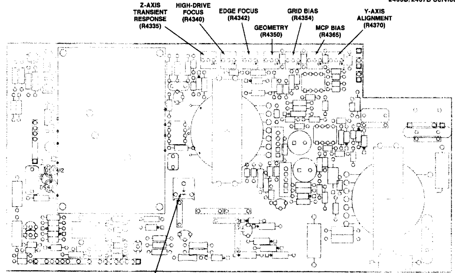
FOCUS RANGE (R4430) A9—2467B HIGH VOLTAGE, ADJUSTMENT LOCATIONS 2
