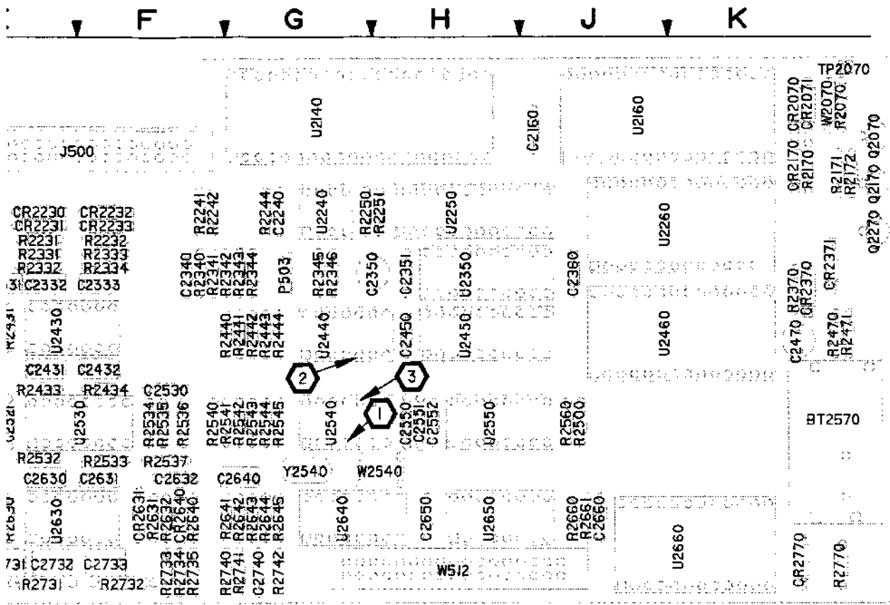
1-5b. A5—Control board (SN B049999 & Below).
