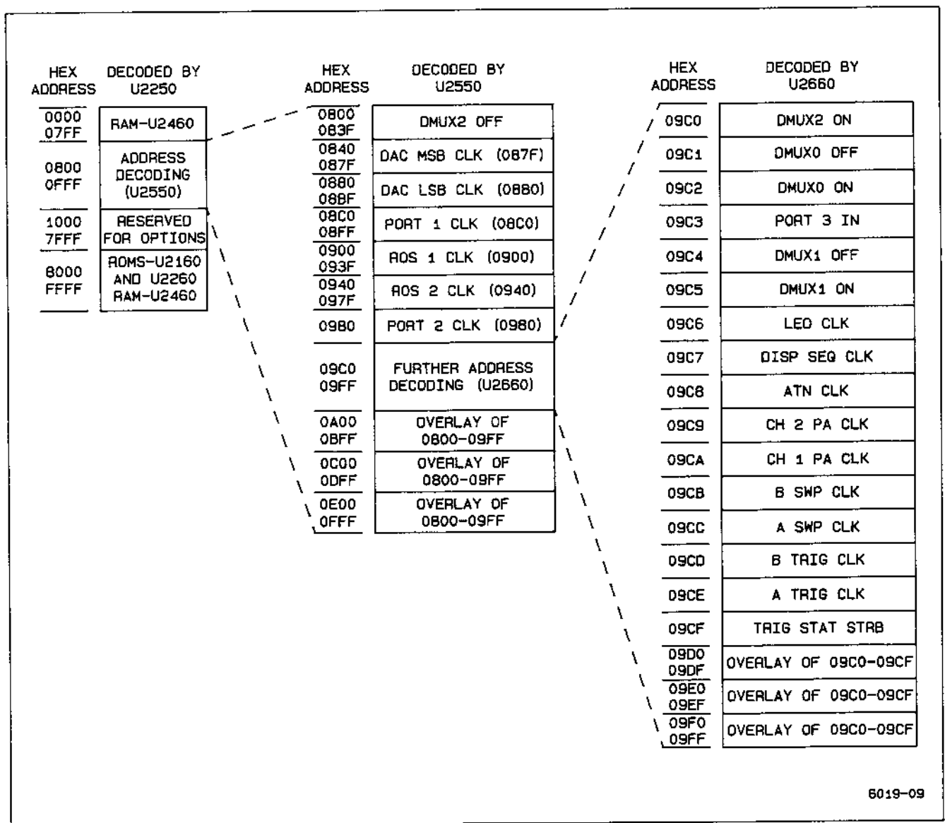
Figure 3-2. Address decoding.
