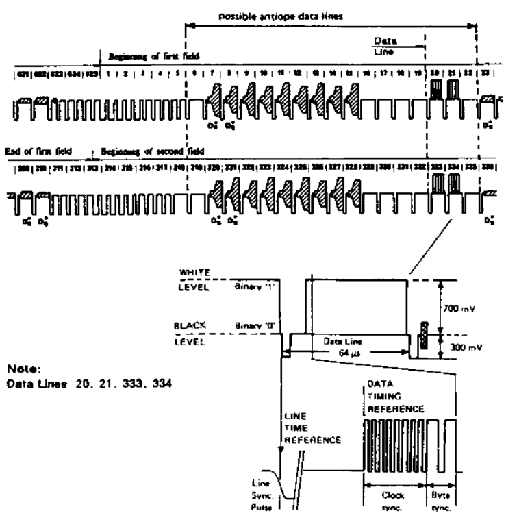
Fig. 3 Identification and Levels of Antiope Data Lines
