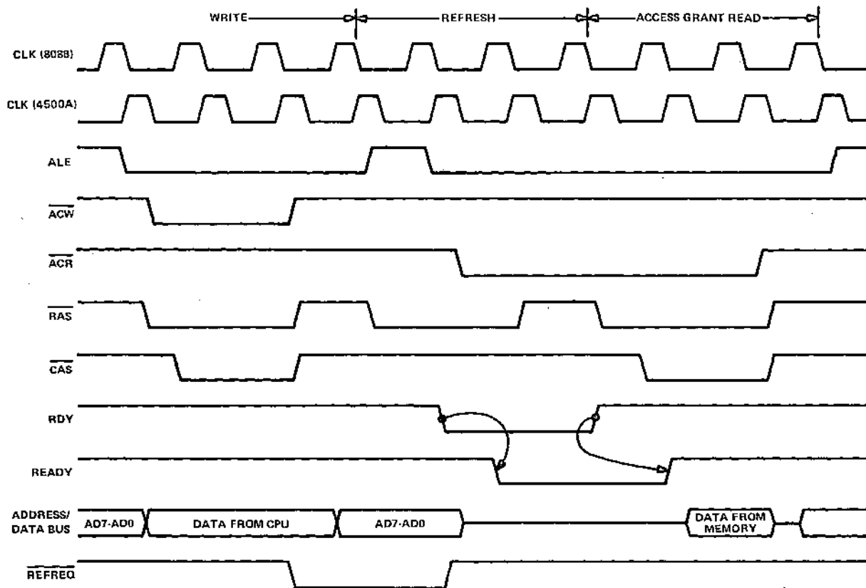
FIGURE 2 - TIMING DIAGRAM
