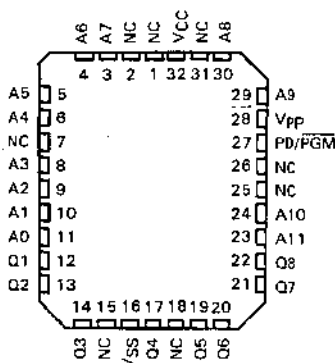
SMJ2532 . . . FE PACKAGE
