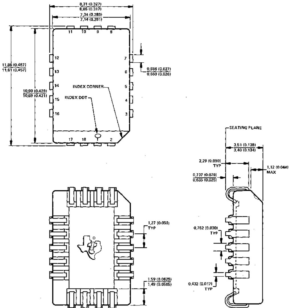
Figure 1. Plastic Chip Carrier Package (FP Suffix)
