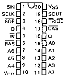
TMS4161 . . . NL PACKAGE (TOP VIEW)
