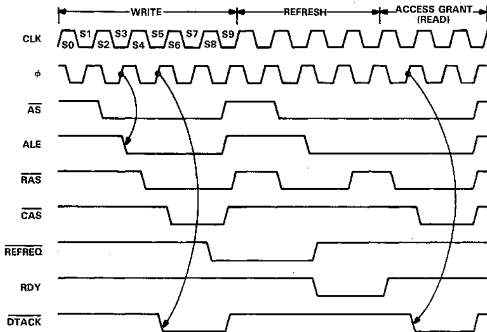
FIGURE 4B - TMS4500A/MC68000LB-MC68000L10 TIMING DIAGRAM
