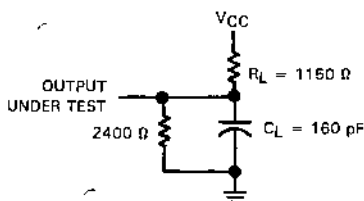
FIGURE 1 - LOAD CIRCUIT
