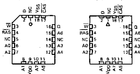
SMJ4164 . . . FE PACKAGE (TOP VIEW)
