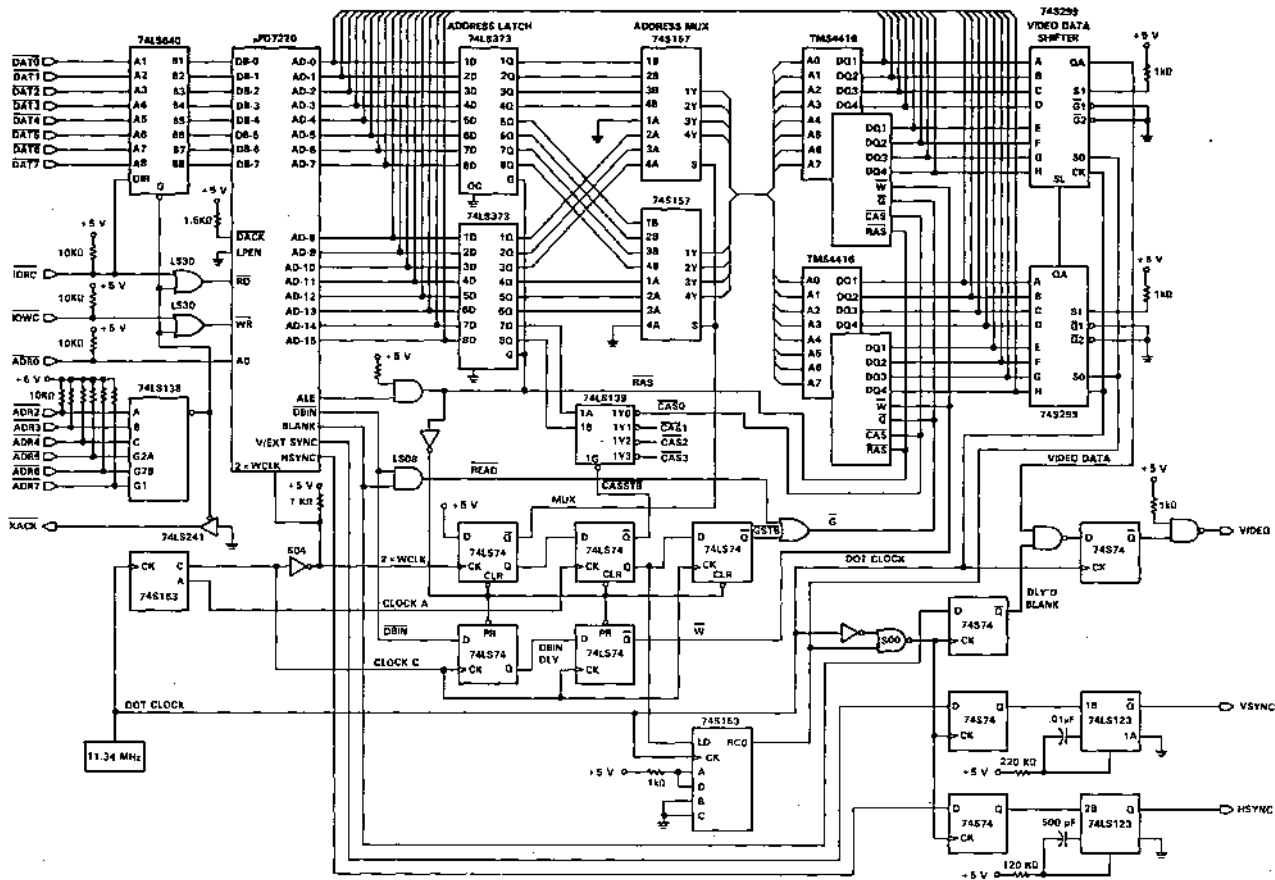
Figure 1. TMS4416/7220 Interface
