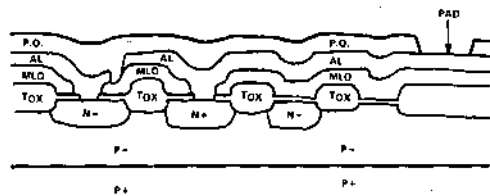
FIGURE 2B - CROSS SECTION OF CLAMPING CIRCUIT
