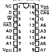
TMS4164 . . . FPL PACKAGE SMJ4164 . . . FG PACKAGE (TOP VIEW)
