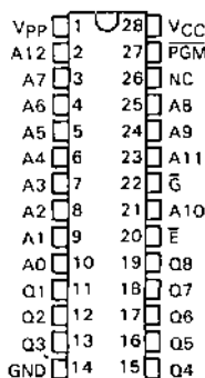
TMS2764 . . . J1 PACKAGE (TOP VIEW)
