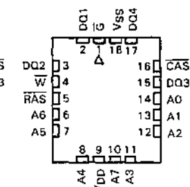
SMJ4416 . . . FG PACKAGE (TOP VIEW)
