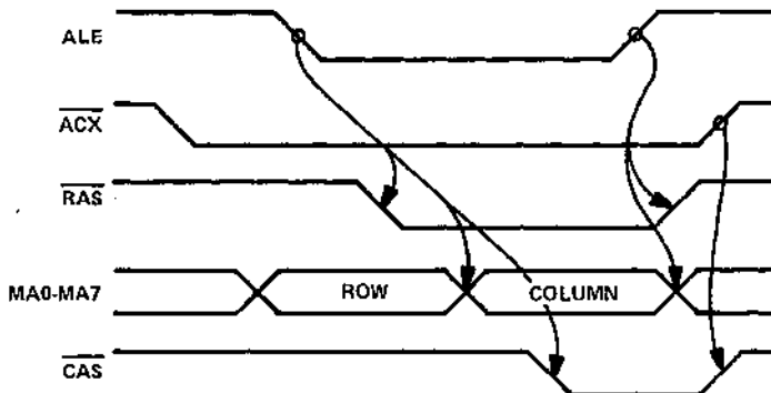
FIGURE 4 — \overline{ACX} OVERLAPPING \overline{ALE}
