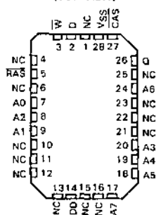
SMJ4164 . . . FE PACKAGE (TOP VIEW)
