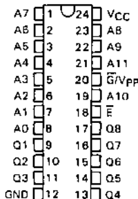
TMS2732A . . . JL PACKAGE (TOP VIEW)
