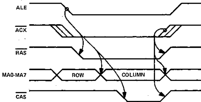
FIGURE 3 — \overline{ACX} PRIOR TO OR COINCIDENT WITH ALE
