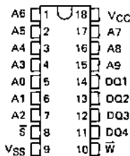
TMS2114, TMS2114L . . . NL PACKAGE (TOP VIEW)
