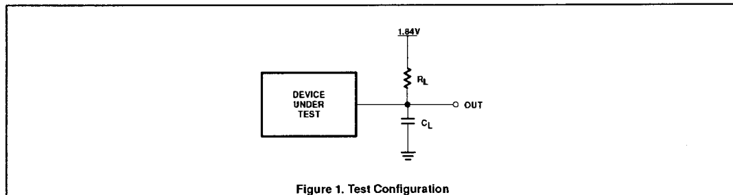
Figure 1. Test Configuration
