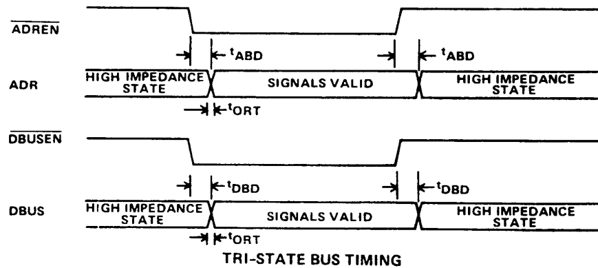
Figure 9. 2650 TIMING DIAGRAMS
