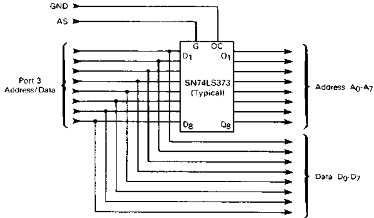
FIGURE 14 — TYPICAL LATCH ARRANGEMENT
