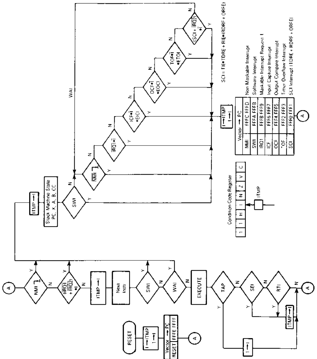
FIGURE 18 - INTERRUPT FLOWCHART
