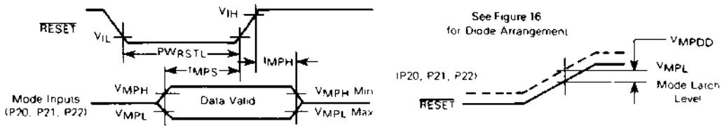
FIGURE 15 — MODE PROGRAMMING TIMING
