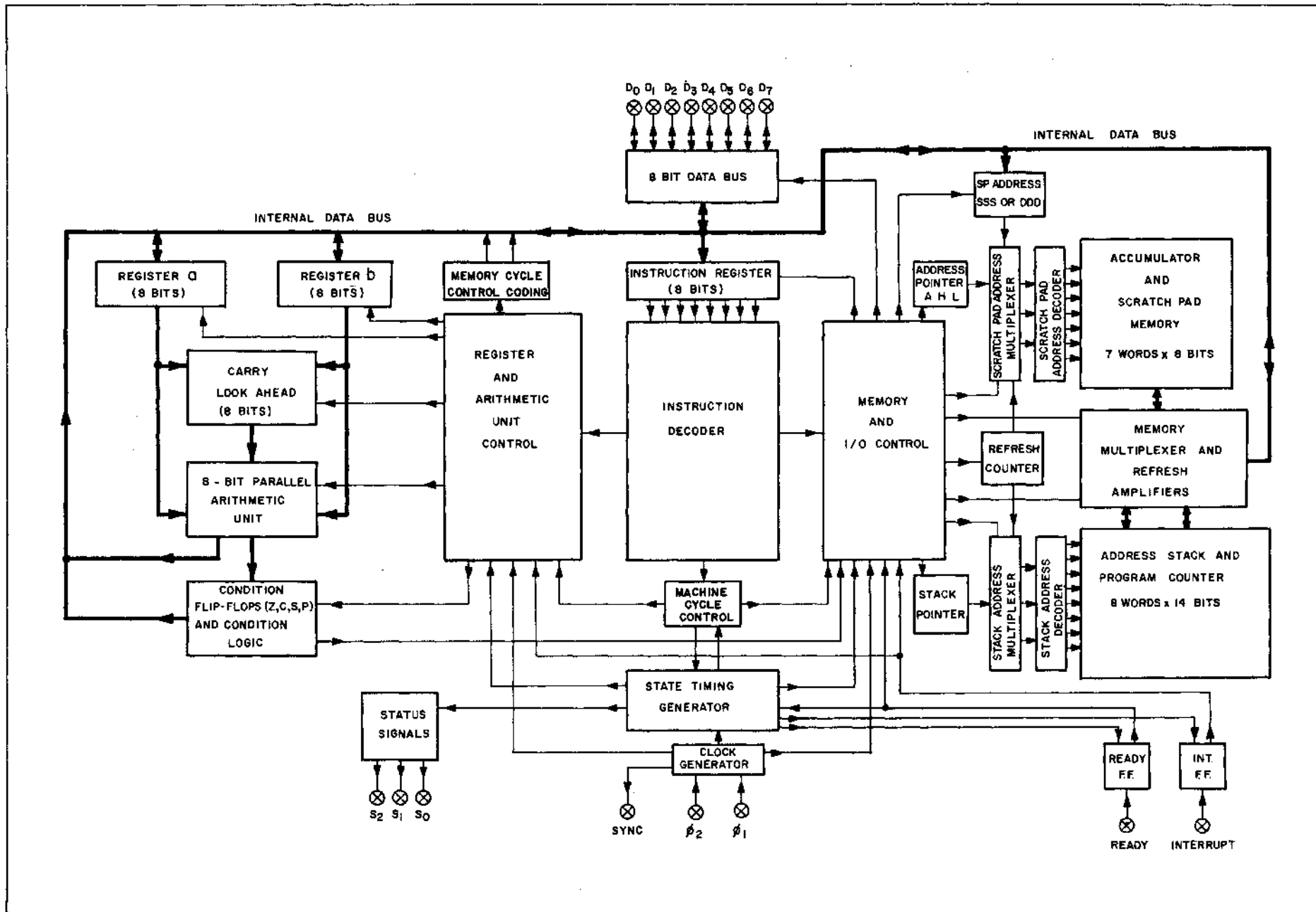
Figure 3. 8008 Block Diagram
