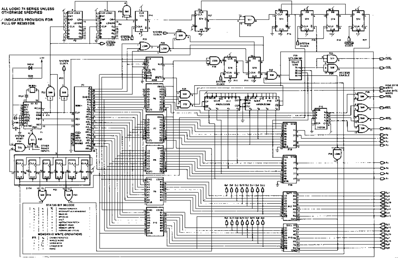
Figure 31. Logic Diagram — 10 MHz System
