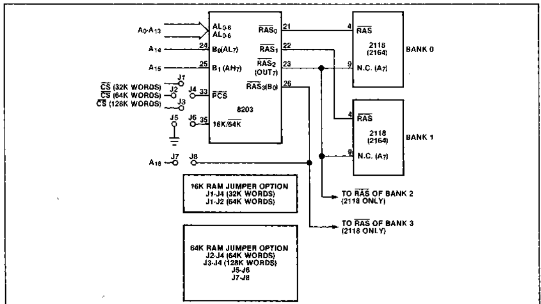
Figure 20. 8203 Jumper Options
