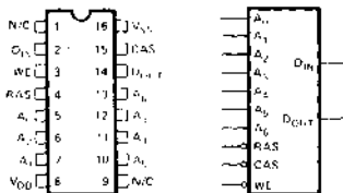
PIN CONFIGURATION LOGIC SYMBOL
