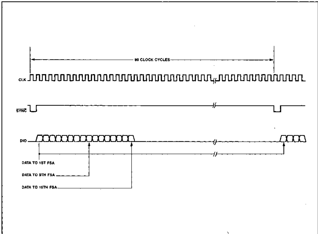
Figure 5. Data Sequences
