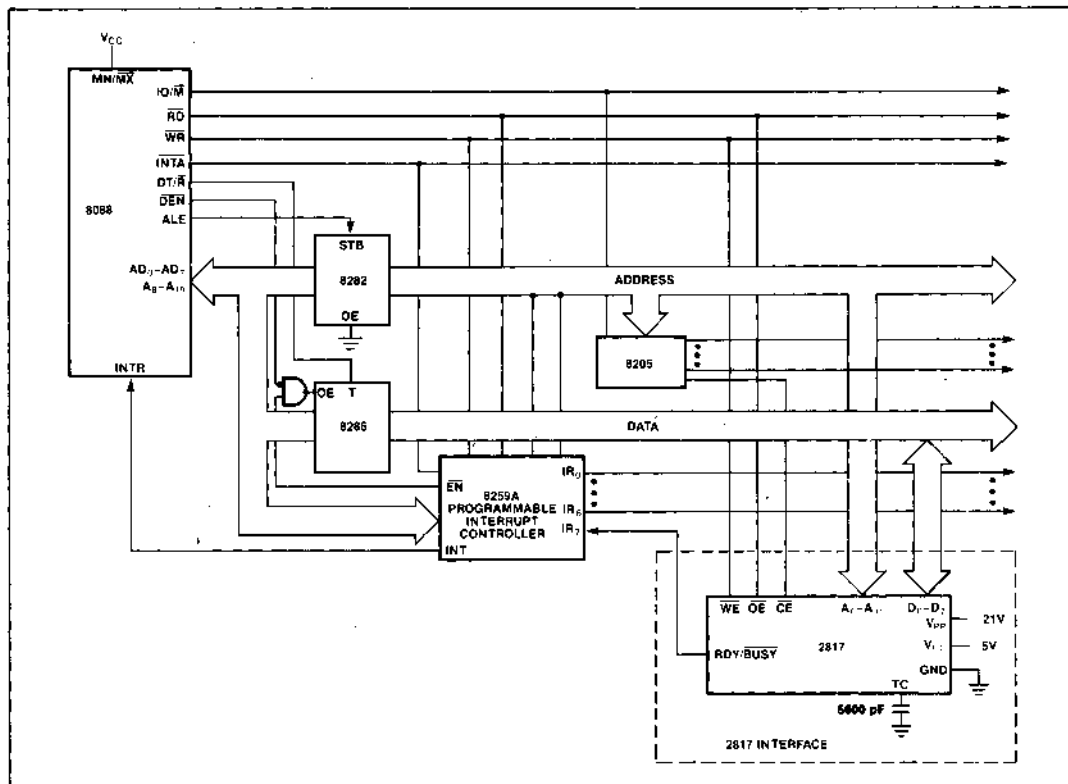
Figure 7. 2817/8088 Interface Example
