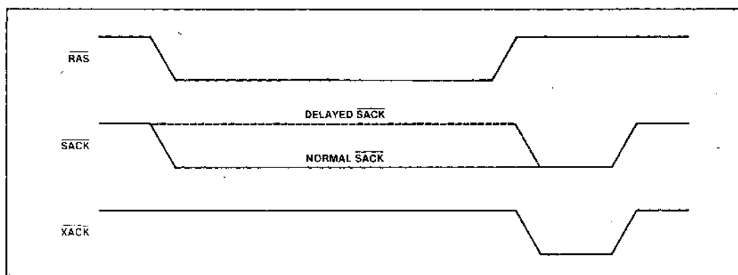
Figure 18. Delayed \overline{SACK} Mode
