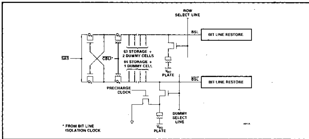
Figure 6. Sense Amp
