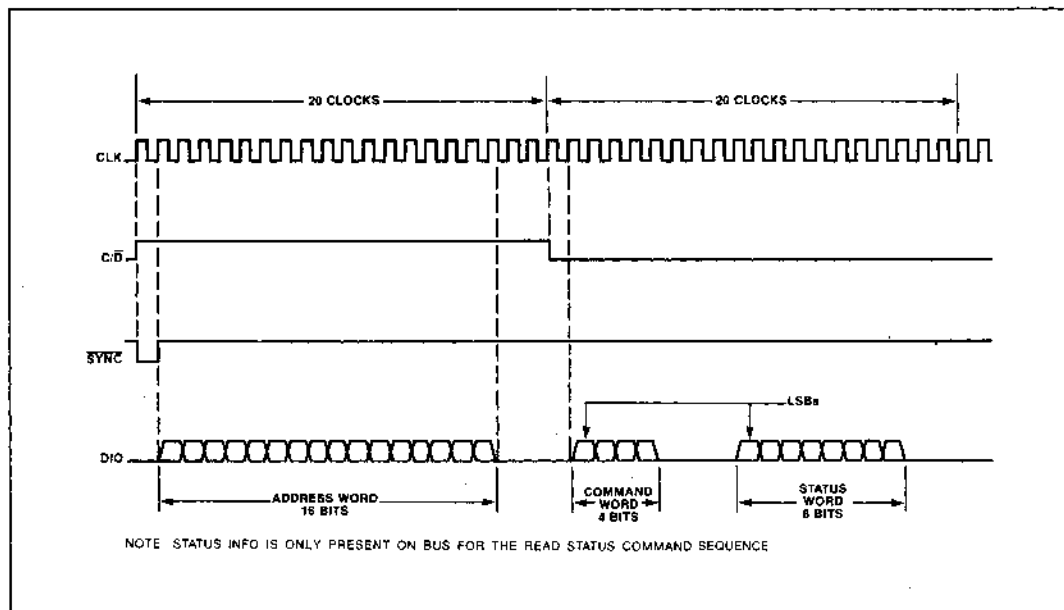
Figure 4. Command Sequences
