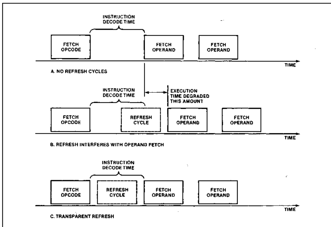
Figure 9. Transparent Refresh
