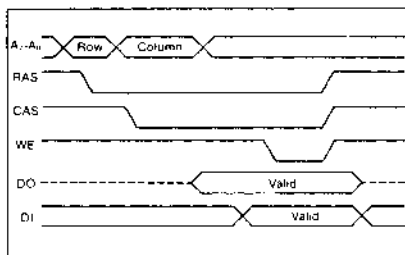
8. In all memory cycles, the row and column addresses are strobed to the RAMs by RAS and CAS. Sometimes after the data out is valid, the control logic in Fig. 7b generates Write Enable ( \overline{WE} ) to write the data back into the RAMs.
