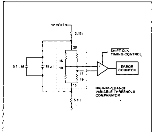
Figure 8. Test Setup for Output Measurement
