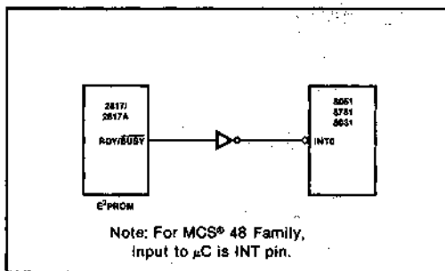
Figure 7. Interrupt-Driven Microcontroller System
