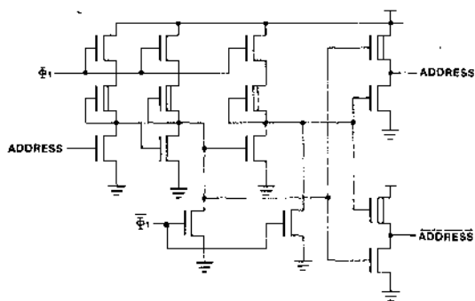
Figure 4. Address Buffer.
