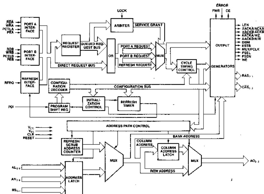
Figure 1. 8207 Block Diagram
