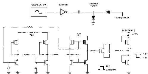
Figure 8. 2147H Substrate Bias Generator
