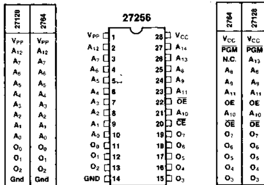
Figure 2. Pin Configurations
