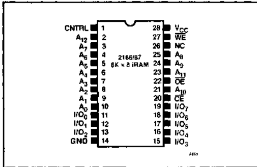
Figure 11. 2186/87 Pinout
