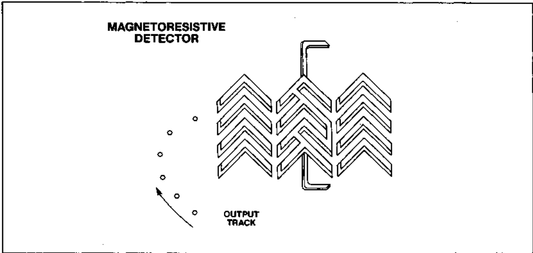
Figure 9. Bubble Detection
