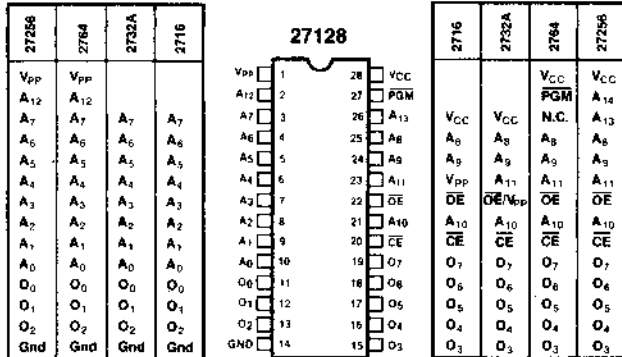
Figure 2. Pin Configurations NOTE: INTEL UNIVERSAL SITE COMPATIBLE EPROM PIN CONFIGURATIONS ARE SHOWN IN THE BLOCKS ADJACENT TO THE 27128 PINS
