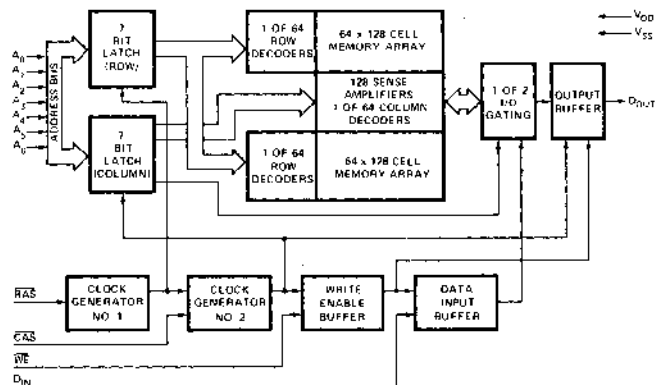
BLOCK DIAGRAM
