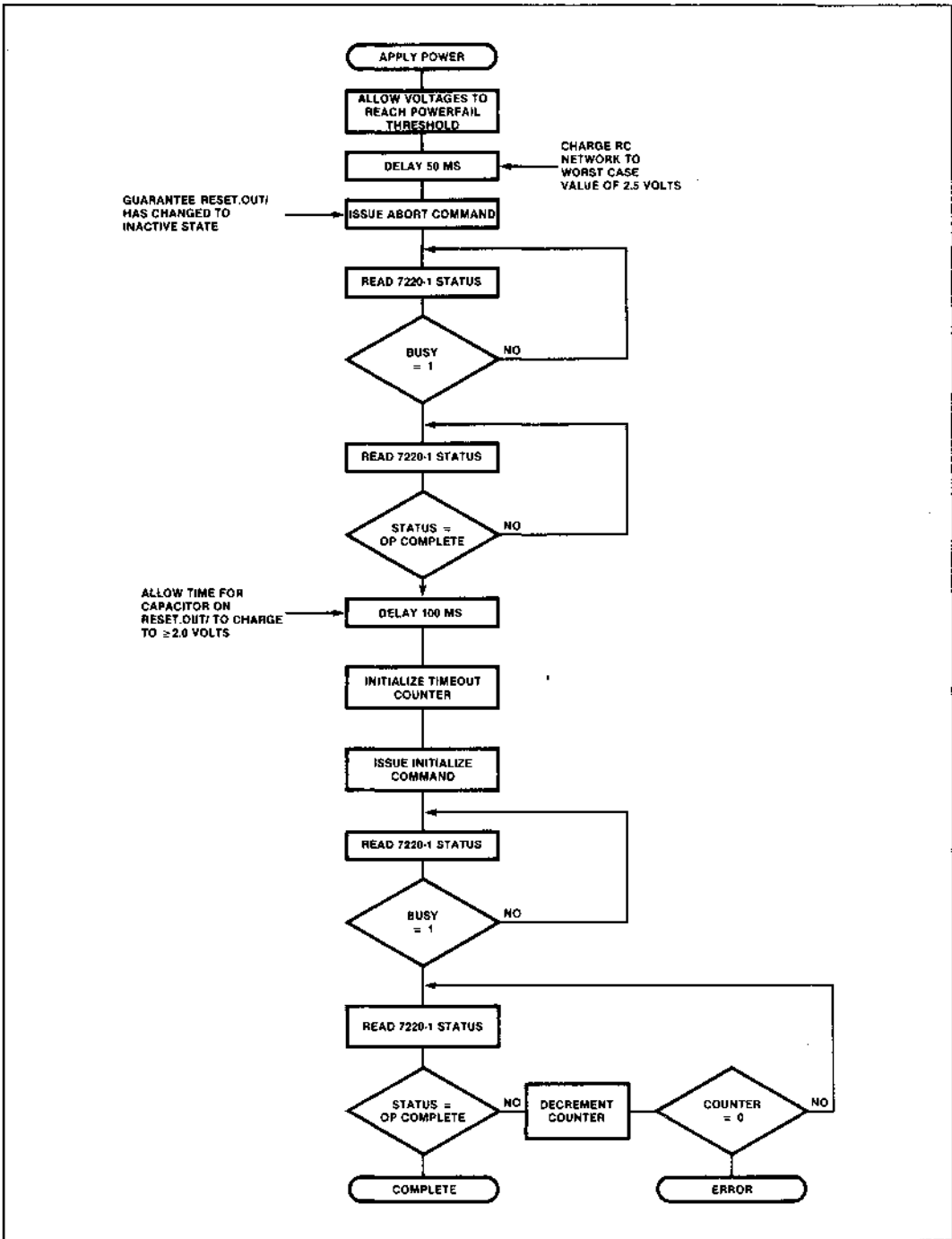
Figure 4. Power-up Flowchart
