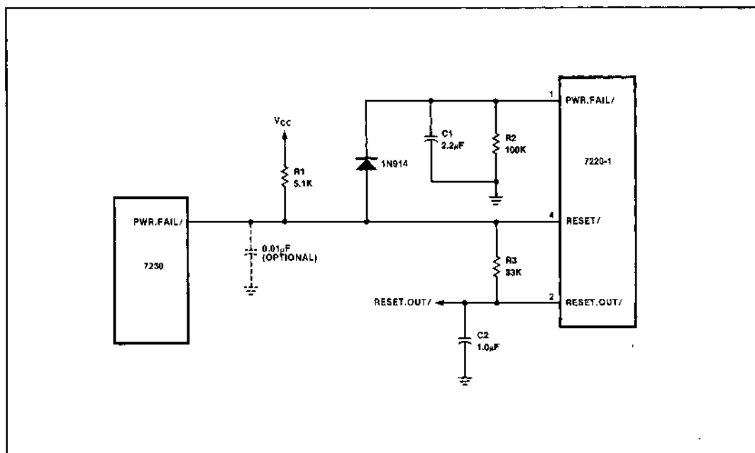
Figure 11. Revision 1 Circuit
