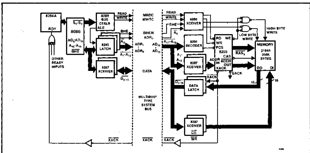
Figure 17. 8203/2164A Global Memory System
