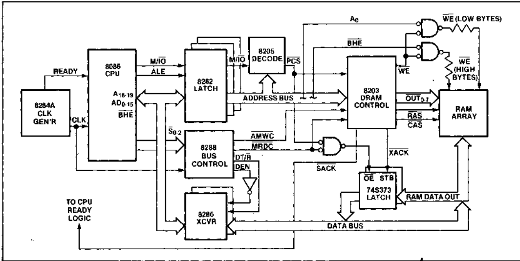
Figure 23. 8086 Maximum Mode
