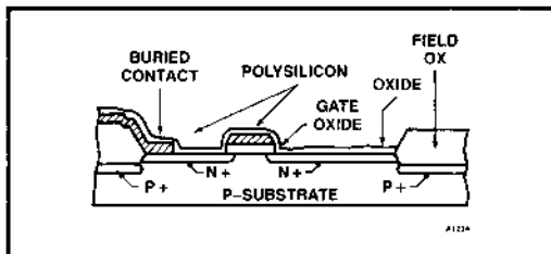
Figure 5. Post Oxidation
