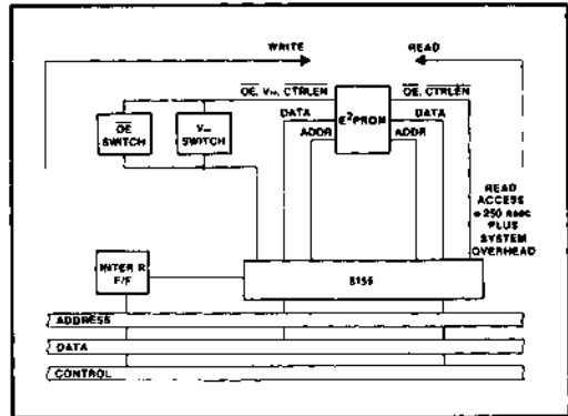
Figure 10. Controller IV
