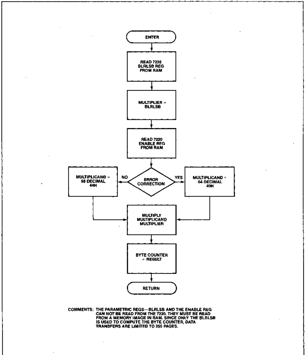
Figure 13. BYTCNT
