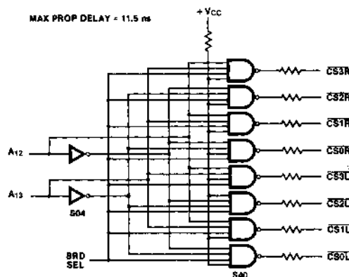
Figure 31. CS Decode
