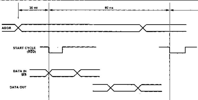
Figure 27. System Timing
