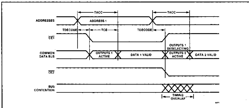
Figure 7. One-line Control
