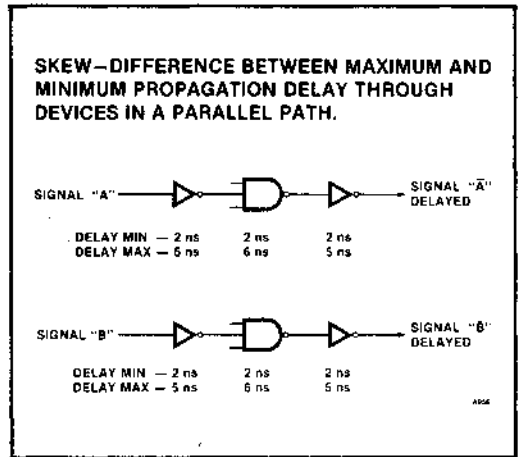
Figure 36. Skew
