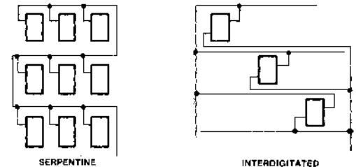
Figure 17. Pseudo-Gridding Techniques
