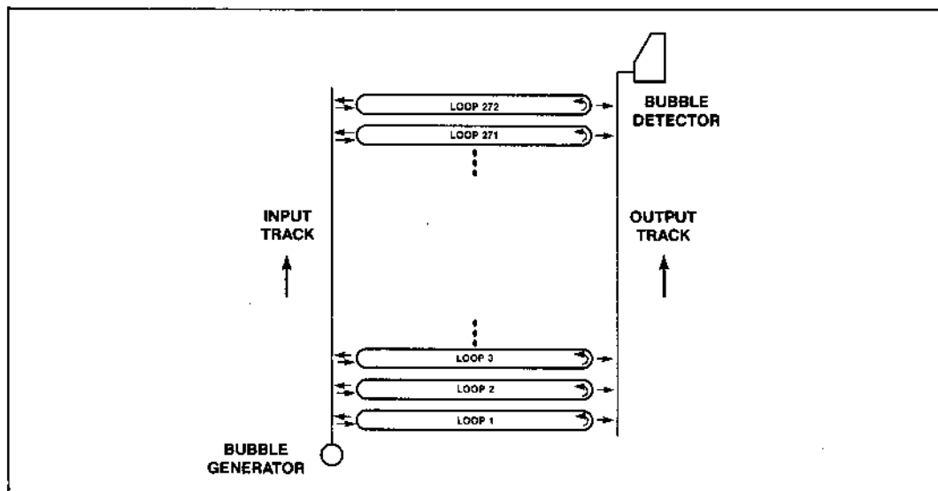
Figure 6. Block-Replicate Architecture
