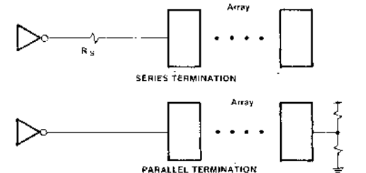
Figure 23. Series and Parallel Termination
