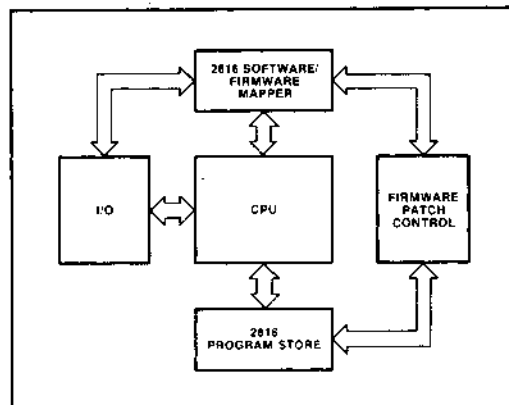
Figure 13. Dynamic Reconfiguration
