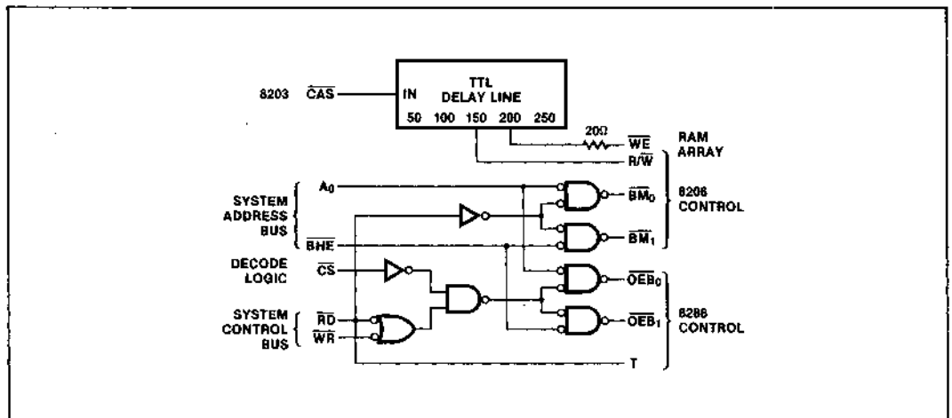
Figure 2. Interface Logic
