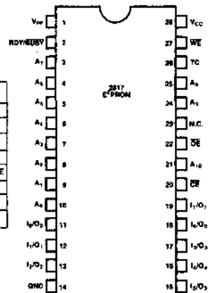
Figure 2. 2817 Pin Configuration
