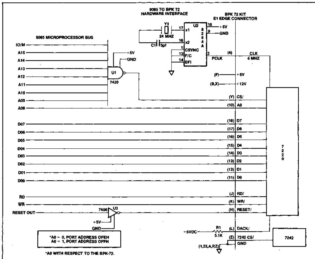
Figure 2. Hardware Interface
