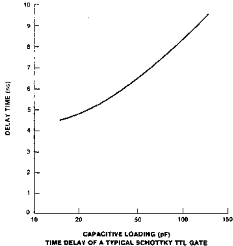
Figure 25. Capacitive Loading
