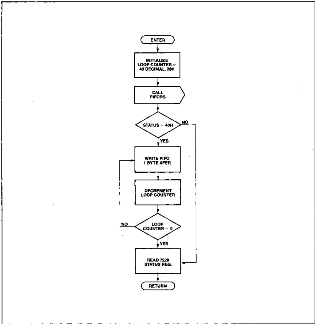
Figure 22. WRFIFO
