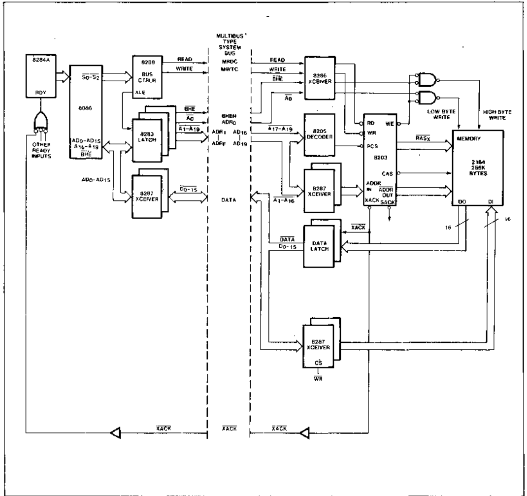
Figure 11. 8086/256K Byte System
