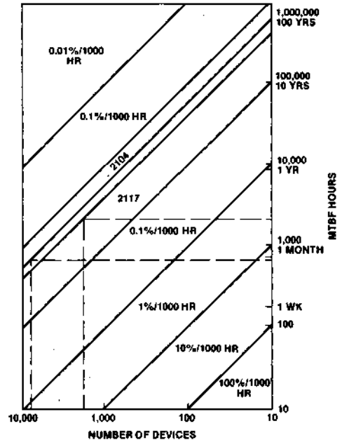
Figure 1. System Reliability vs Number of Devices
