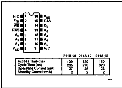
Figure 2. Intel® 2118 Pinout
