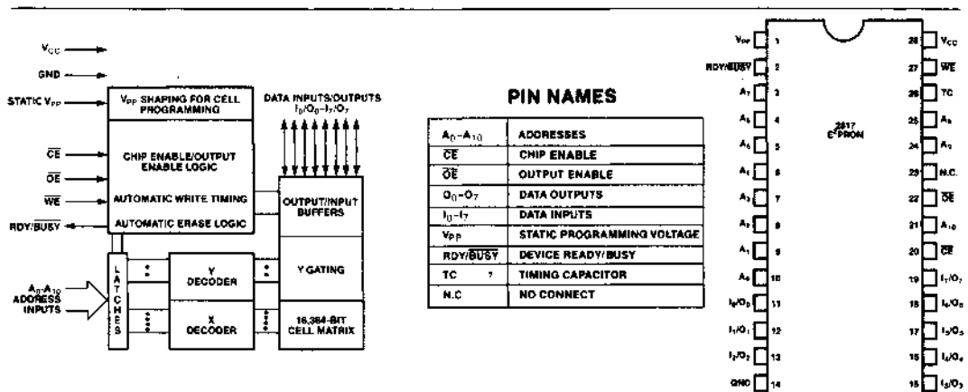
Figure 1. 2817 Functional Block Diagram
