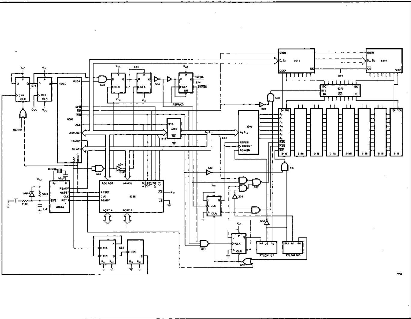
Figure 24. Discrete DRAM Controller
