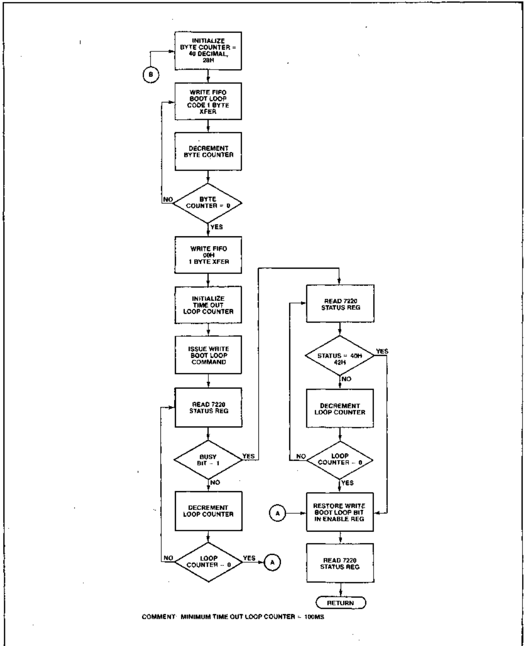
Figure 20 (Con't). BOOTUP
