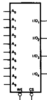
LOGIC SYMBOL
