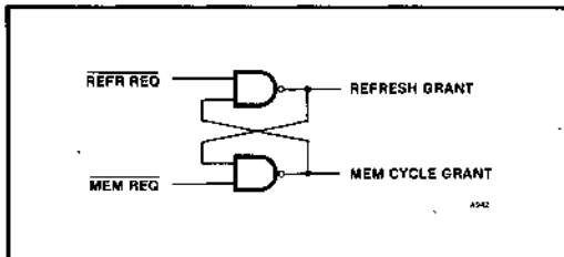
Figure 10. Arbiter Cross-coupled NAND Gates
