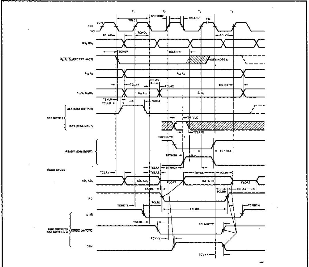
Figure 18. 8086 Bus Timing — Maximum Mode System (using 8288)
