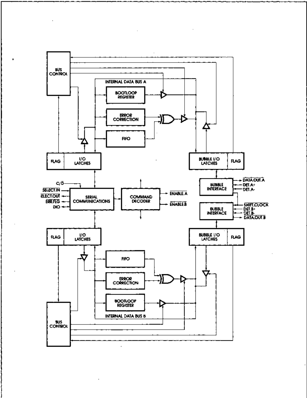
Figure 3. Logic Diagram
