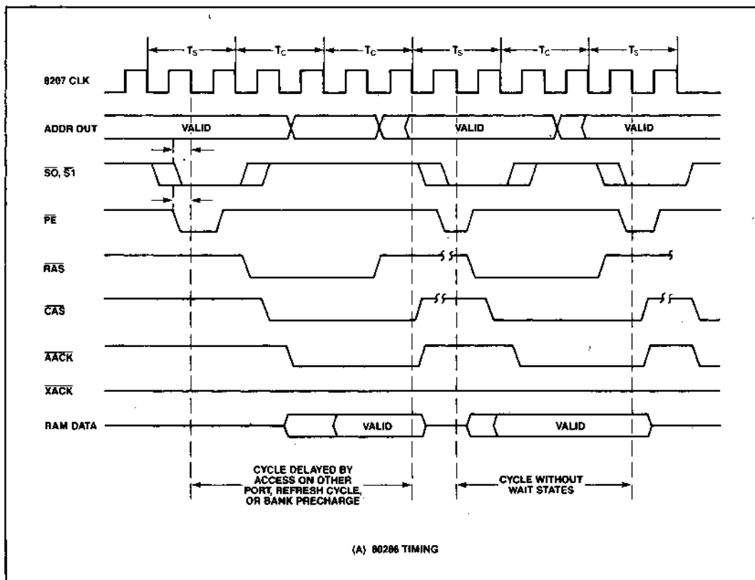
Figure 14. 80286 Synchronize Timing
