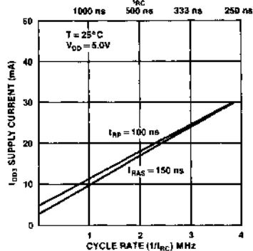
GRAPH 12 TYPICAL RAS-ONLY REFRESH CURRENT I_{DD3} vs. 1/t_{RC}
