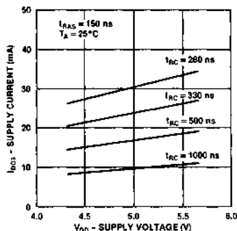
GRAPH 10 TYPICAL RAS-ONLY REFRESH CURRENT I_{DD3} vs. V_{DD}
