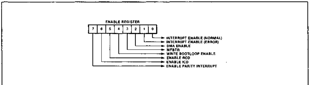
Figure 8. Enable Register
