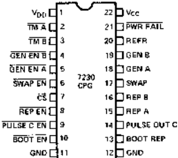
Figure 2. Pin Configuration
