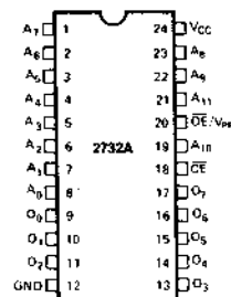
Figure 2. Pin Configuration
