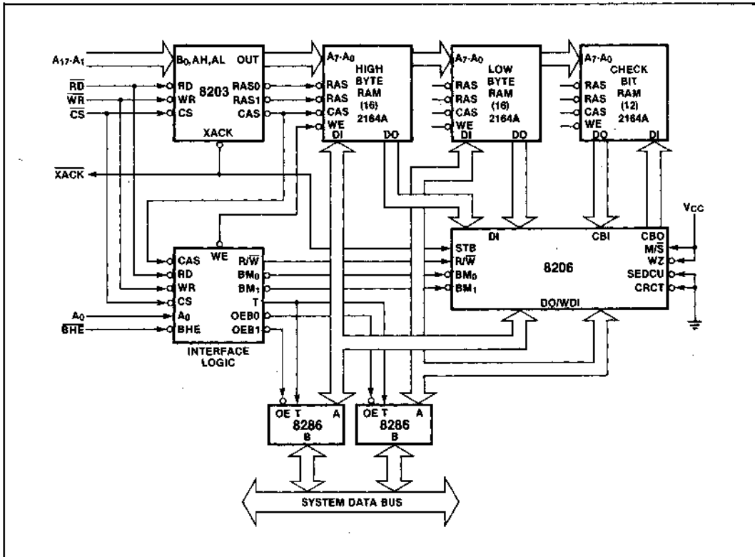
Figure 1. 8203/8206 Memory System
