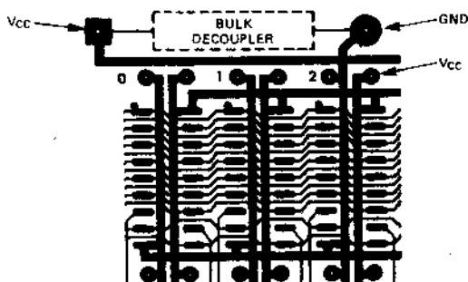
FIGURE 4. PC LAYOUT.
