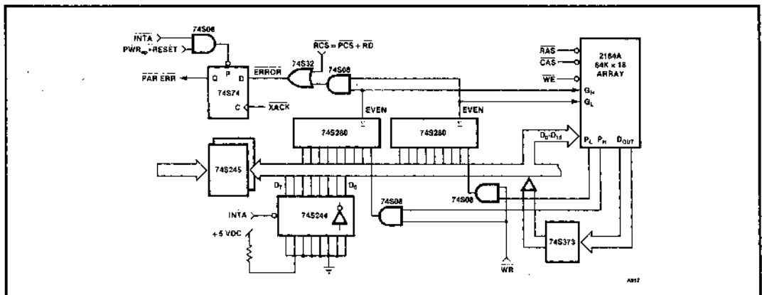
Figure 23. Parity Checker/Generator
