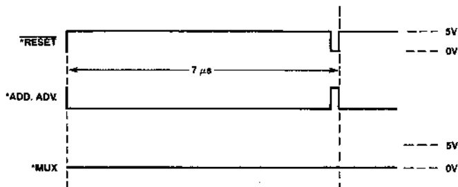
2115/2125 TIMING DIAGRAM 7 \mu S CYCLE TIME
