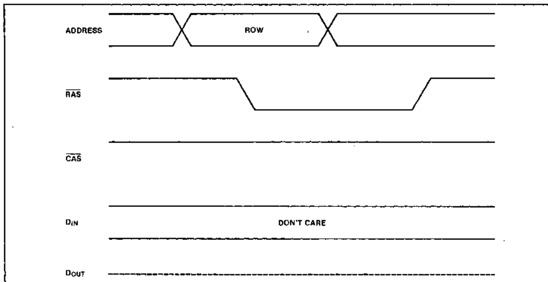
Figure 8. RAS-only Refresh
