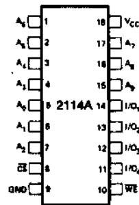
PIN CONFIGURATION
