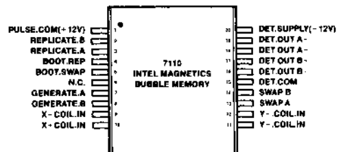
Figure 2. Pin Configuration
