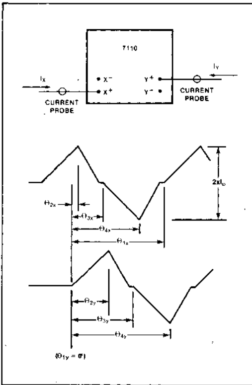
Figure 6. X-Y Coil Waveforms
