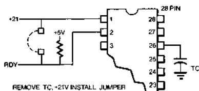
FIGURE 7. 2817 TO 2817A UPGRADE DESIGN
