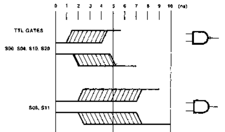
Figure 24B. Skew
