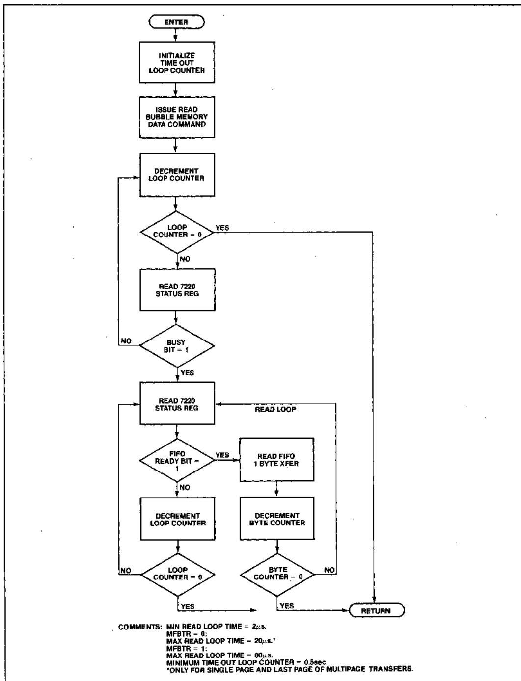
Figure 15. READ
