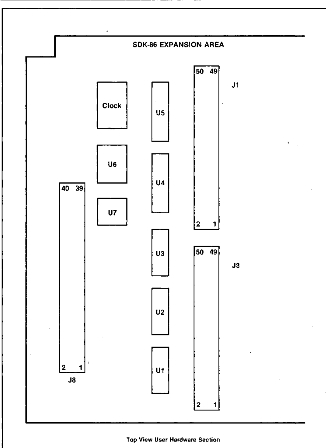
Figure 10. Parts Layout
