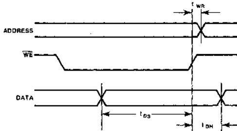
Figure 39. WE Constraints
