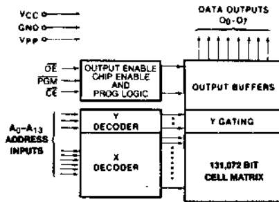
Figure 1. Block Diagram MODE SELECTION
