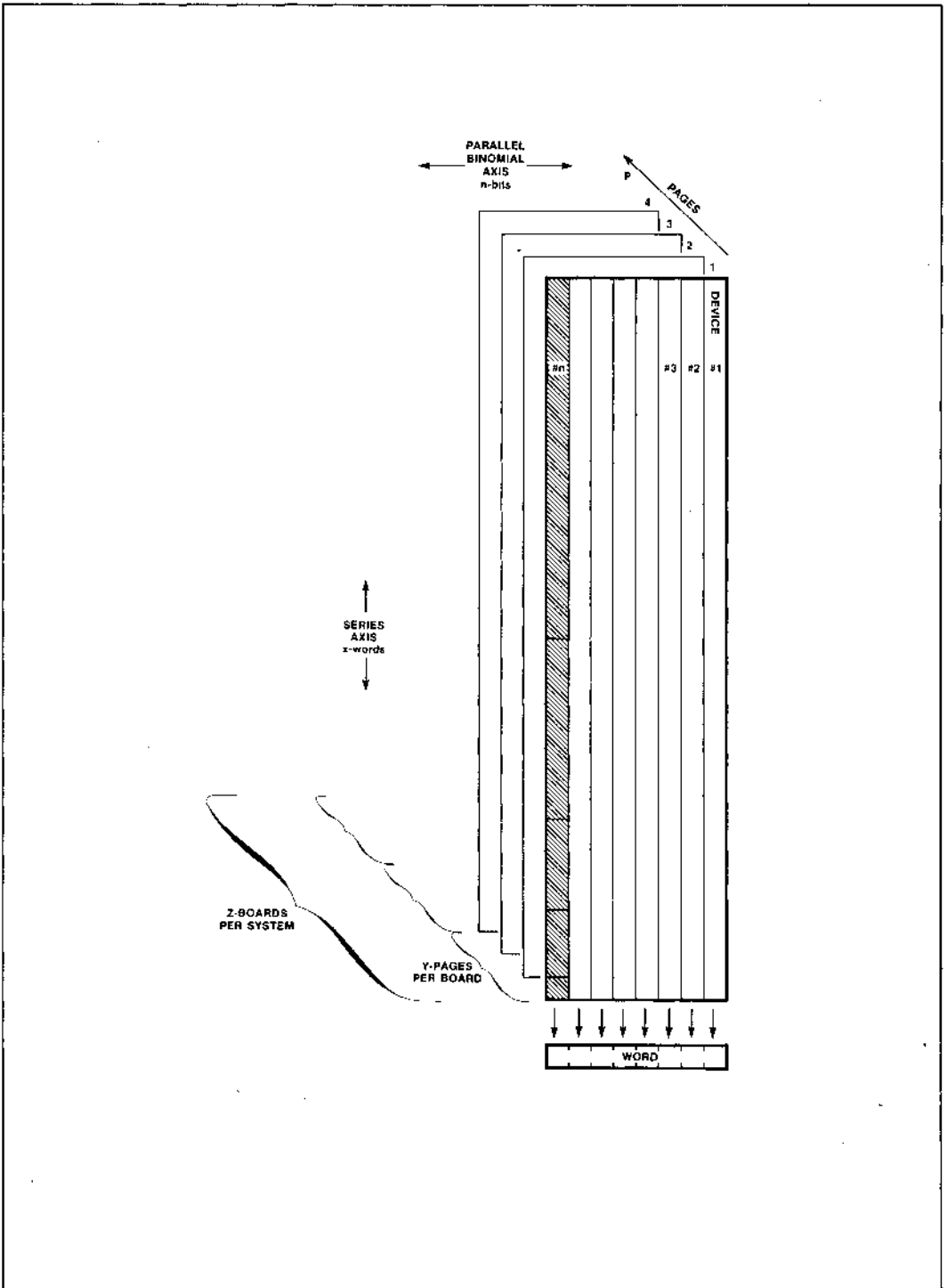
Figure 1. Memory Configuration
