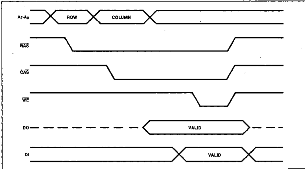
Figure 3. Single-Cycle Read-Modify-Write
