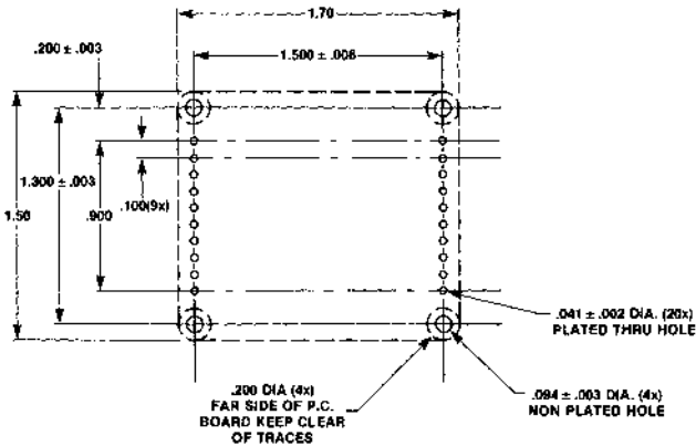
P.C. BOARD SPACE REQUIREMENTS
