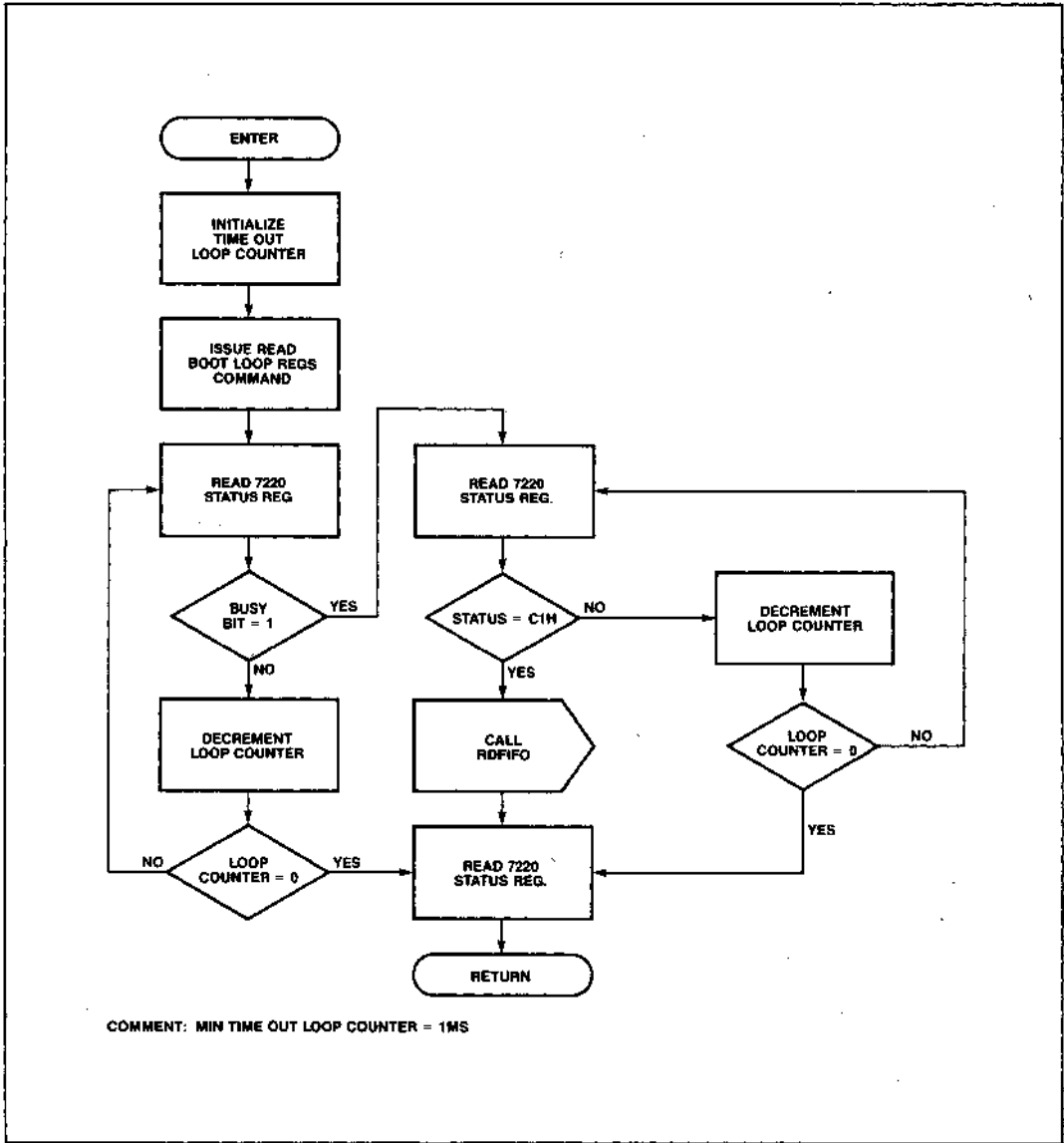
Figure 25. RDBLRS
