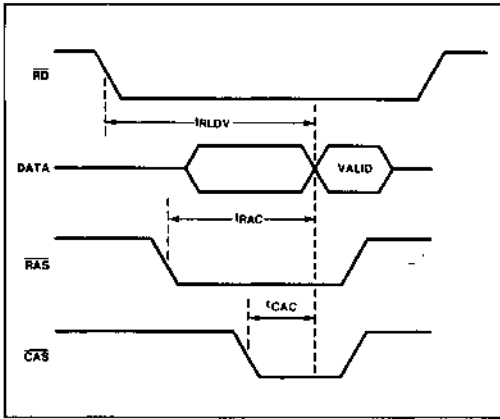
Figure 9. Read Access Time
