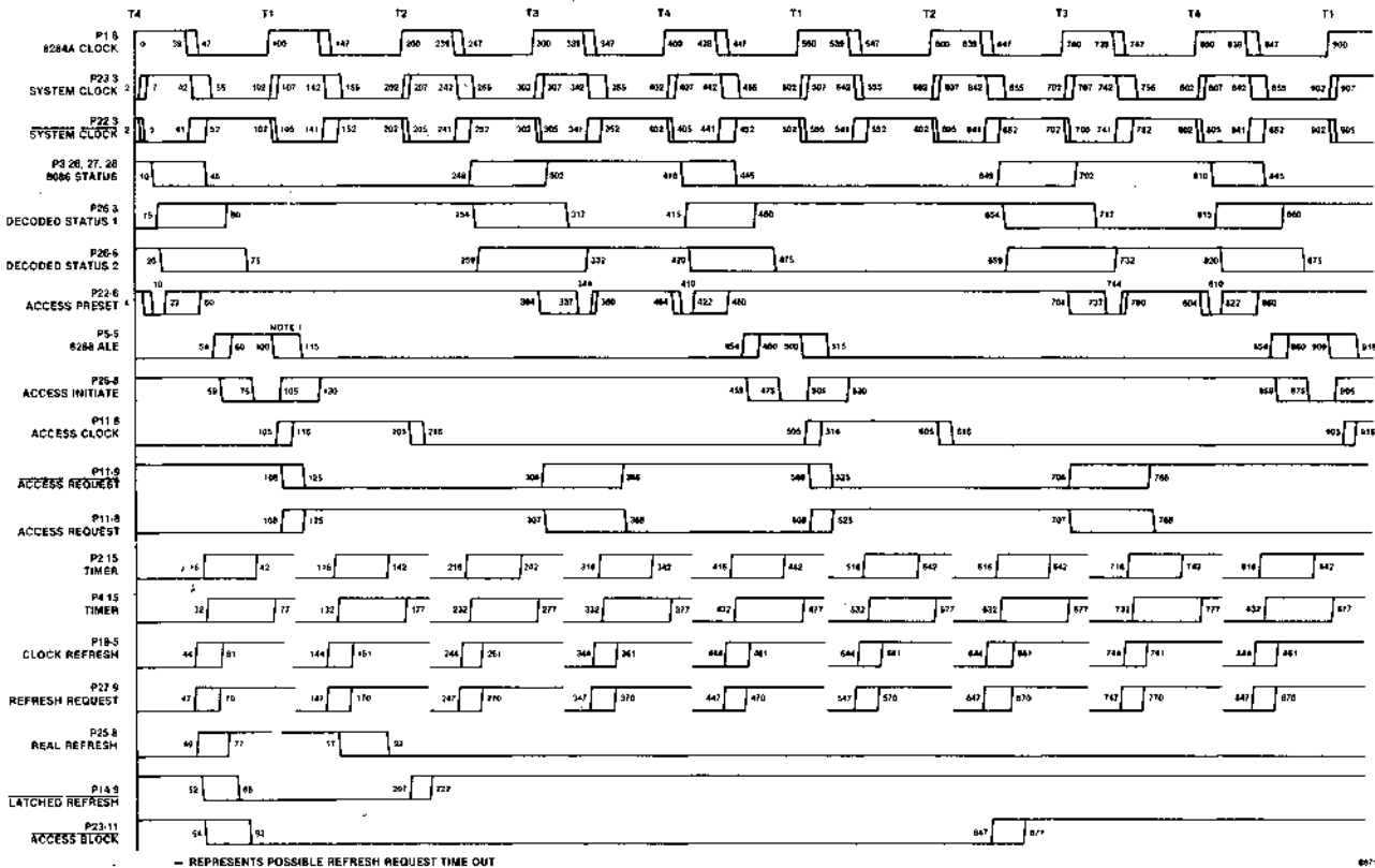
Figure 28. Refresh Cycle Followed by a Read/Write Cycle
