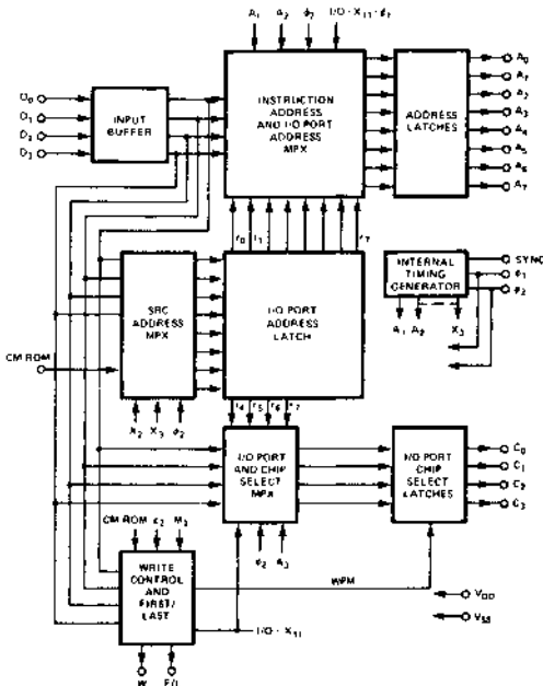
4008 BLOCK DIAGRAM
