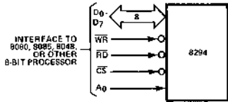
Figure 1. Polling Interface
