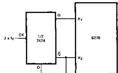
EXTERNAL CLOCK
