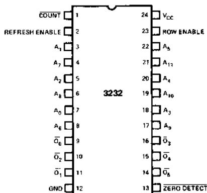
PIN CONFIGURATION
