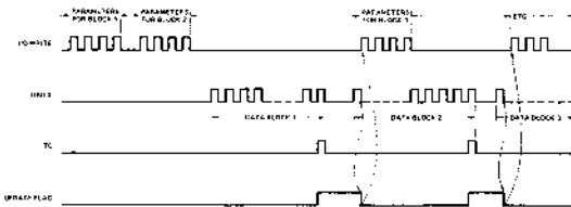
Figure 5. Autoload Timing
