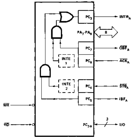
Figure 12. MODE 2
