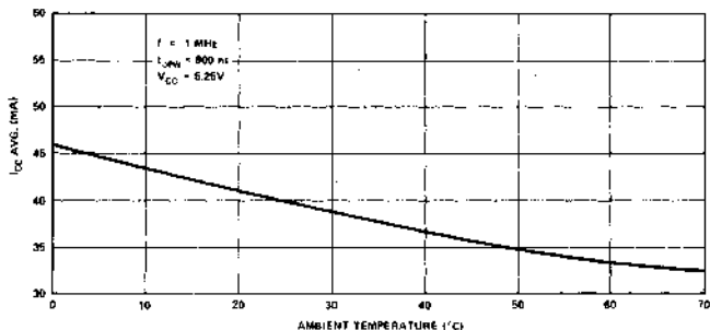
POWER SUPPLY CURRENT ( I_{CC} ) VS. AMBIENT TEMPERATURE ( ^{\circ}C )
