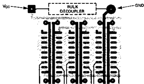
FIGURE 4. PC LAYOUT.
