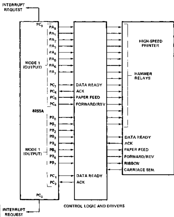
Figure 17. Printer Interface
