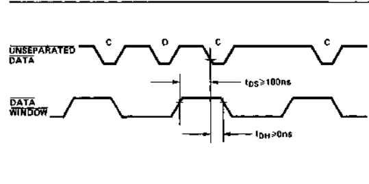
Figure 21. Data Separator
