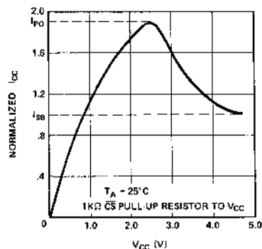
GRAPH 1 TYPICAL POWER-ON CURRENT VS. POWER SUPPLY VOLTAGE
