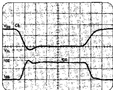
FIGURE 1. i_{CC} WAVEFORM.
