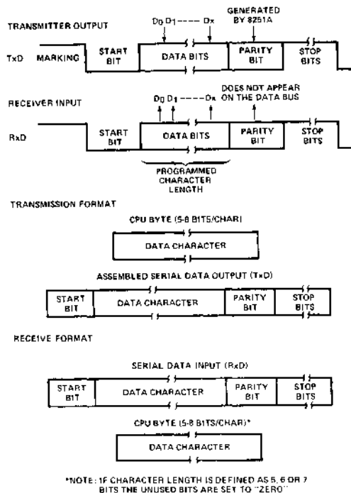
Figure 7. Asynchronous Mode
