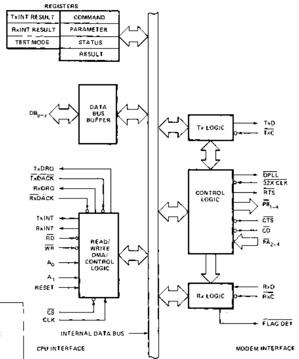
BLOCK DIAGRAM
