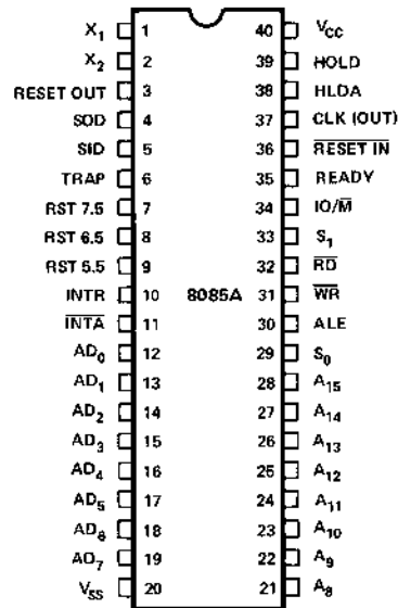
Figure 1. Pin Configuration
