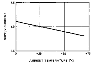
Figure 2. Typical Supply Current vs. Temperature, Normalized [1]
