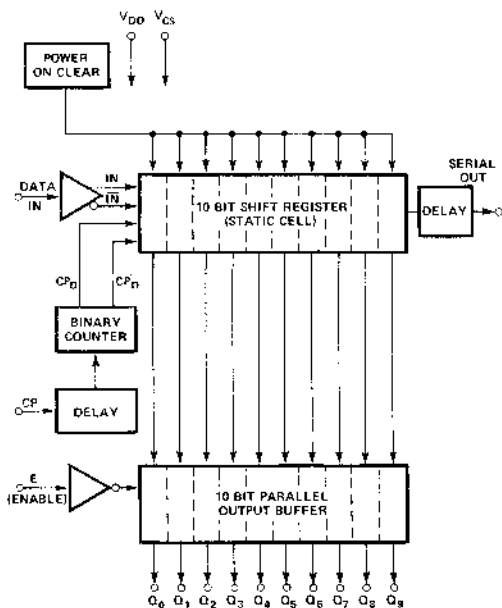
BLOCK DIAGRAM
