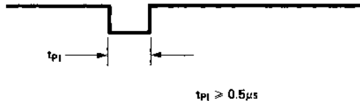
Figure 15. Index Timing
