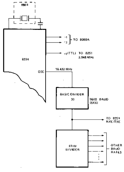
Figure 1. Block Diagram
