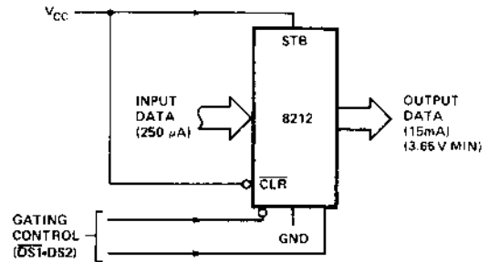
Figure 3. Gated Buffer (3-State)
