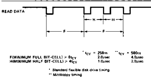
Figure 19. Read Data
