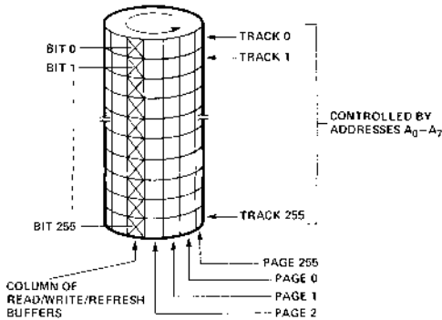
FIGURE 1. ORGANIZATION
