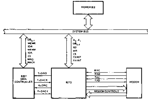
Figure 14. 8273 System Diagram
