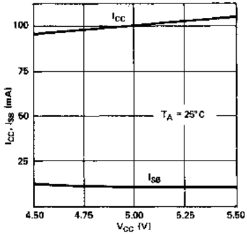
GRAPH 1 SUPPLY CURRENT [1] VS. SUPPLY VOLTAGE
