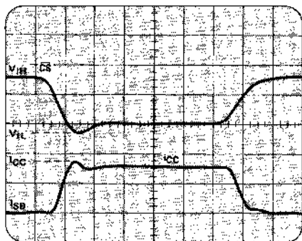
FIGURE 1. I_{CC} WAVEFORM.
