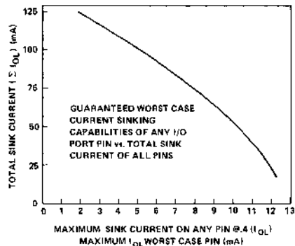
Figure 1. Sink Capability
