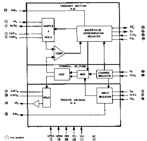
BLOCK DIAGRAM
