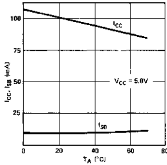
GRAPH 2 SUPPLY CURRENT [1] VS. AMBIENT TEMPERATURE
