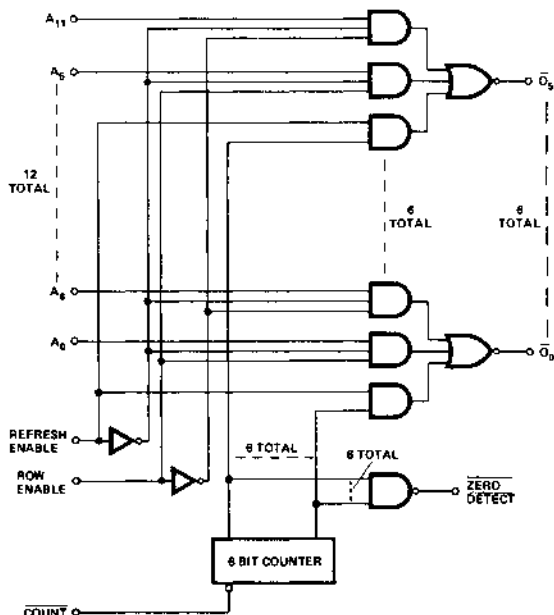
LOGIC DIAGRAM
