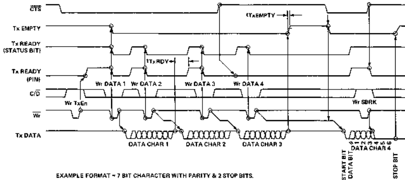
EXAMPLE FORMAT - 7 BIT CHARACTER WITH PARITY & 2 STOP BITS.
