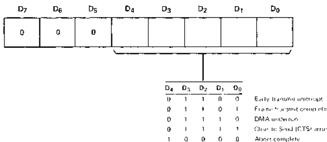
Figure 9. Tx Interrupt Result Byte Format
