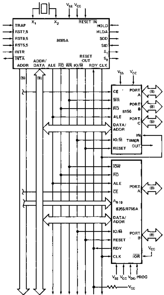
Figure 4. 8085A Minimum System (Standard I/O Technique)
