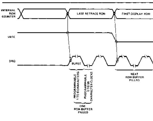
Figure 18. DMA Timing
