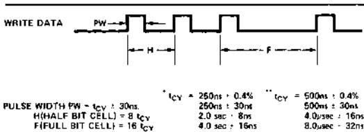
Figure 18. Write Data
