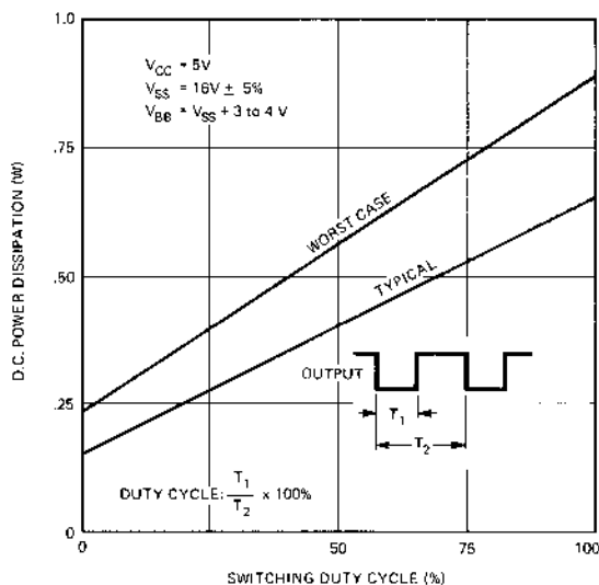
NO LOAD D.C. POWER DISSIPATION VS. OPERATING DUTY CYCLE
