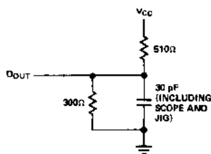
Figure 1. Output Load
