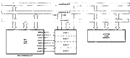
Figure 10. Floppy Disk Controller (4 Drives)
