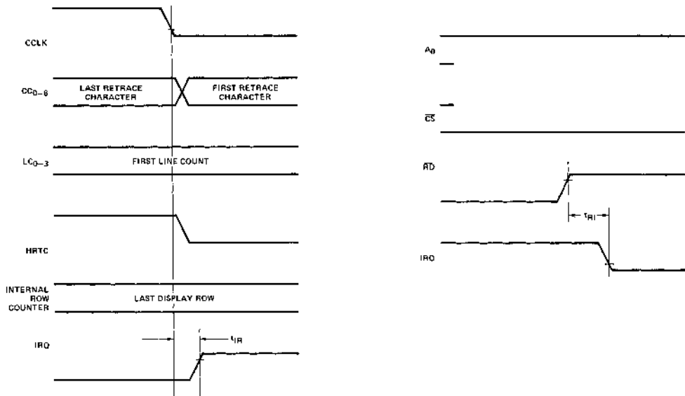
Figure 29. Interrupt Timing
