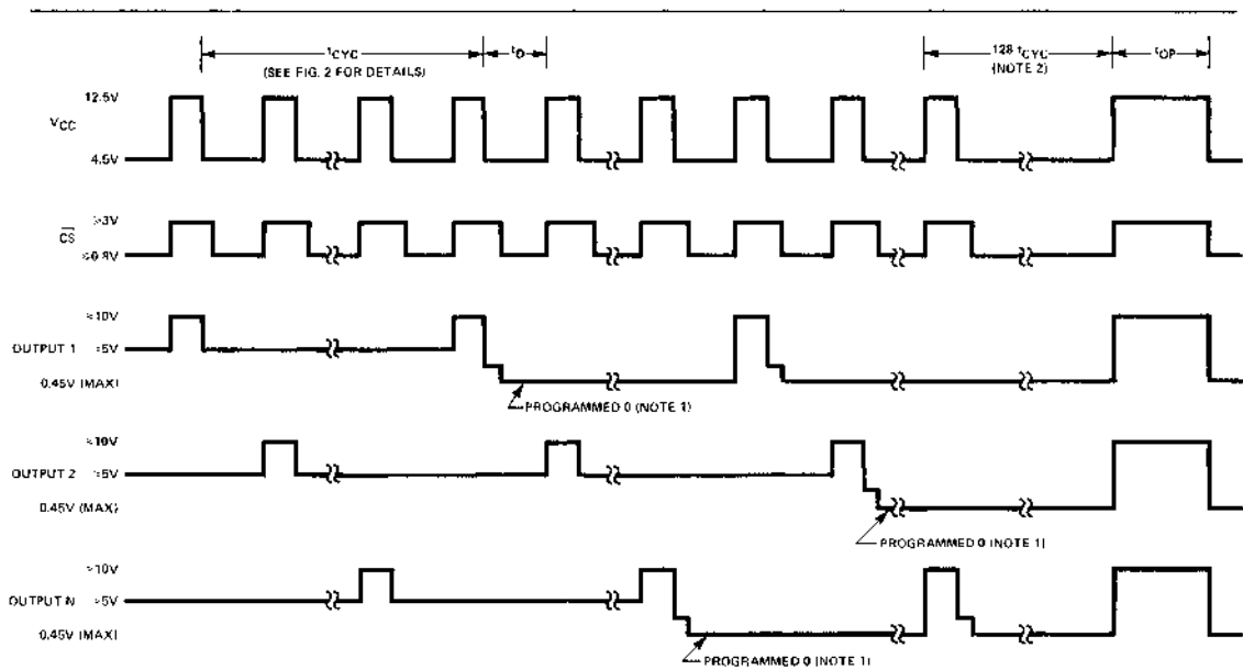
Figure 1. Programming Cycles.
