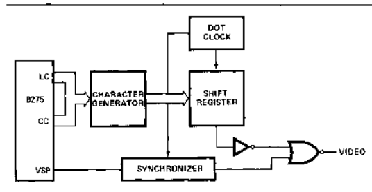
Figure 14. Typical Dot Level Block Diagram
