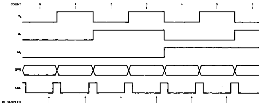
Figure 3. Keyboard Timing
