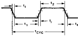
Figure 10. Clock Timing Waveform
