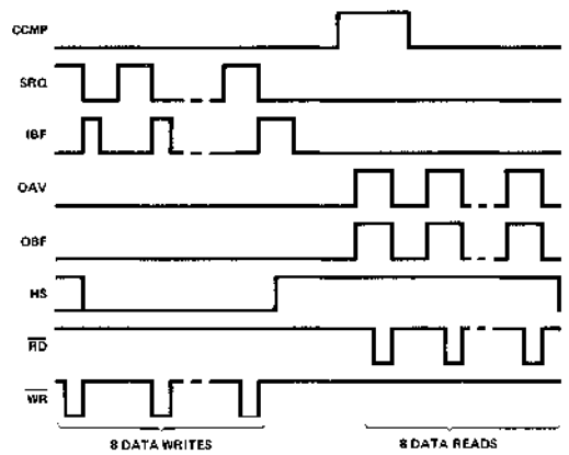
Figure 7. Encode/Decode data
