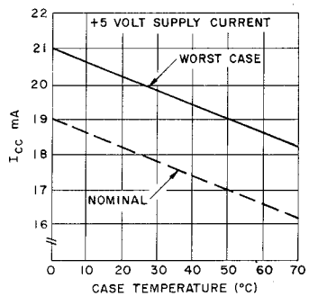
Fig.26 +5 VOLT SUPPLY CURRENT
