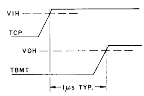
Fig.20 TBMT TURN-ON
