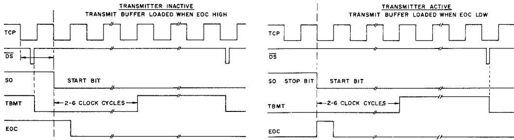
Fig.6 TRANSMITTER AT START BIT
