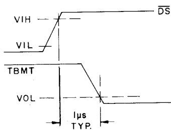
Fig.40 TBMT TURN-OFF
