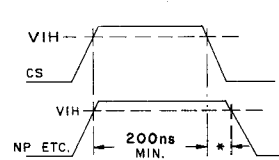
Fig.35 XR PULSE
