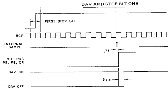
Fig.12 RECEIVER DURING 1st STOP BIT
