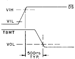
Fig.18 TBMT TURN-OFF
