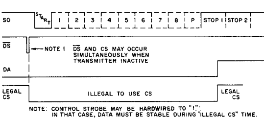
Fig.8 ALLOWABLE POINTS TO USE CONTROL STROBE
