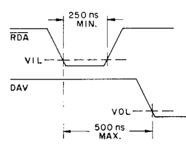
Fig.22 RDAV
