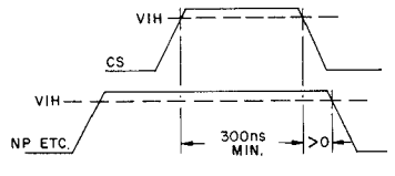
Fig.15c CS
