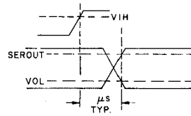
Fig.38 SEROUT
