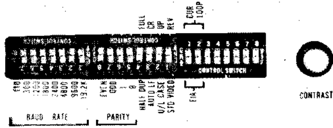
Figure 3-1. Legend Plate (Under Access Panel)
