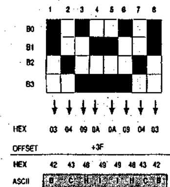
Figure 2-6: Bottom Sixel
