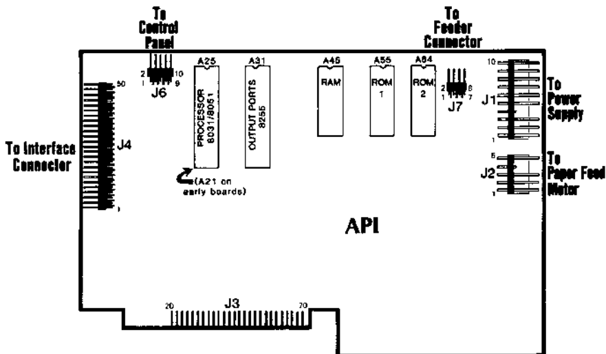
Figure 2-1. API CIRCUIT BOARD LAYOUT
