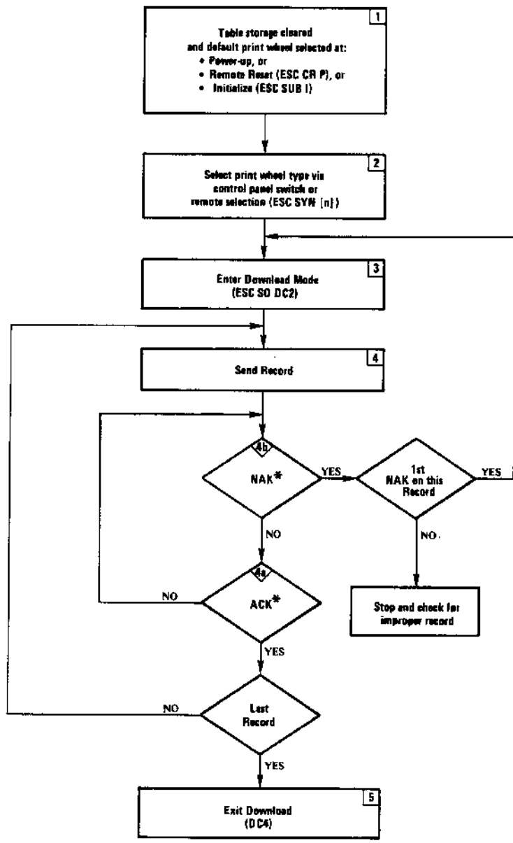
Figure 3-7. DOWNLOAD FLOW CHART
