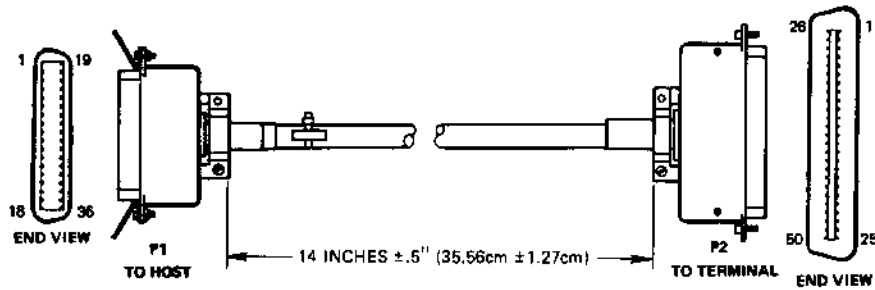
Figure 2-8. CENTRONICS 703 INTERFACE CABLE DIABLO Part No. 320839-01
