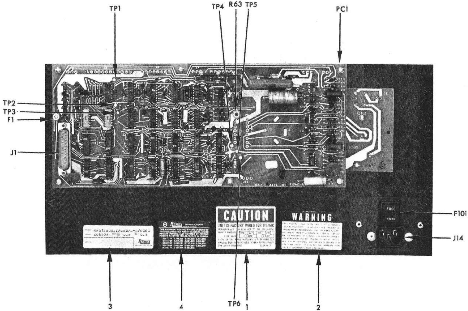
Figure 7-5. RRS7200 Rear View.
