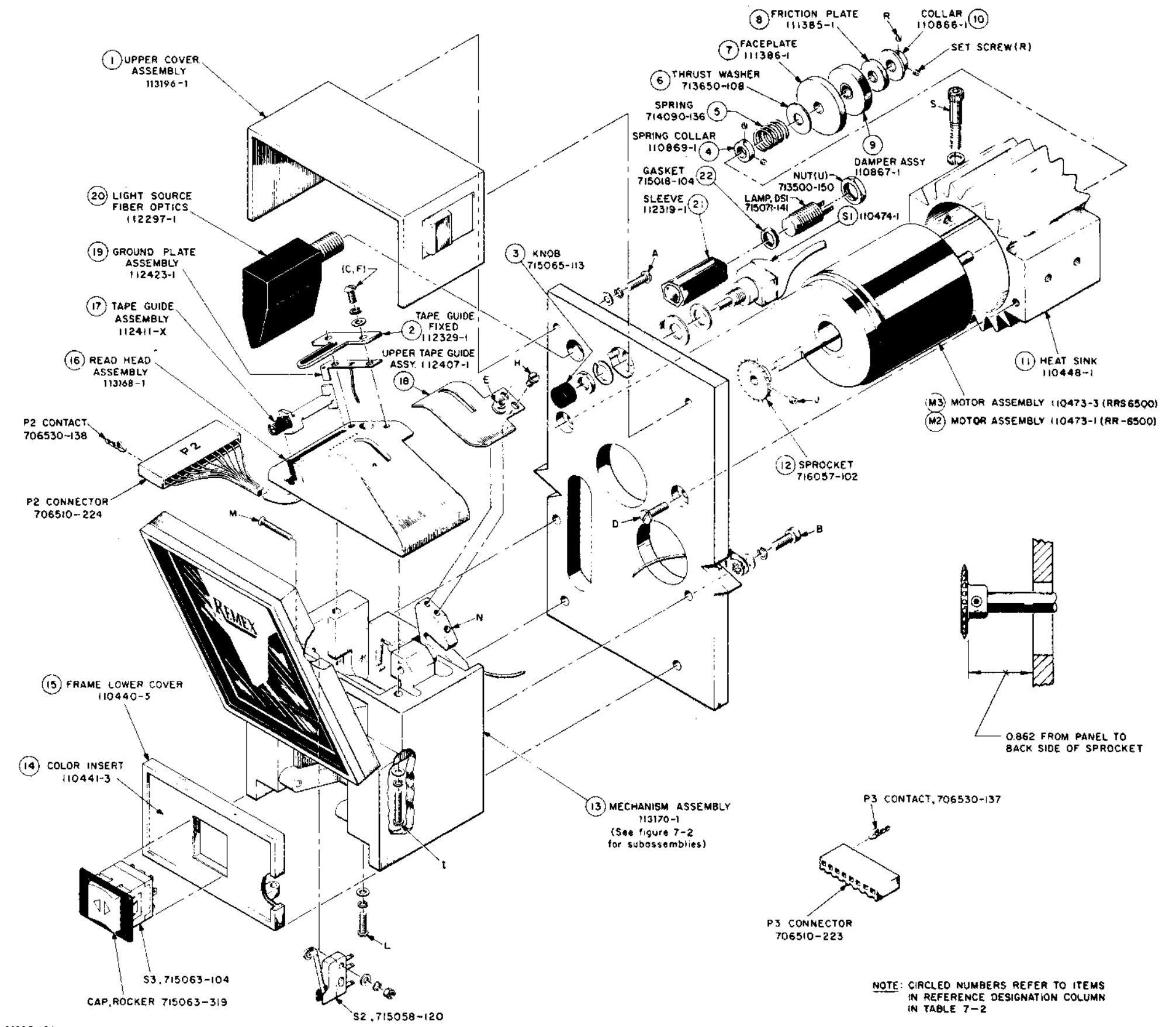
Figure 7-1. Exploded View of Readhead Mechanism Assembly
