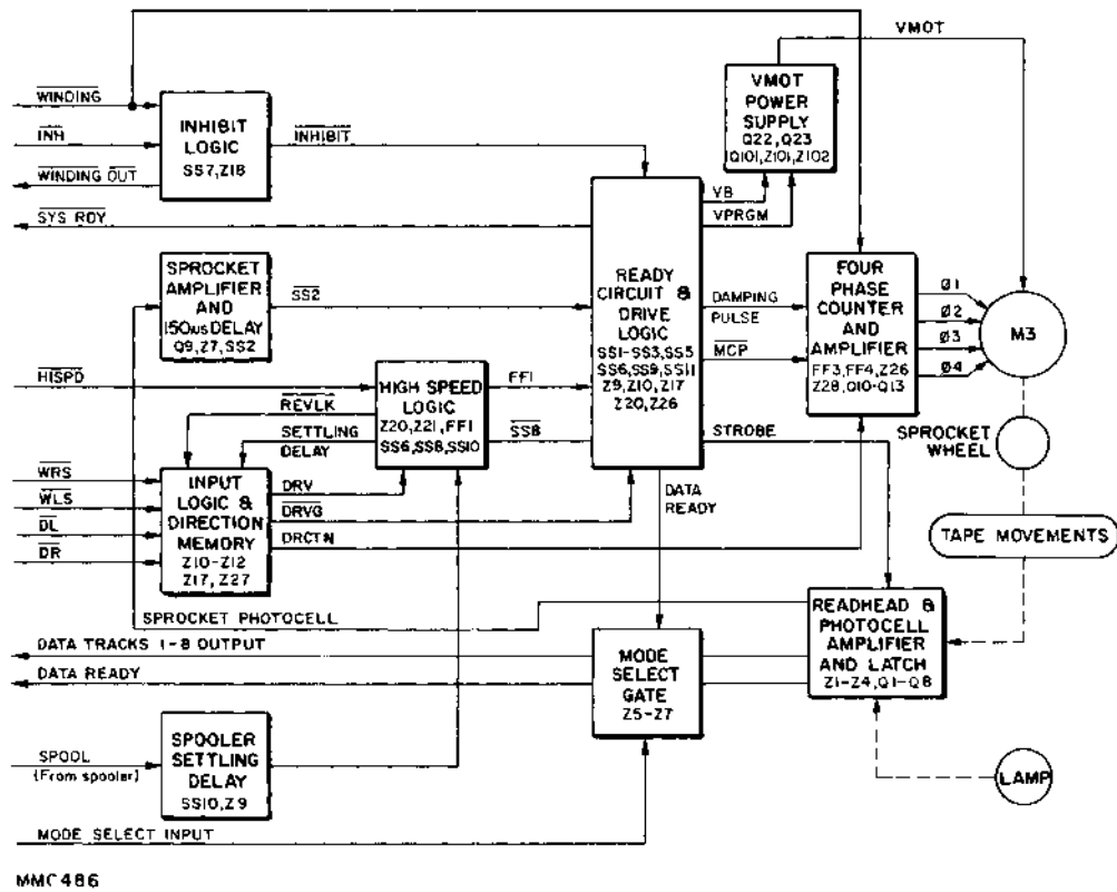
Figure 4-1. Block Diagram, Reader Circuitry. Component Designations listed are for RRS6500.
