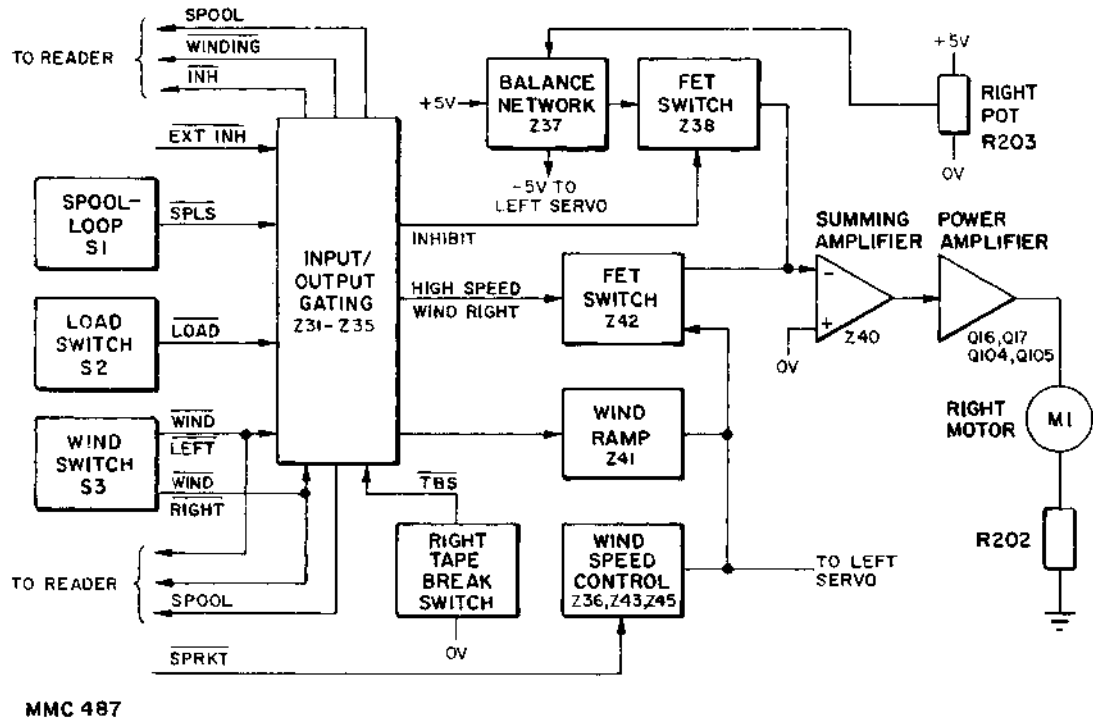
Figure 4-2. Block Diagram, Spooler Circuitry, RRS6500 Only.
