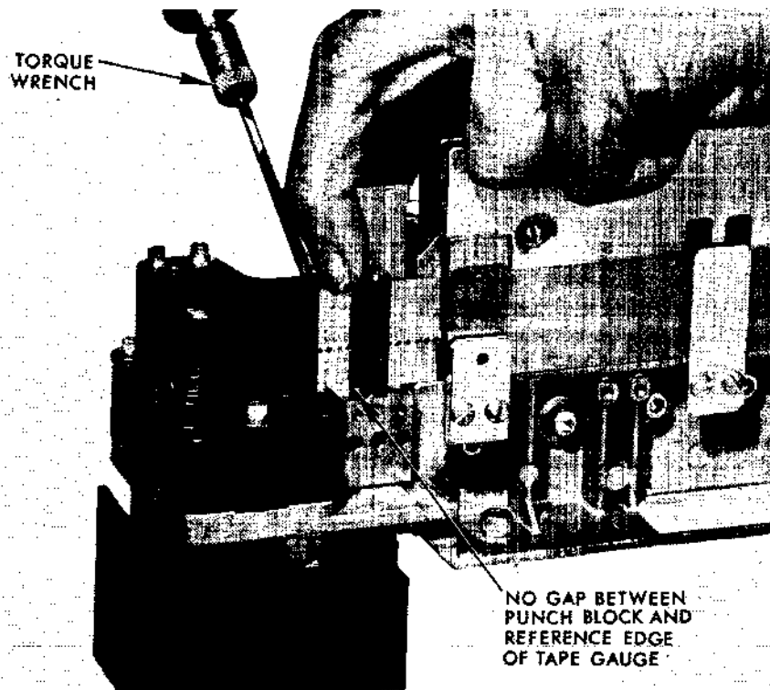
Figure 6-4. Installation of Punch and Pin Block Assembly.
