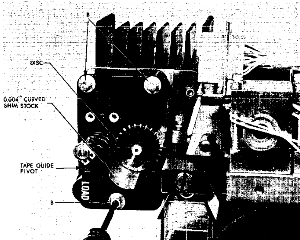
Figure 5-4. Tape Drive Assembly Alignment.
