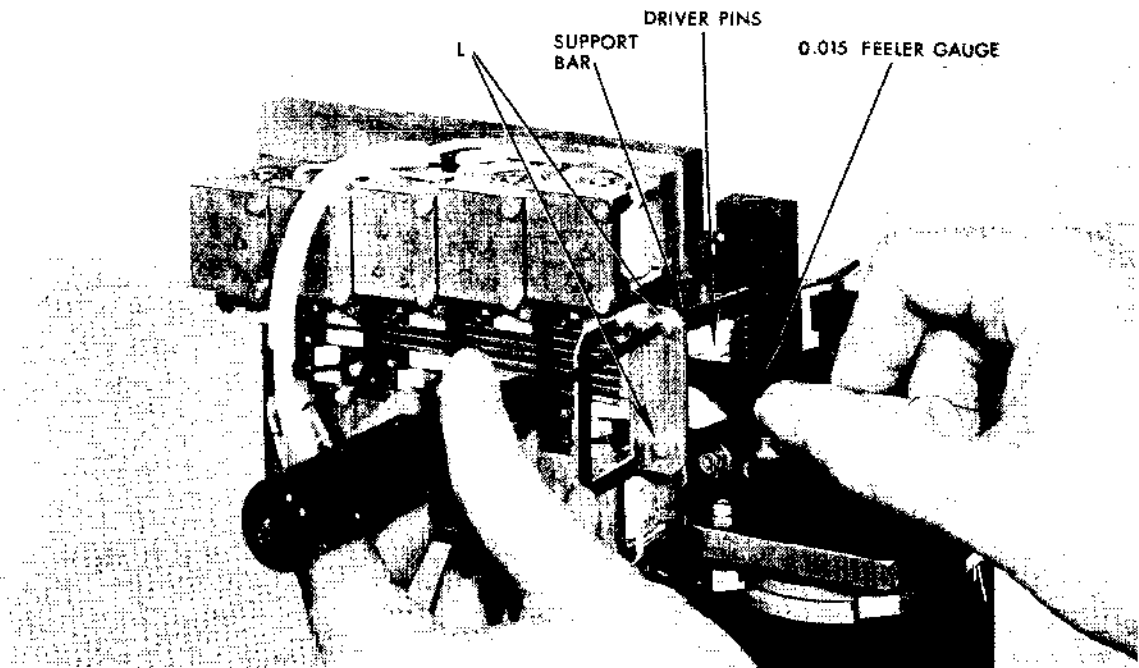
Figure 6-5. Adjustment of Support Bar and Support Bracket.
