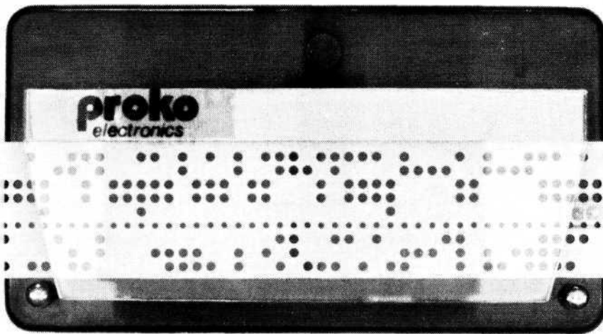
Low-cost Paper Tape Reader from PROKO (assembled).
