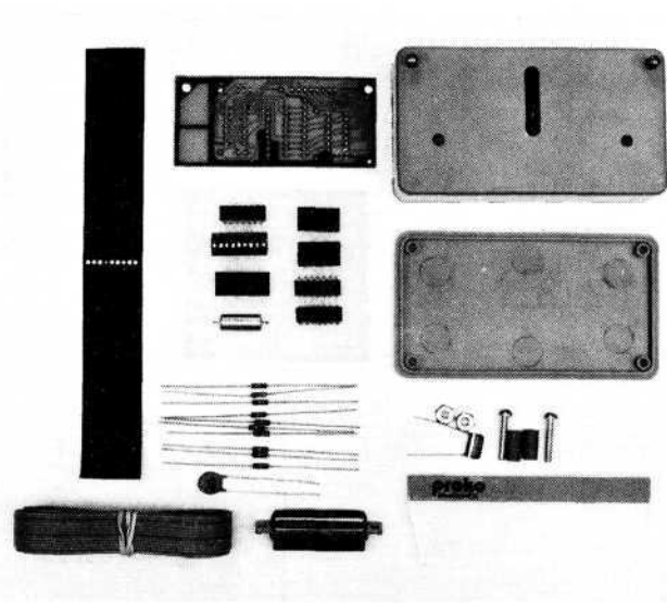
Low-cost Paper Tape Reader from PROKO (kit).
