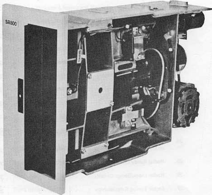
Figure 1. SA800/801 Diskette Storage Drive
