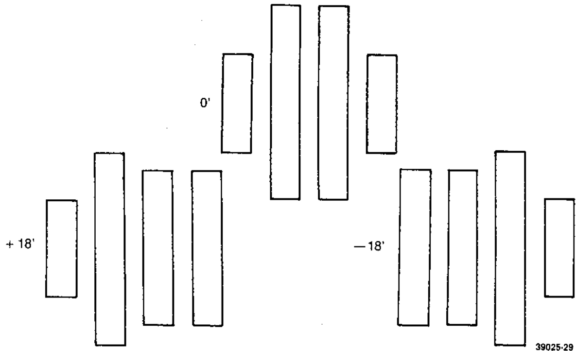
FIGURE 5-13. AZIMUTH BURST PATTERNS
