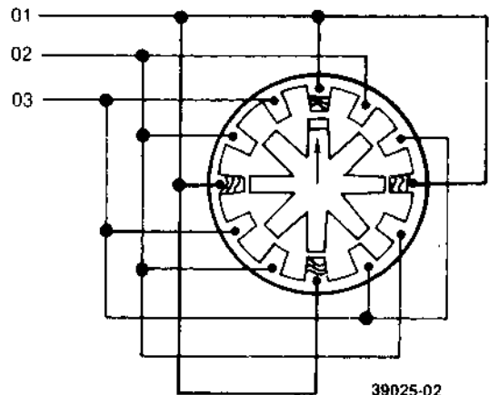
FIGURE 4-2. POSITION 1 (TRK 00)
