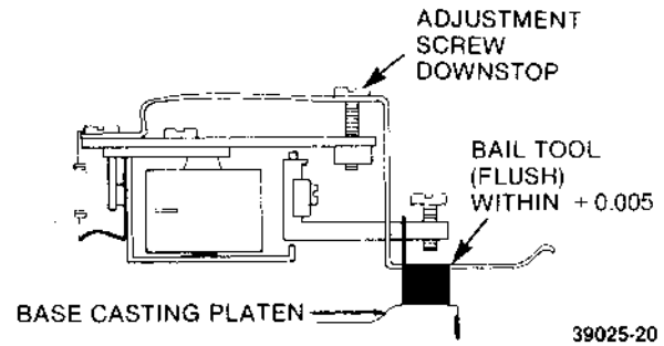
FIGURE 5-4. HEAD LOAD ACTUATOR DOWNSTOP ADJUSTMENT
