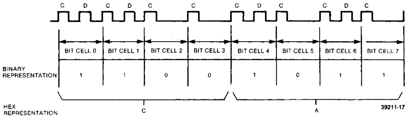
FIGURE 4-11. BIT CELL
