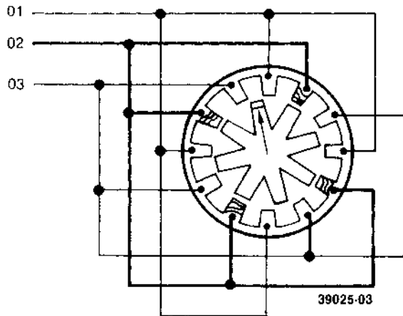
FIGURE 4-3. POSITION 2 (TRK 01)
