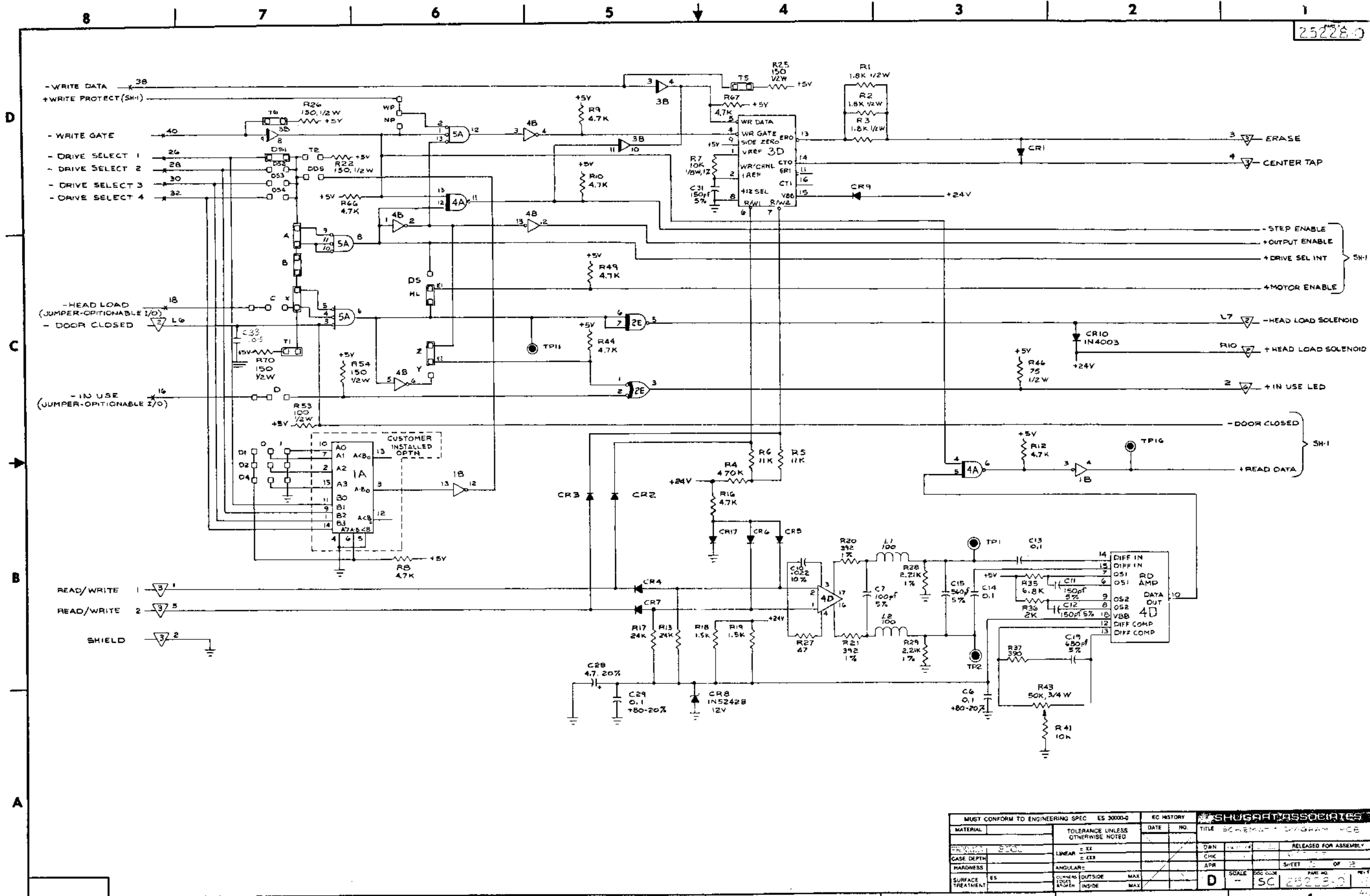
FIGURE 6-4. SCHEMATIC DIAGRAM, P/N 25229 (SHEET 2 OF 2)
