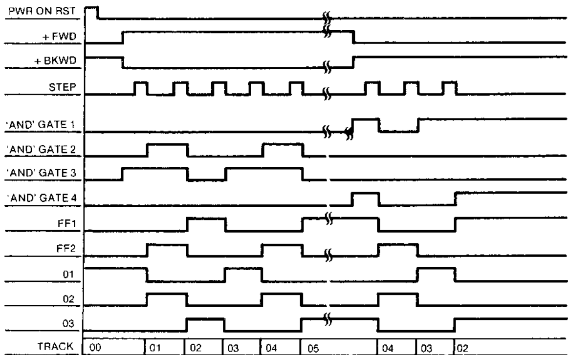
FIGURE 4-6. TRACK ACCESSING
