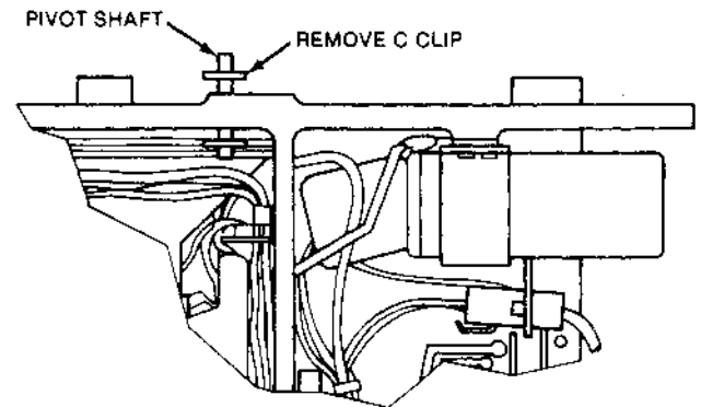
FIGURE 5-8. CARTRIDGE GUIDE REMOVAL
