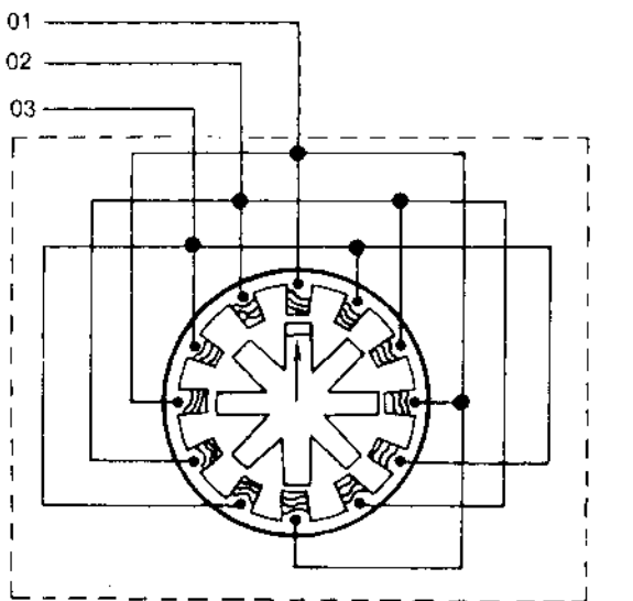
FIGURE 4-1. STEPPER MOTOR
