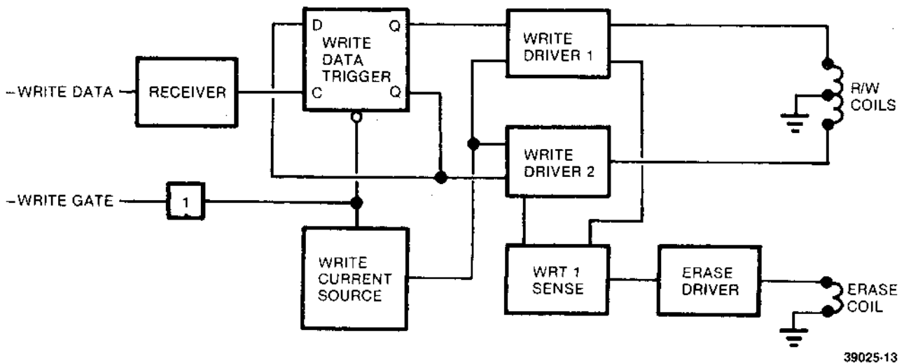
FIGURE 4-17. WRITE CIRCUIT FUNCTIONAL DIAGRAM
