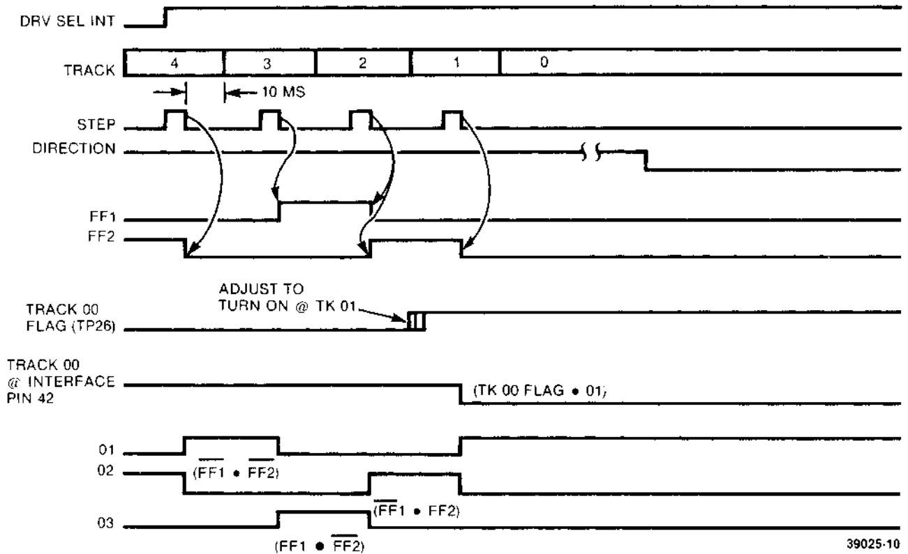
FIGURE 4-10. TRACK 00 TIMING
