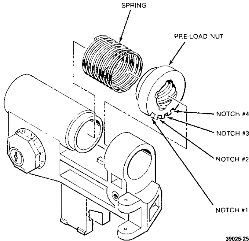
FIGURE 5-9. CARRIAGE ASSEMBLY
