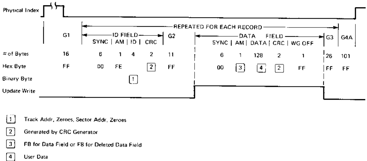
FIGURE 1. FM RECOMMENDED FORMAT – 128 Byte & 16 Records/Track (IBM Type)
