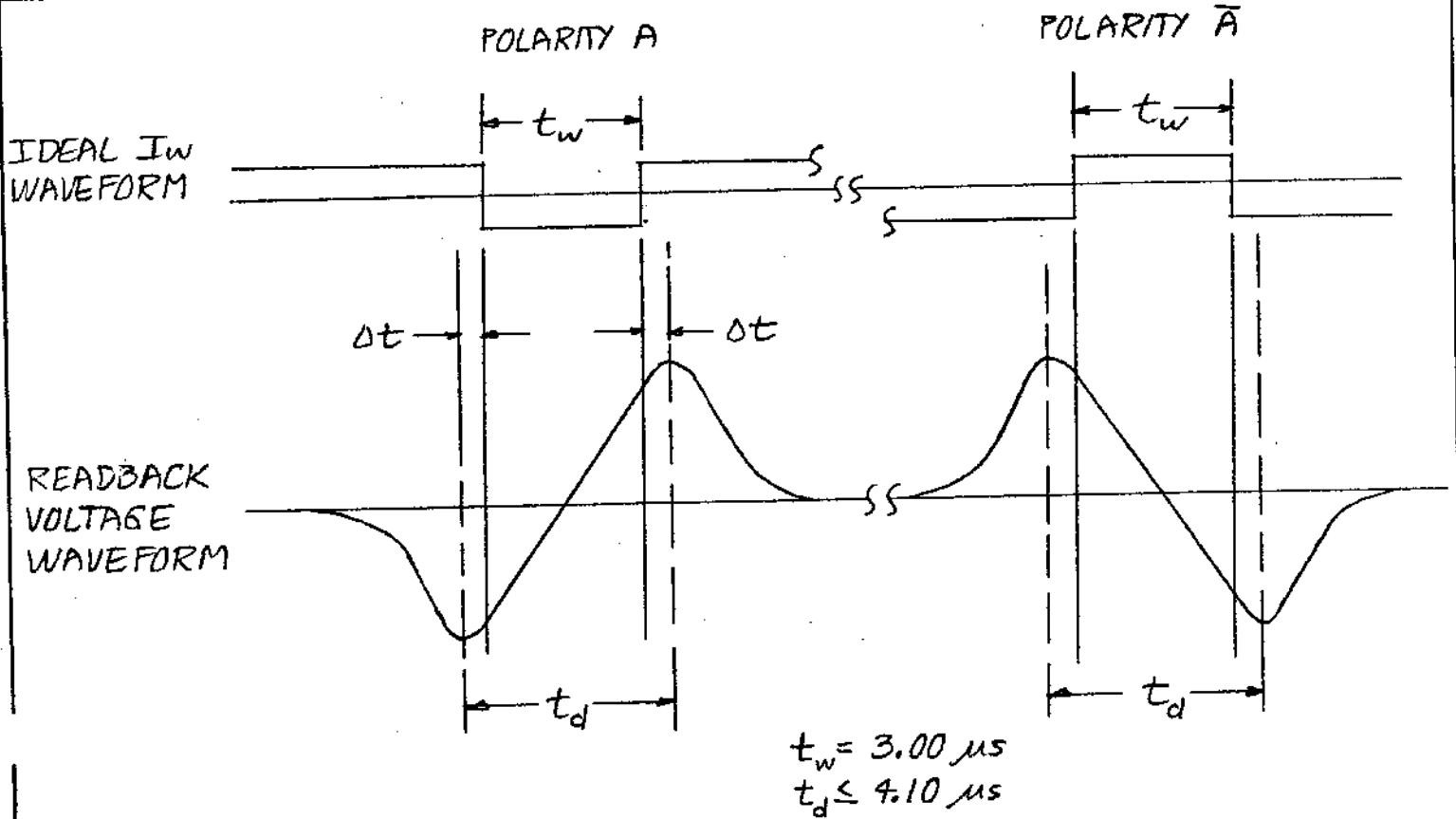
Figure 7: Dipulse Test
