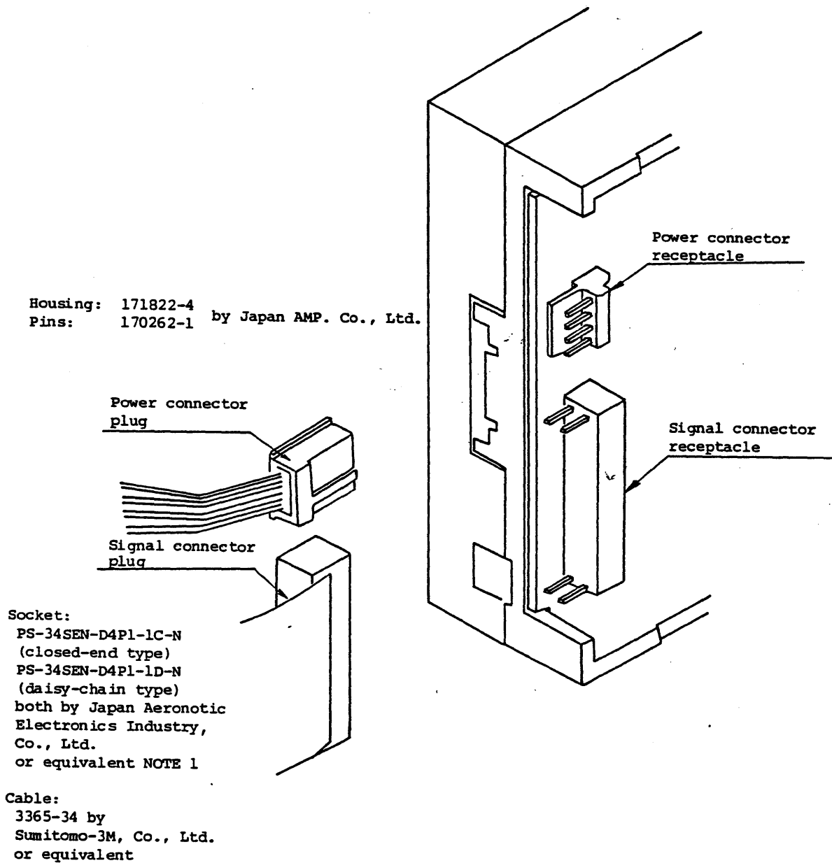
Fig. 3.4 Connector Locations and Recommended Models
