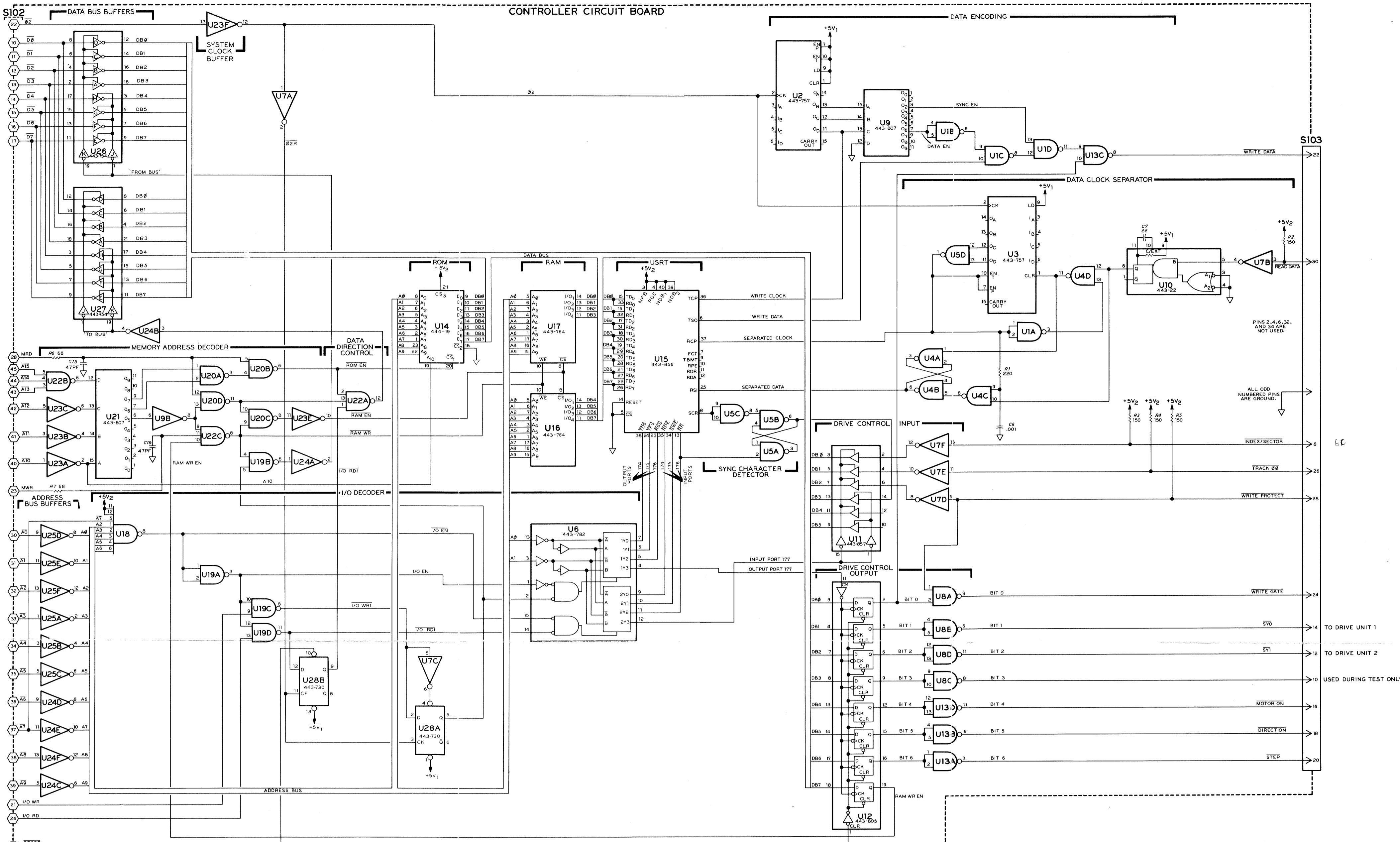
SCHEMATIC OF THE HEATH MODEL WH17 FLOPPY DISK
