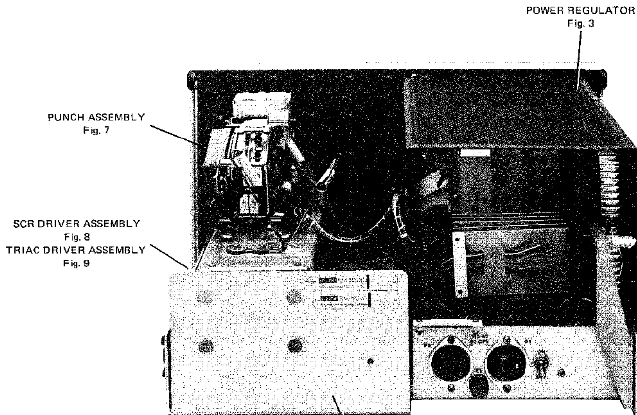
READER ASSEMBLY Fig. 4
