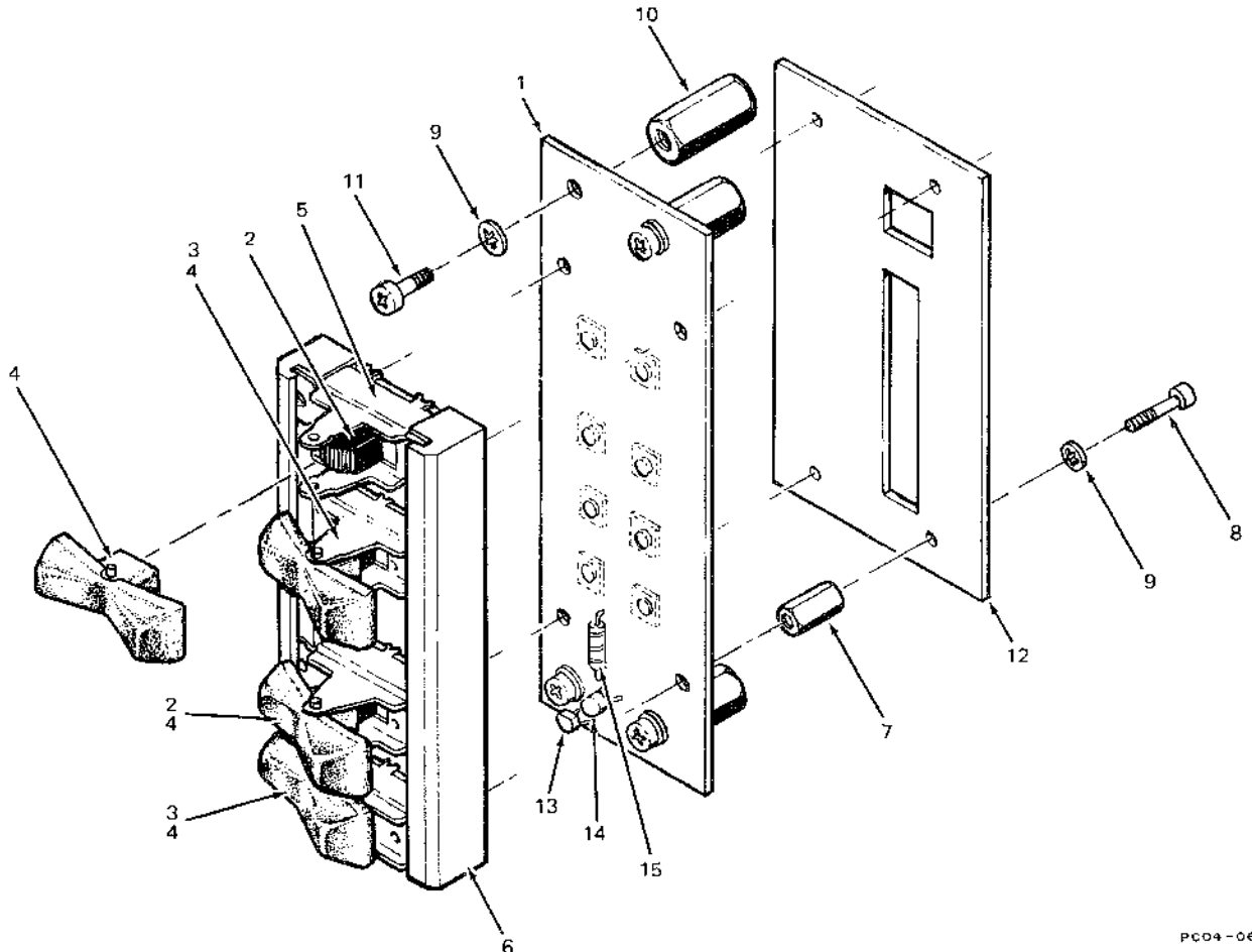
Figure 5. Switch Assembly
