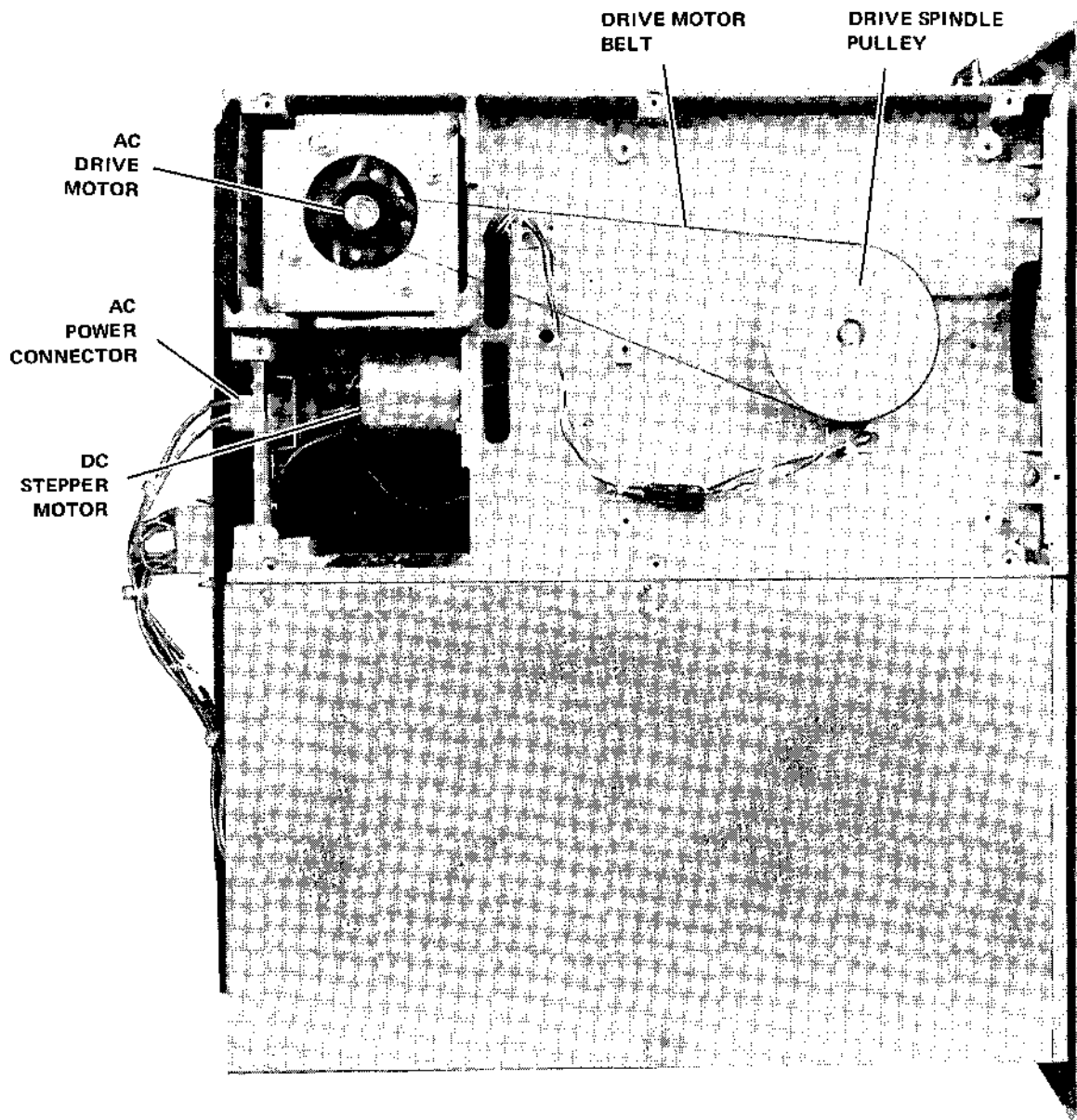
Figure 1-6 Underside View of Drive
