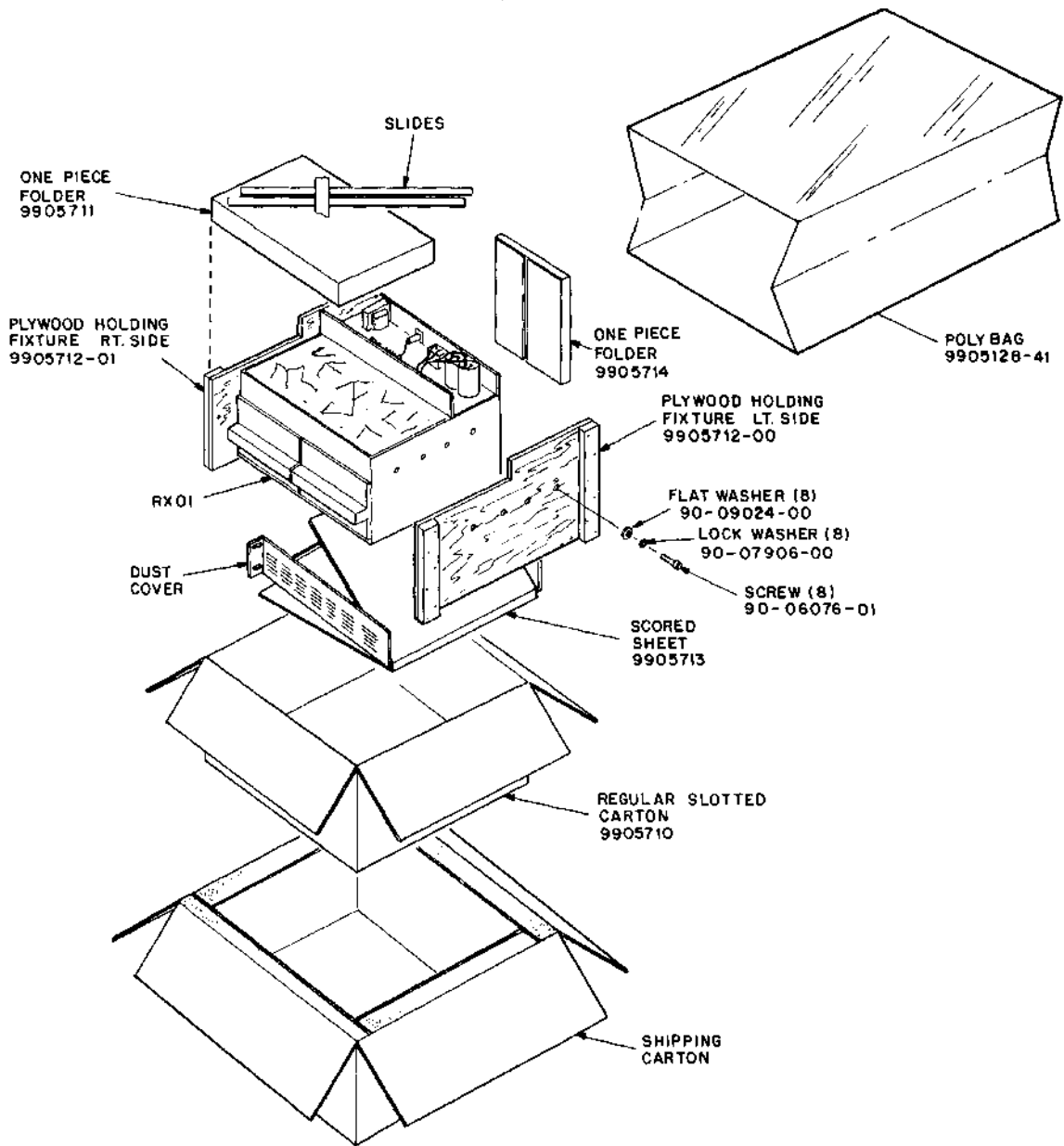
Figure 2-4 RX8/RX11 Unpacking
