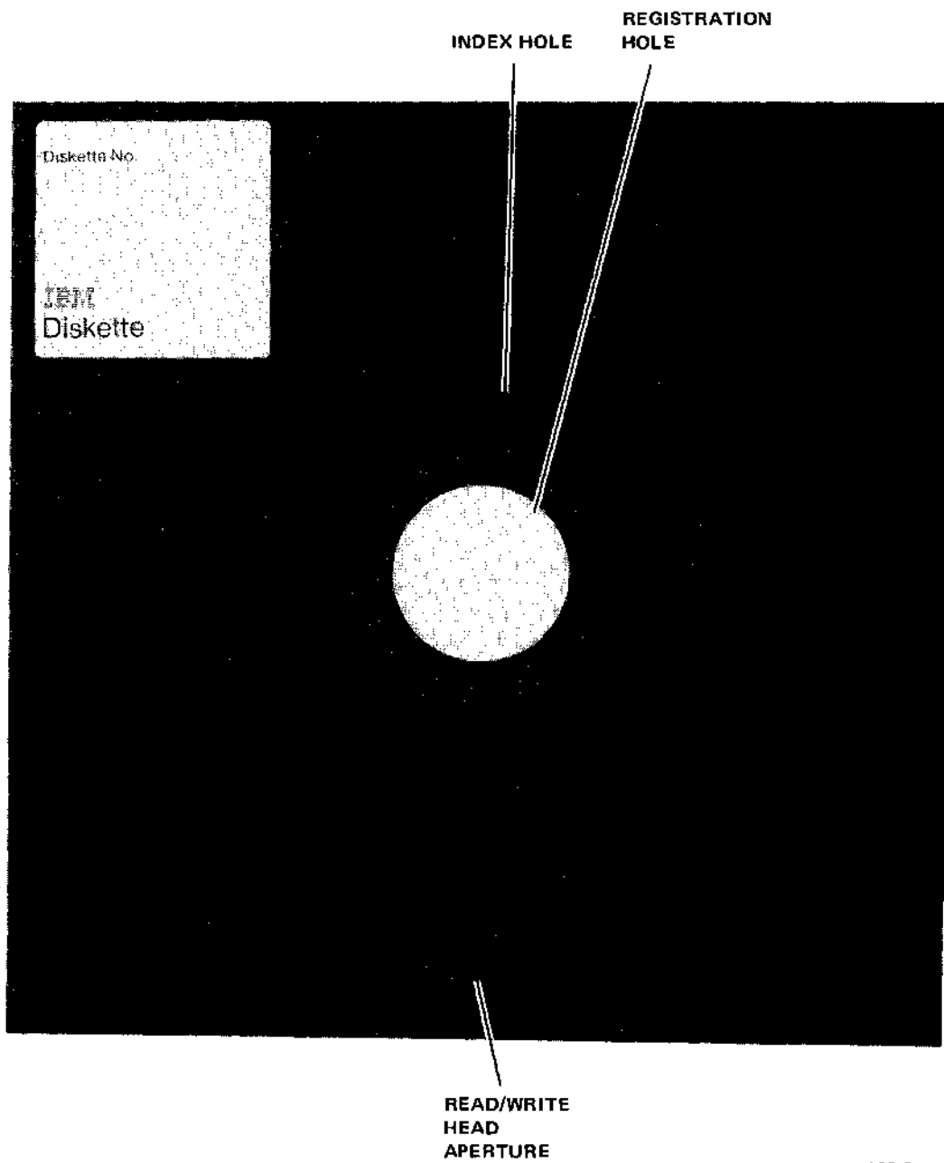
Figure 1-8 Diskette Media
