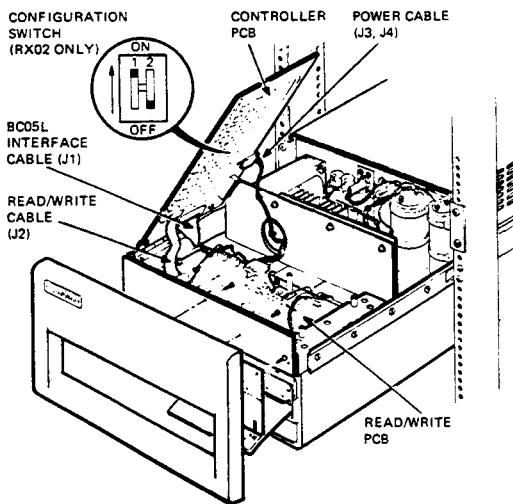
Figure 2-3 Controller Board Connections
