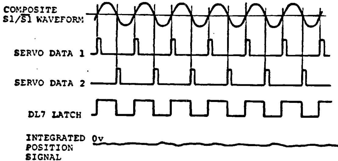
Figure 3 Integration of S1/\overline{S1} Composite
